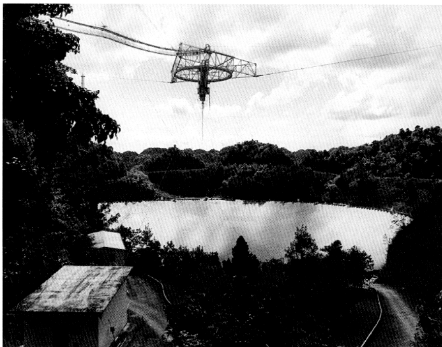
Fig. 3 The Arecibo telescope. This photo was taken on October 12, 1992 by Seth Shostak.
