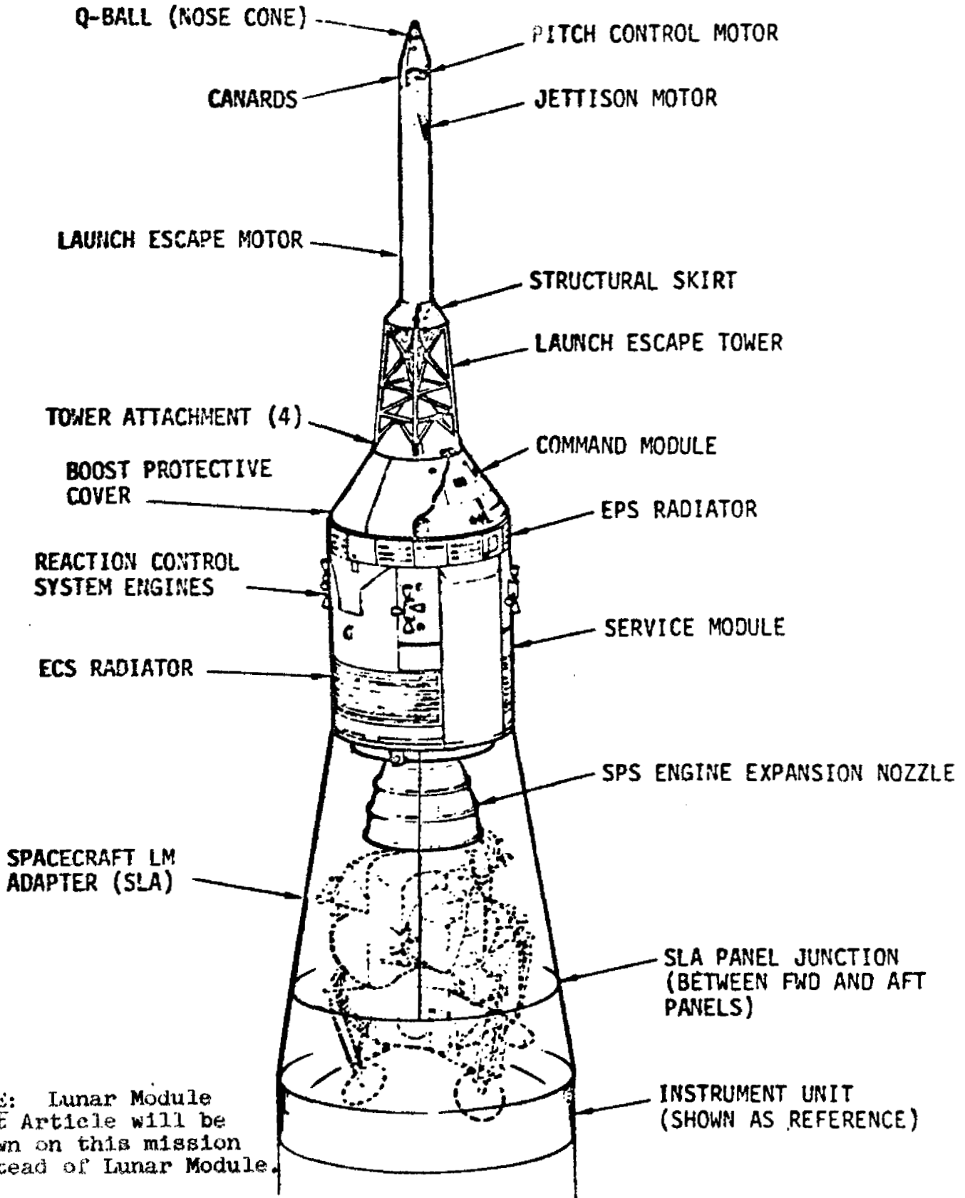
SPACECRAFT CONFIGURATION
