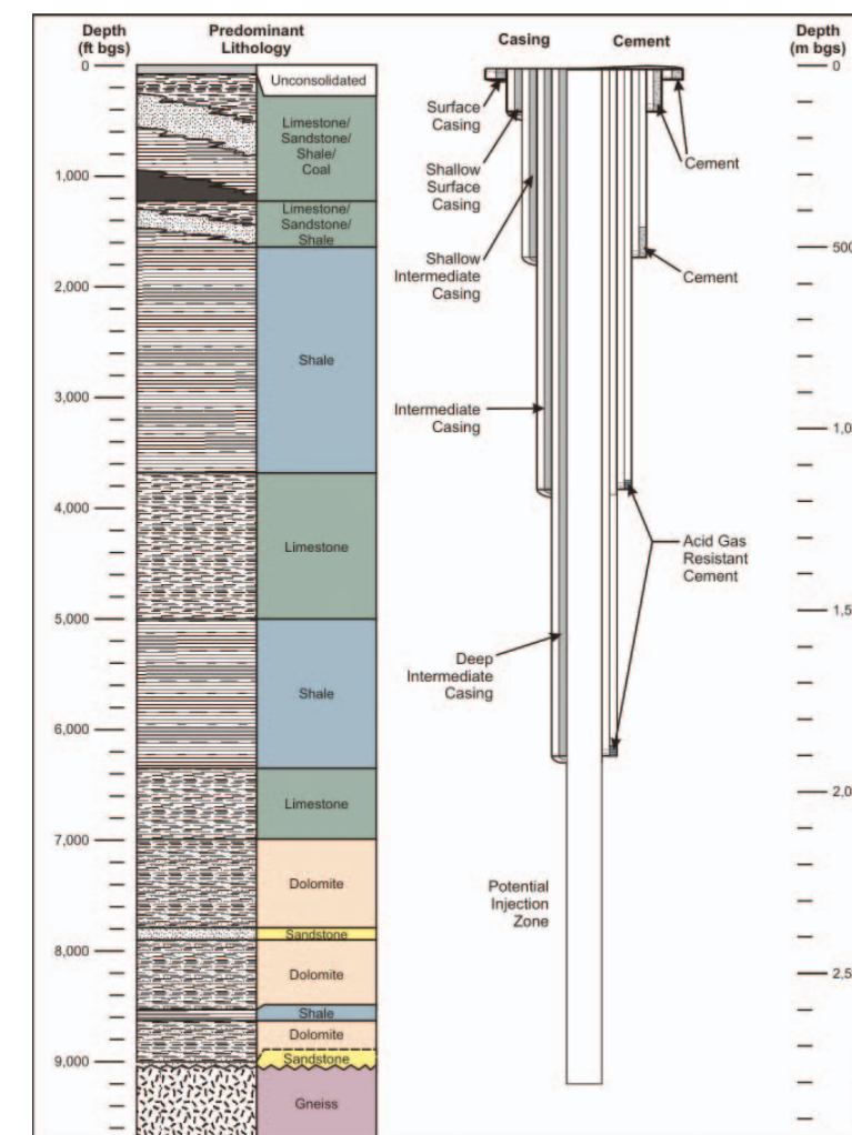
▲ CO 2 injection wells are engineered systems designed to ensure that injected CO 2 only reaches the appropriate storage formation.
