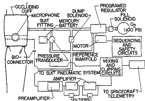
FIGURE 3-16.—Block diagram of automatic BPMS.
