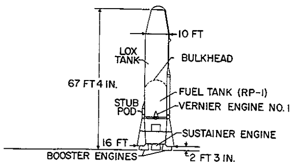
FIGURE 4-3.—Standard Atlas D launch vehicle.
