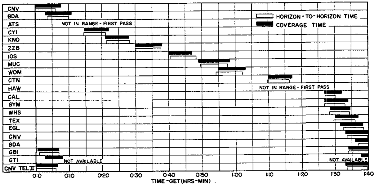
FIGURE A-7. Telemetry reception coverage, first orbit.
