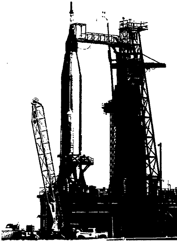
FIGURE 4-8.—Emergency egress tower.
