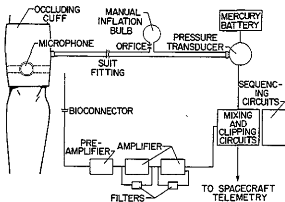
FIGURE 3-18.—Block diagram of manual BPMS.
