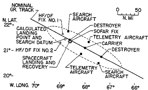
FIGURE 7-5.—MA-6 landing area.
