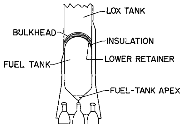
FIGURE 4-14.—Bulkhead between fuel and liquid oxygen tanks.
