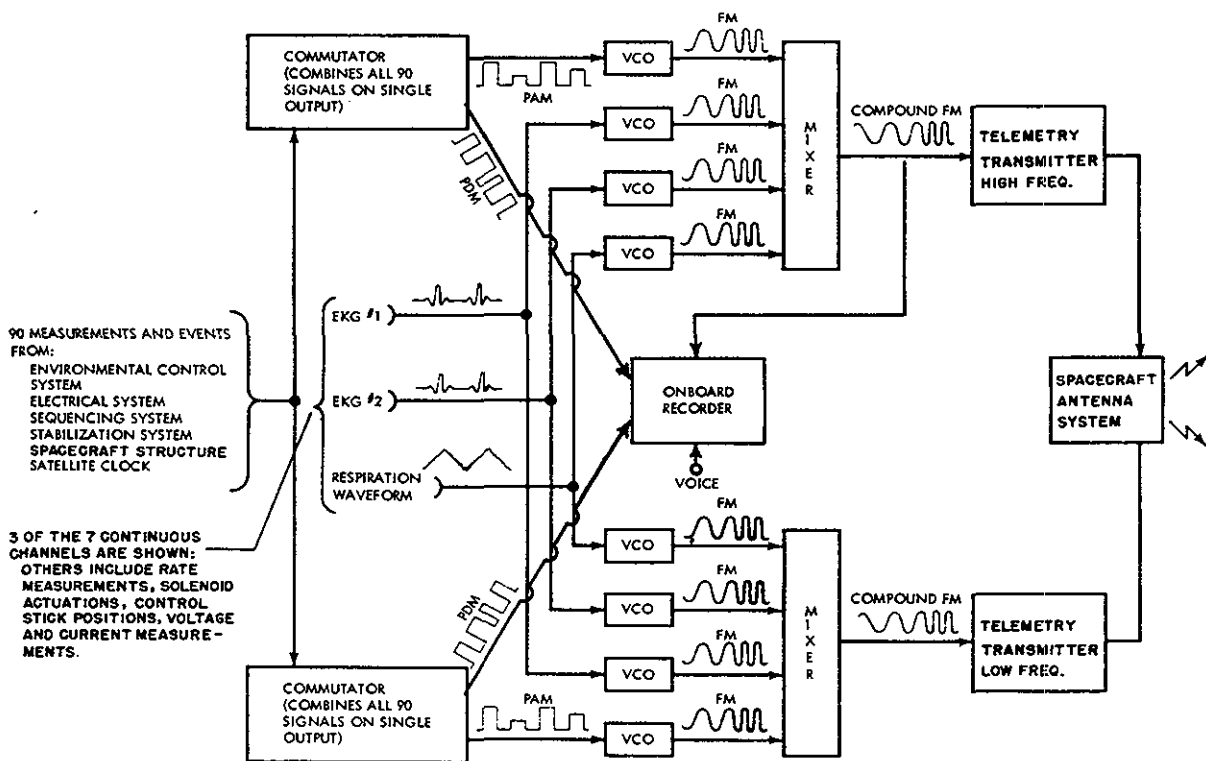
FIGURE 2-18.—Instrumentation system schematic diagram.
