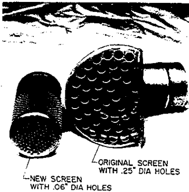
FIGURE 5-5.—Cooling fan duct inlet screens for Friendship 7 and Spacecraft 9.
