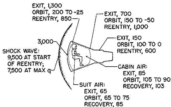
FIGURE 2-7.—Representative temperatures in degrees Fahrenheit.
