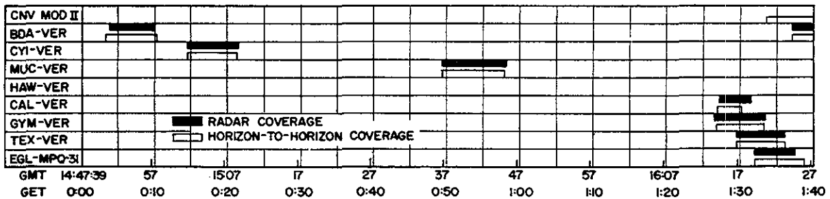
FIGURE A-4. S-band radar coverage, first orbit.
