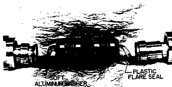
FIGURE 5-2.—Reaction Control System flare seals.
