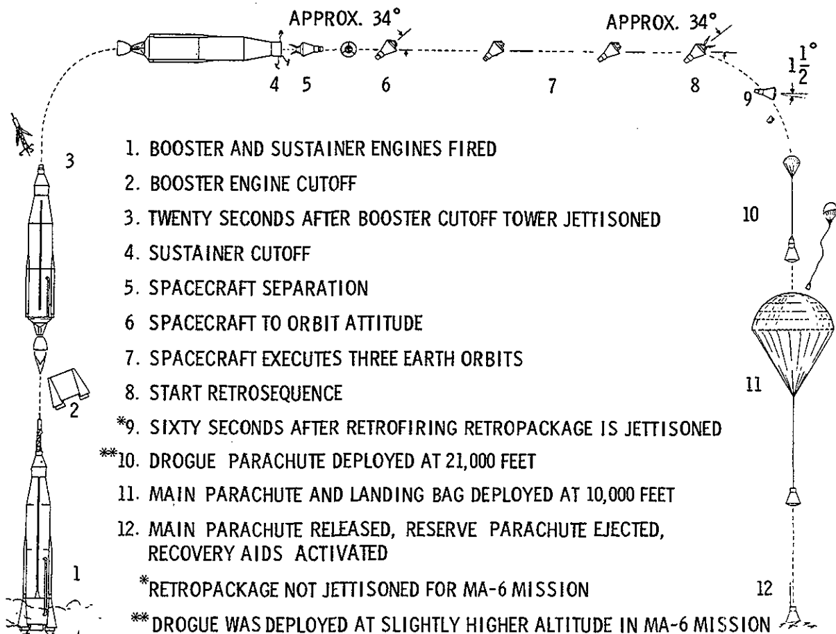
FIGURE 2-22.—Sequence of major events for the MA-6 mission.
