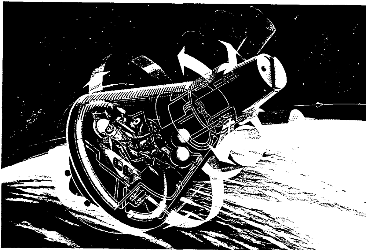
FIGURE 2-11.—Arrangement of reaction control system.
