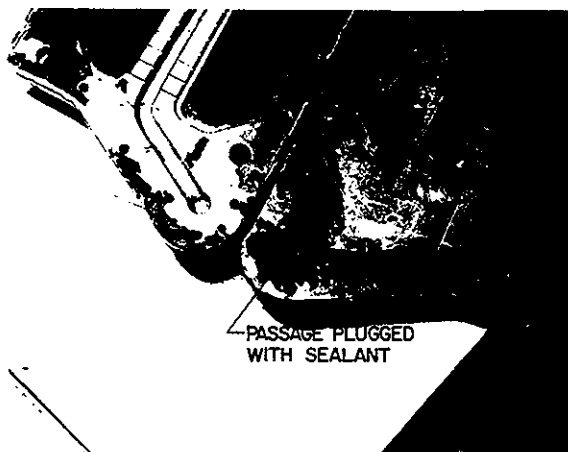
FIGURE 5-16.—Plugged inlet part of cooling plate for 150 v-amp inverter.
