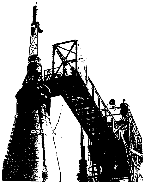
FIGURE 5-24.—Emergency egress tower ramps in place during emergency egress tests.
