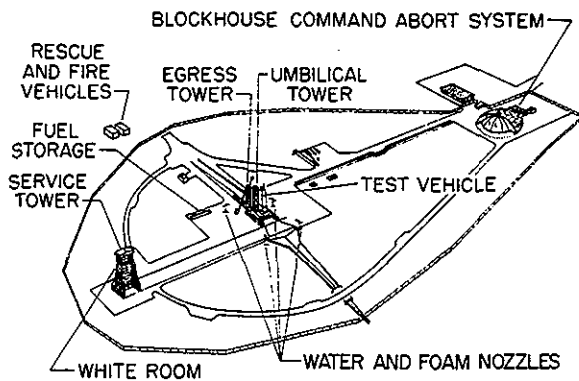
FIGURE 4-5.—Mercury modifications to launch complex.
