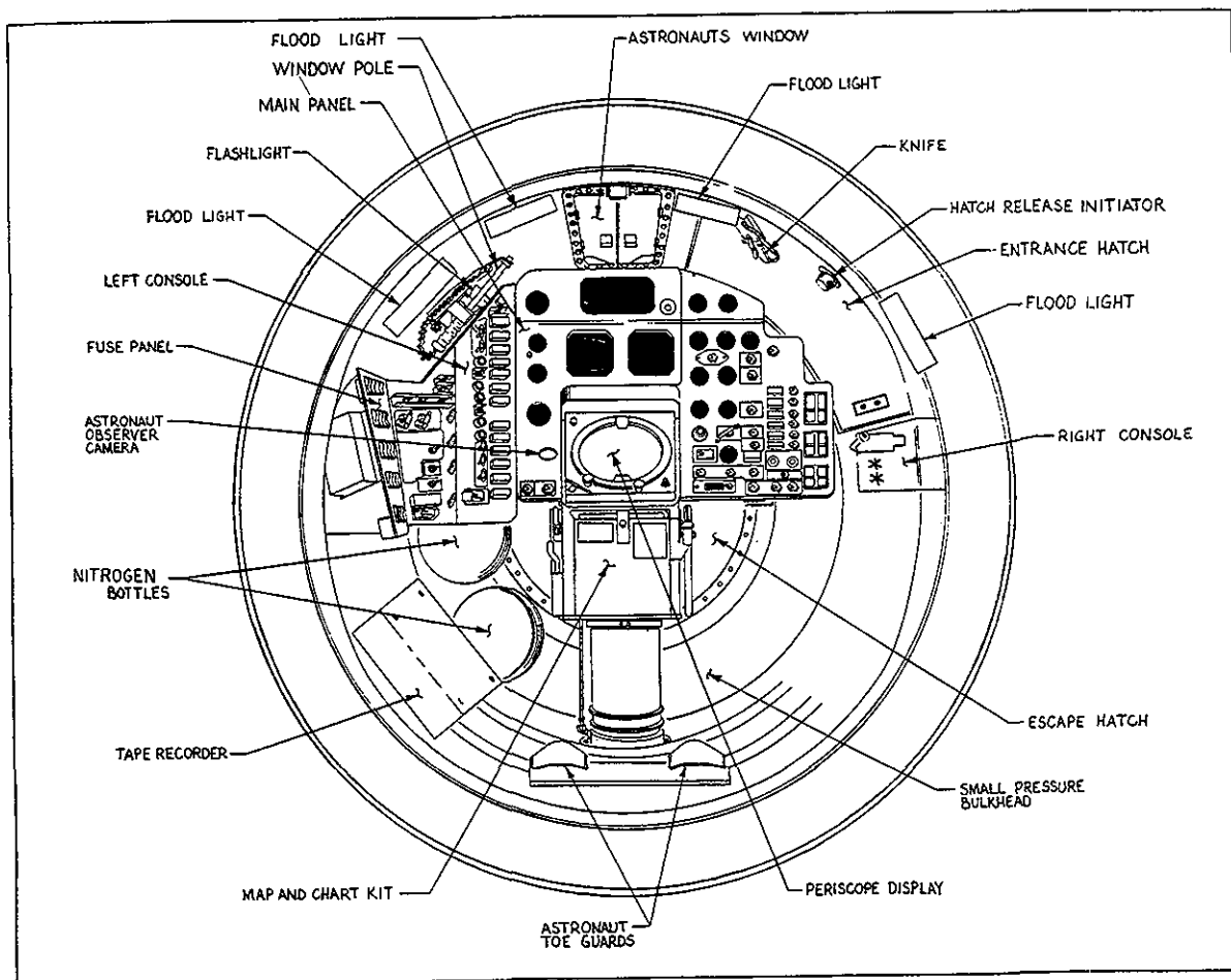
FIGURE 2-3.—Spacecraft cabin arrangement.
