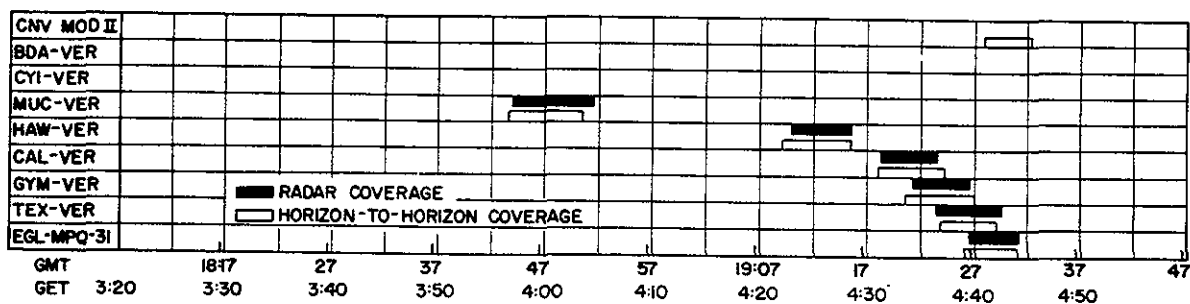
FIGURE A-6. S-band radar coverage, third orbit.
