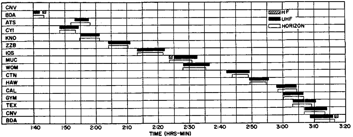
FIGURE A-11. HF and UHF communications, second orbit.
