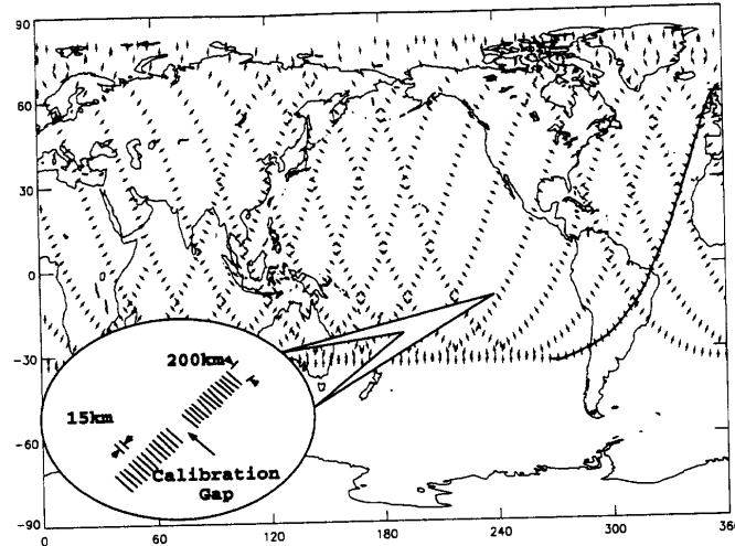
Figure 2. UARS/MLS sampling tracks on 28 December 1994 marked by the first measurement of each major frame (65.5 seconds). The inset details the set of individual measurements in a single major frame with the short lines indicating the orientation of the temperature weighting functions (see text). On this day MLS was preferentially observing the Northern Hemisphere. The ascending portion of orbits 1 is highlighted with solid lines.
