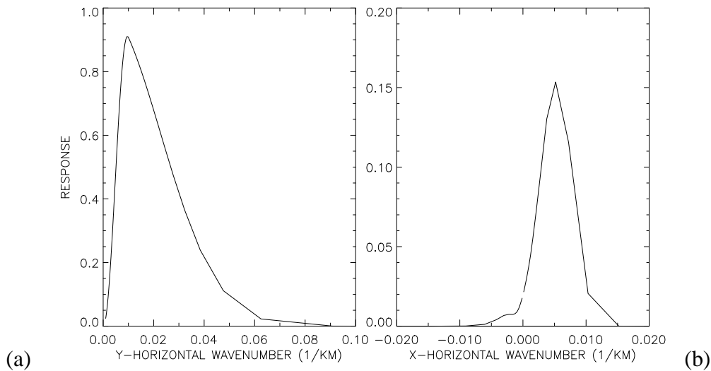
Figure 8. Radiance responses to the horizontal wavenumbers (a) along and (b) cross the track. The response function in (a) is a simple convolution of a 6-point ( \sim 90 km) truncation functions and along-track smearing, while the response function (b) is calculated by convolving the instrument weighting function (Figure 6b) with a 1 K monochromatic wave that has a 10 km vertical wavelength. For a given vertical wavelength, positively propagating waves have wavefronts more parallel to the MLS field of view direction.
