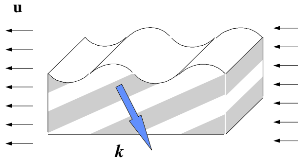
Figure 14. Gravity wave propagation in a background wind, as suggested by the MLS wave variance observations, showing the zonal wave vector k_\lambda in opposite of the wind velocity \mathbf{u} .
