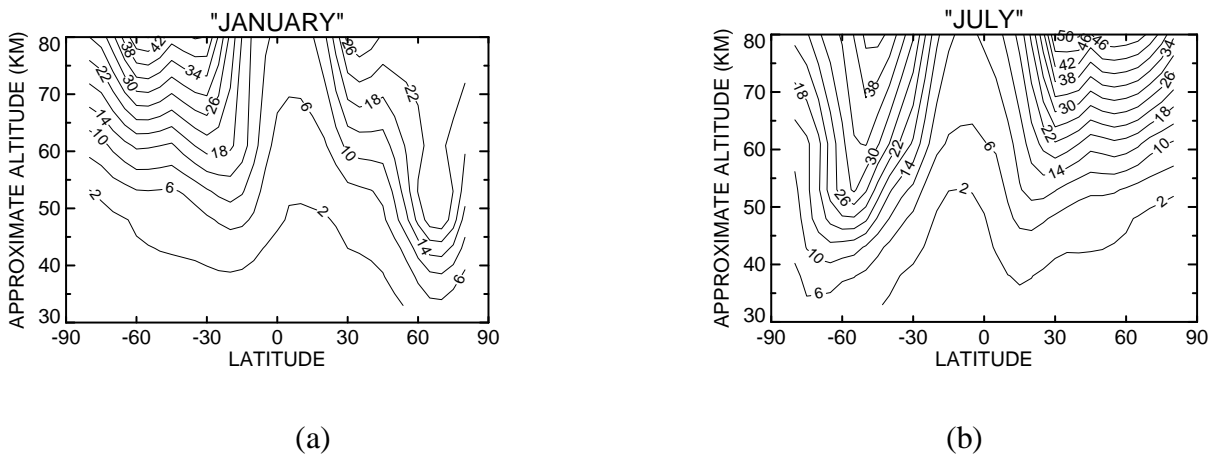
Figure 12. Zonal mean normalized GW variances for (a) January and (b) July. Contours are in units of 10^{-7} .
