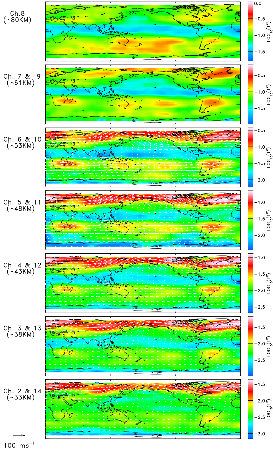
Figure 10(a). Maps of gravity wave variances for January. Latitude and longitude bins are respectively 5^\circ and 10^\circ with more than 40 measurements in each grid point. The variances are in a unit of \text{K}^2 and colored in a logarithmic scale, i.e., \log_{10}(\sigma_{GW}^2) . Winds (up to \sim 1 hPa) are derived from the US National Meteorological Center data [Manney et al. 1994] and averaged over the same periods.
