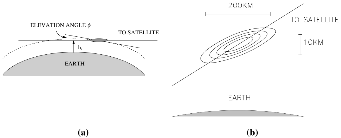
Figure 6 (a) Observing geometry for MLS saturated radiances. (b) Detailed weighting functions in the saturation region where the line of sight is indicated by the straight line. The weighting function in (b), normalized by its peak, is contoured at 0.2, 0.4, 0.6 and 0.8 from edge to center, while the line of sight is indicated by the straight line.
