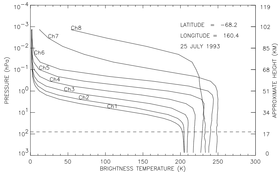
Figure 1. An example of MLS O 2 radiance profiles near 63 GHz as the instrument step-scans from the mesosphere to the surface. Fluctuations in the saturated radiances are generally large for center channels but small for wing channels due to atmospheric temperature variability and instrument noise.
