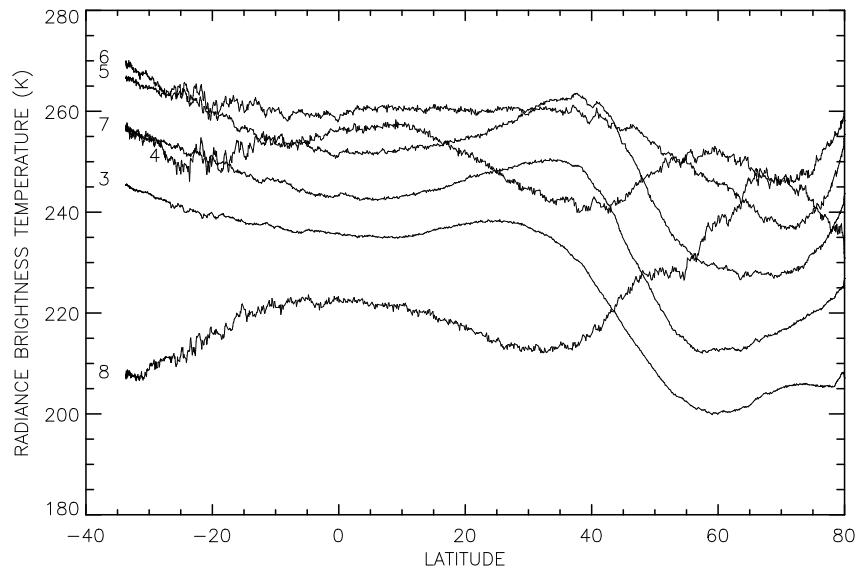
Figure 3. Channel 3-8 radiance measurements from the ascending part of orbit 1 on 28 December 1994.
