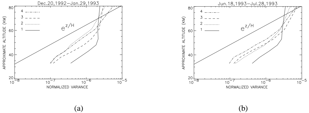
Figure 11. Variance growth at different latitudes during (a) January and (b) July compared with the exponential growth expected for non-breaking GWs. The variances are normalized by the squared mean radiance brightness temperature.
