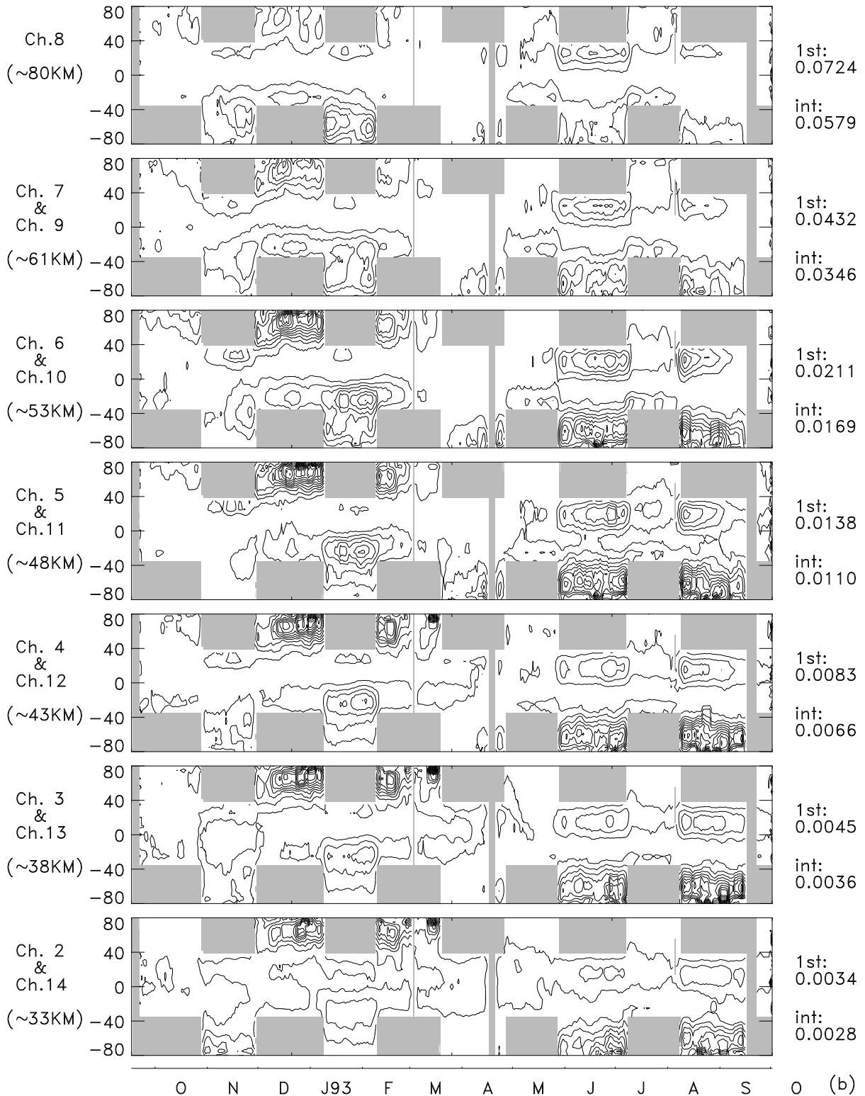
Figure 13(b). As in Figure 13(a) but for descending measurements.. As a result of the yaw maneuver, the MLS viewing direction changes at a given latitude, providing an opportunity for observing wave propagation directions. To the first-order approximation, the variance differences between ascending and descending measurements are caused by the angle variations between the instrument FOV and wave vectors.
