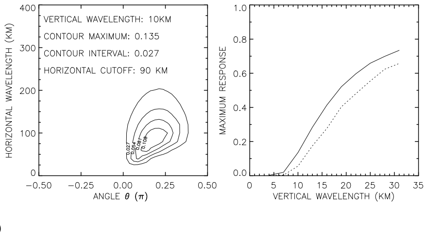
Figure 9. MLS radiance response as a function of (a) horizontal wavelength and observing angle \theta and (b) vertical wavelength. The radiance responses in (b) correspond to the peak value in (a), where the solid (dashed) line is for channel 1 (8).
