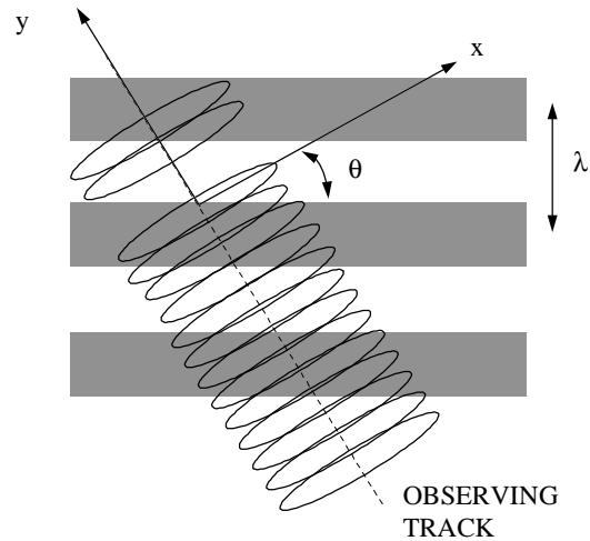
Figure 7. Temperature weighting functions of the saturated radiances projected on the horizontal plane. The footprints of the weighting function move across wavefronts (shaded) with an angle \theta , and k = 2\pi/\lambda .
