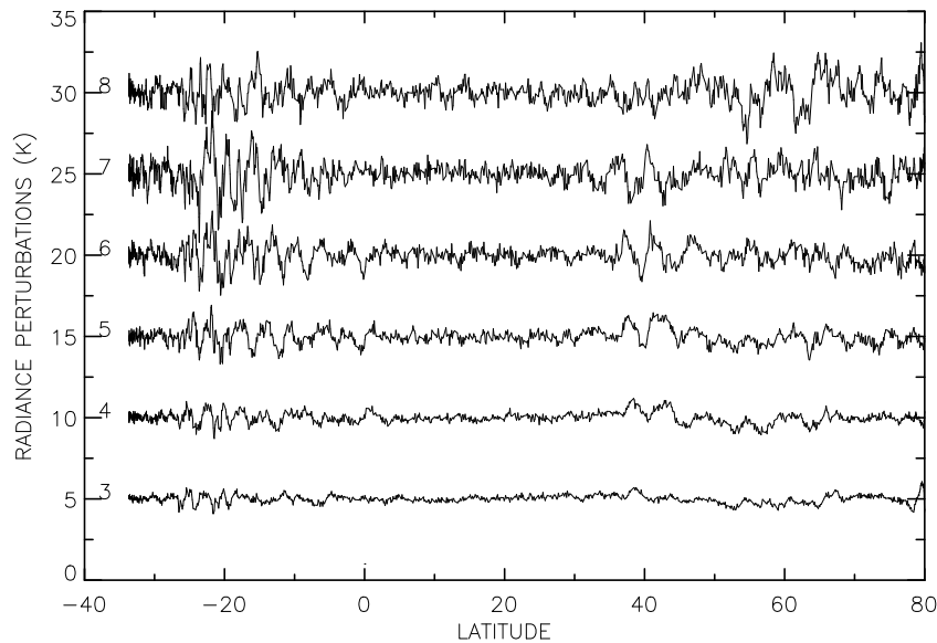
Figure 4. Radiance fluctuations derived from Figure 3 with large-scale ( >1000 km) variations removed. Radiance fluctuations of each channel are displaced by 5 K with the channel number indicated at the left of each measurement series. There are more samples near the turning latitudes at 34^\circ\text{S} and 80^\circ\text{N} than elsewhere. In the middle portion of the orbit, a 10^\circ latitude band corresponds to a distance of \sim 1300 km.
