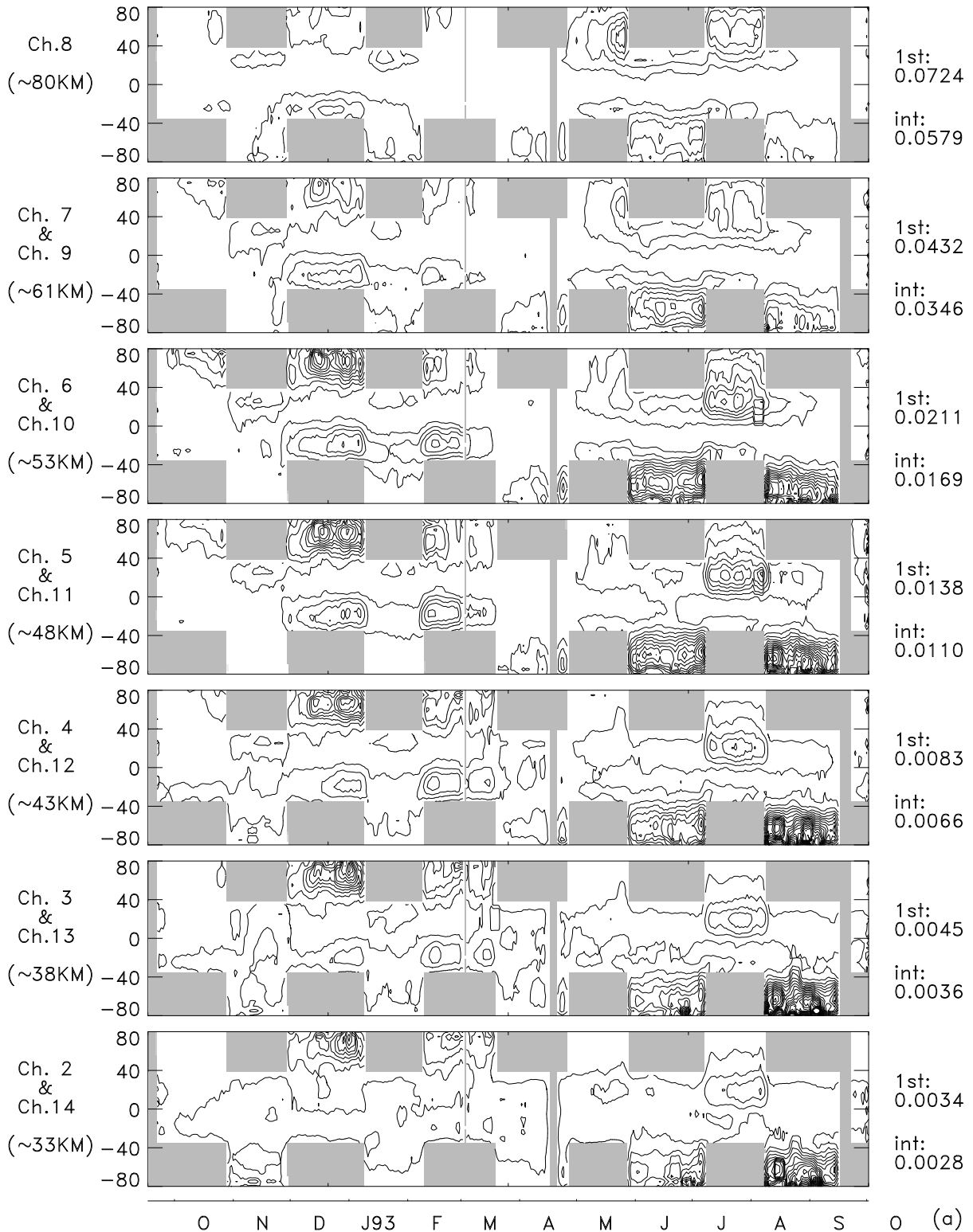
Figure 13(a). Time-latitude plots of daily GW variances for ascending measurements. The first contour and contour interval, in units of K^2 , are noted on the right of each panel. A 5-day smoothing is employed for each latitude band with data gaps highlighted by shaded areas. The large data gaps alternated at high latitudes are caused by the UARS yaw maneuvers. At a given latitude the MLS looking angle with respect to the atmosphere is approximately the same for an entire UARS month.
