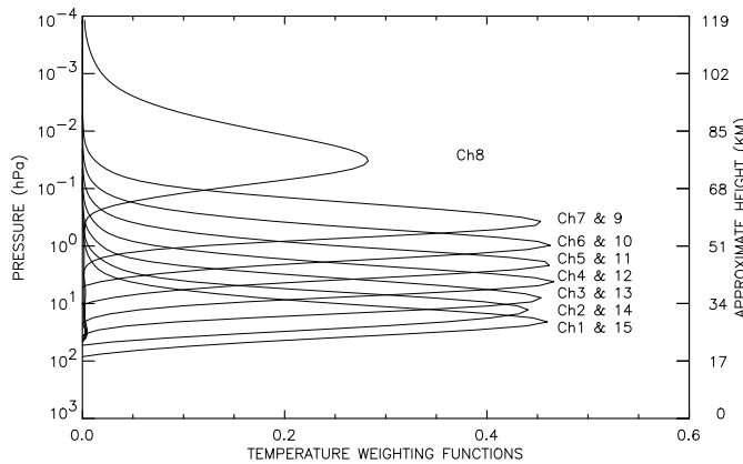
Figure 5 Temperature weighting functions of channels 1-15 for the MLS 63 GHz radiometer viewing the limb at 18 km (calculated by W. G. Read).
