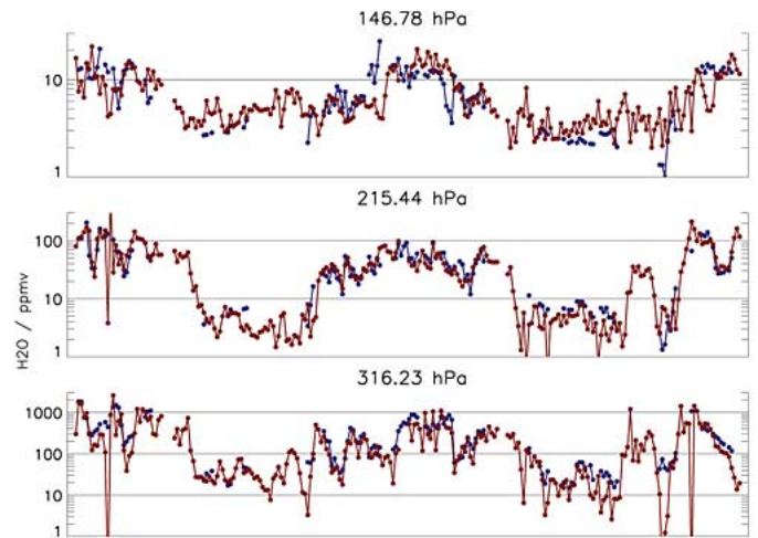
Fig. 13. Typical comparison between MLS (red) and AIRS (blue) retrieved H 2 O abundances in the upper troposphere at the pressures indicated, for one orbit on November 5, 2004. Time goes from right to left, and the orbit starts at the equator descending node. According to quality acceptance criteria for each of these datasets, the fraction of rejected profiles along the MLS track is \sim 3\% for MLS and 51% for AIRS, based on the two days that we have analyzed so far.
