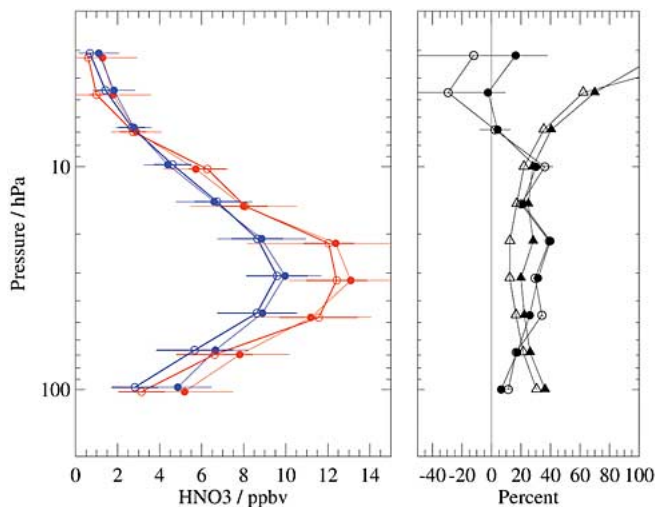
Fig. 20. As Fig. 3, but for MLS and ACE HNO_3 comparisons. A total of 621 matched profiles was used in this case.
