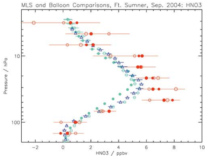
Fig. 21. Similar to Fig. 8, but for \text{HNO}_3 Ft. Sumner data versus MLS; MLS profiles (red symbols) are compared to MkIV (blue triangles) and FIRS-2 (cyan) profiles on September 23–24, 2004.
