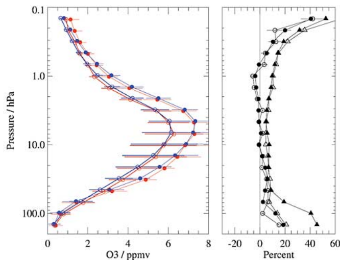
Fig. 4. As Fig. 3, but for MLS and HALOE O_3 comparisons; 303 matched profiles were used in this case, with a time coincidence criterion of \pm 6 h.
