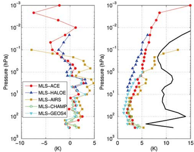
Fig. 1. (Left) Mean MLS-minus-comparison-set temperature differences averaged over sets of matched (“coincident”) profile pairs from the first three months of 2005. The AIRS and CHAMP pairs are only from January, but have 12 438 and 3074 matched profiles with MLS, respectively. The HALOE comparisons include 284 matched profiles, while the ACE comparisons include 525 matches. The GMAO comparisons lead to a large number of matched profiles, namely over 215 000. (Right) Standard deviations of these differences, for each set of profile pairs. The thick black line is the standard deviation of all MLS profiles in the three-month period.
