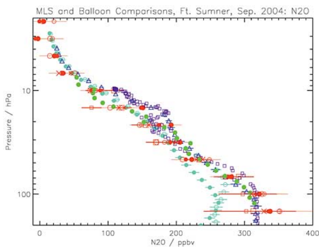
Fig. 19. Similar to Fig. 8, but for N_2O Ft. Sumner data versus MLS; MLS profiles (red symbols) are compared to MkIV (blue triangles) and FIRS-2 (cyan) profiles on September 23–24 2004. Also shown is the LACE September 17 ( in situ ) N_2O profile (purple squares), to be compared to the MLS values (red squares) for that day, and the CWAS profile (green dots) of September 29 ( in situ ), to be compared to the MLS values (red crosses) for that day. Error bars are not shown for LACE or CWAS but these should be quite small (less than 1% to 2% total error).
