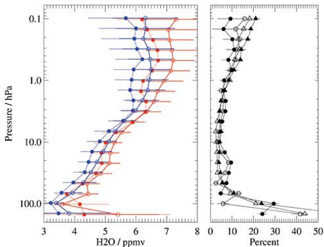
Fig. 9. As Fig. 4, but for MLS and HALOE H_2O comparisons. A total of 326 matched profiles was used in this case.
