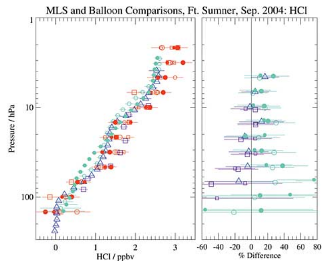
Fig. 17. Similar to Fig. 8, but for HCl data. (Left) This compares MLS (red symbols) to MkIV (blue triangles) and FIRS-2 (cyan) profiles on September 23–24, 2004. Also shown (purple squares) is the ALIAS-II September 17 ( in situ ) HCl profile retrieval, to be compared to the MLS values (red squares) for that day. (Right) Percent differences (for MLS minus balloon data) are shown, with symbols referring to the balloon measurements mentioned in the left panel caption. Error bars give twice the random error in these differences.
