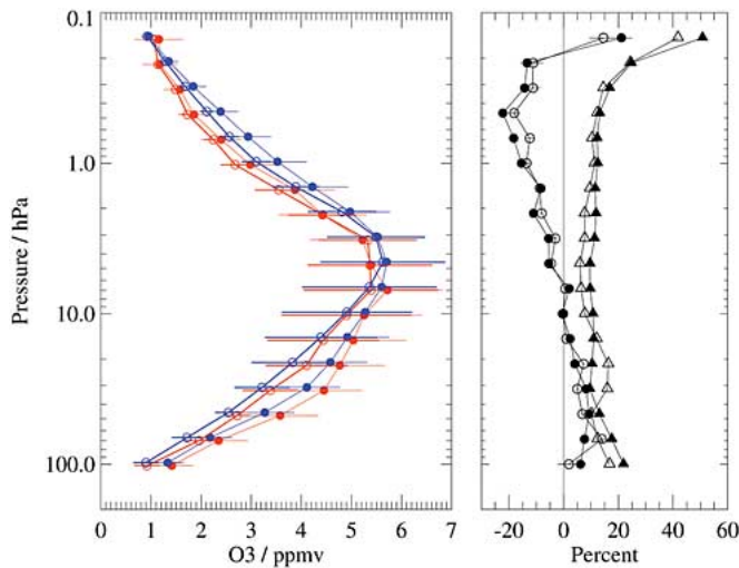
Fig. 6. As Fig. 3, but for MLS and ACE O 3 comparisons. A total of 622 matched profiles was used in this case.
