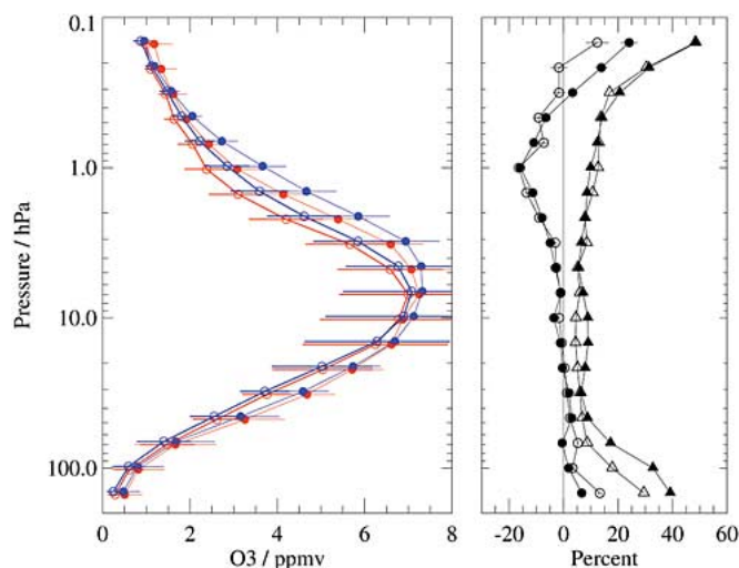
Fig. 3. MLS and SAGE II O_3 comparisons. (Left) Averages of the matched profiles from (red) MLS and (blue) SAGE II, with closed and open circles corresponding to NH and SH profiles. The standard deviation of the profiles is shown by the error bars; a slight shift in pressure between the MLS and other datasets is introduced for clarity, but the SAGE II profiles have been interpolated to the MLS retrieval grid for these plots. (Right) Average differences (circles) are given for MLS minus SAGE II abundances, expressed as a percent difference from the corresponding average SAGE II profile, with error bars representing twice the estimated error in the means; if no error bar is apparent, it is small and hidden by the symbol itself. Also shown are the standard deviations of the differences (triangles), with closed and open symbols referring to the NH and SH, respectively. A total of 873 profiles was used in these matched comparisons; a match means the use of the closest MLS profile within plus or minus 1^\circ latitude and 12^\circ longitude of each SAGE II profile, and within 24 h (on same day).
