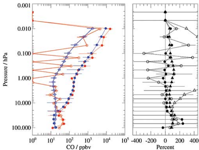
Fig. 22. As Fig. 3, but for MLS and ACE CO comparisons, and with a log axis for mixing ratio. A total of 616 matched profiles was used in this case. In the left-hand panel, mixing ratios less than 1 ppbv (or negative) are set to 1 ppbv to better display the oscillation in the average MLS profiles.
