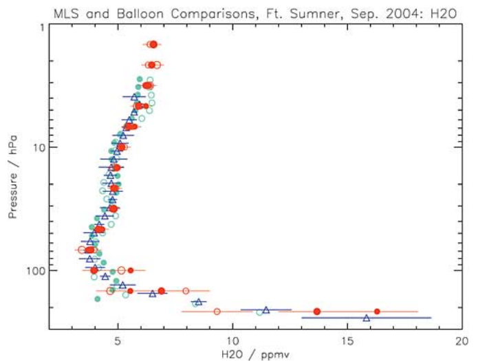
Fig. 14. Similar to Fig. 8, but for H 2 O Ft. Sumner data versus MLS; MLS profiles (red symbols) are compared to MkIV (blue triangles) and FIRS-2 (cyan) profiles on September 23–24, 2004.
