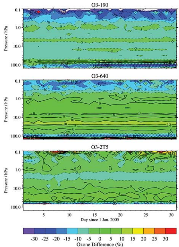
Fig. 7. Percent differences between the various MLS retrievals of O 3 (top panel for 190 GHz, middle panel for 640 GHz, and bottom panel for 2.5 THz) and the standard (240 GHz) MLS O 3 retrieval during January 2005. A positive difference means that the nonstandard ozone product gives a larger value than the standard product.
