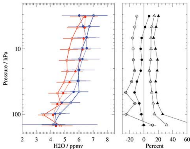
Fig. 12. As Fig. 5, but for MLS and POAM III H 2 O comparisons.
