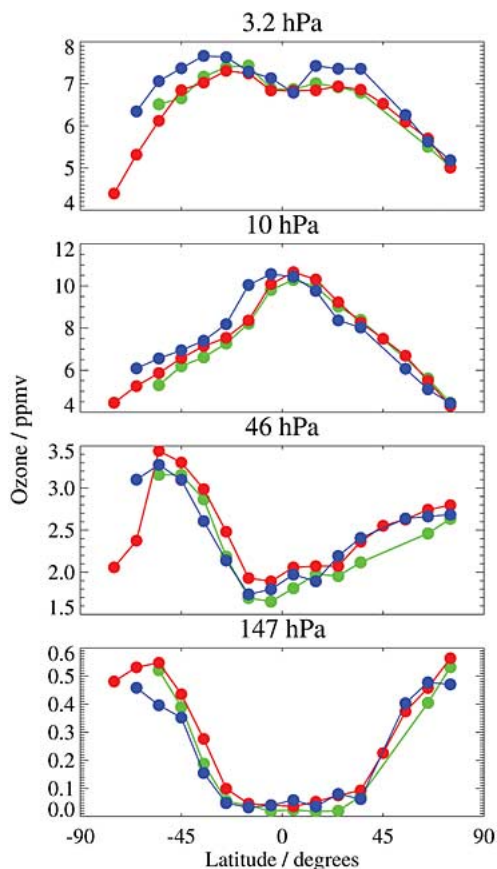
Fig. 2. Early sample comparison between zonal mean (red) MLS, (blue) SAGEII, and (green) HALOE ozone measurements as a function of latitude at four pressure levels. The MLS measurements are for August 30, 2004, in 10^\circ latitude bins. The SAGE II and HALOE data combine sunrise and sunset occultations in the same latitude bins, using all August occultations for HALOE and all August and September data for SAGE II.
