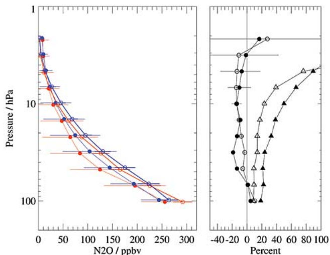
Fig. 18. As Fig. 3 but for MLS and ACE N_2O comparisons. A total of 622 matched profiles was used in this case.
