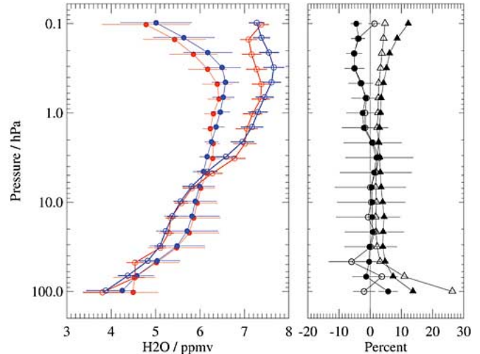
Fig. 10. As Fig. 3, but for MLS and ACE H_2O comparisons. A total of 616 matched profiles was used in this case.
