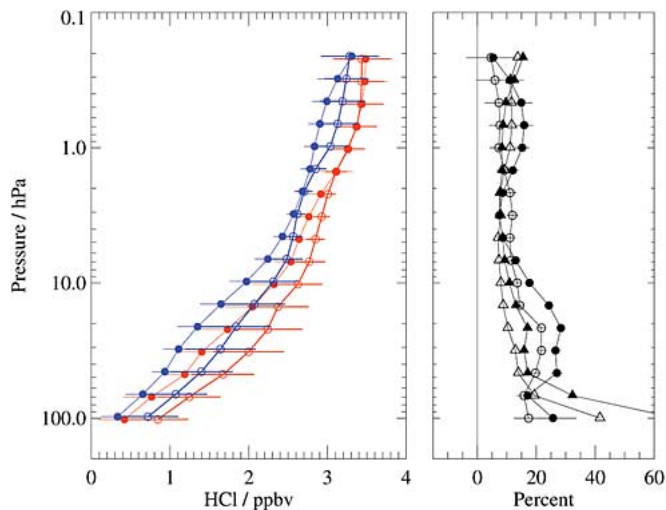
Fig. 15. As Fig. 4, but for MLS and HALOE HCl comparisons. A total of 329 matched profiles was used in this case.
