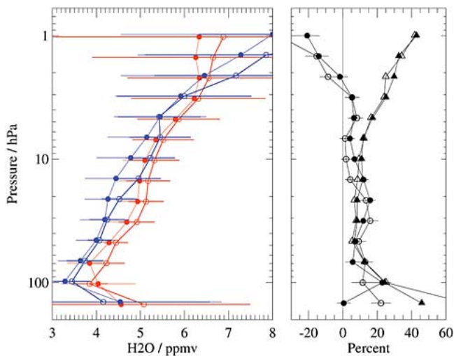
Fig. 11. As Fig. 3, but for MLS and SAGE II H 2 O comparisons. A total of 273 matched profiles was used in this case, with a time coincidence criterion of plus or minus 6 h.
