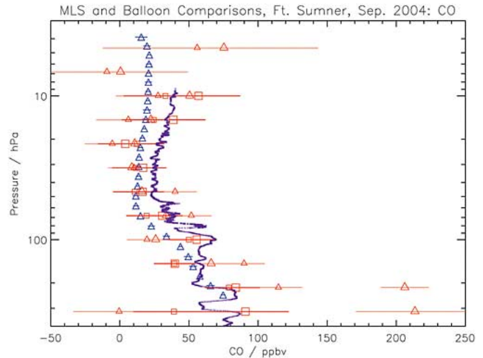
Fig. 23. Similar to Fig. 8, but for CO data; this compares MLS (red symbols) to MkIV (blue triangles) on September 23, 2004. Also shown (fine resolution line of purple crosses) is the ALIAS-II September 17 ( in situ ) CO profile retrieval, to be compared to the MLS values (red squares) for that day. Note the possible high bias in ALIAS-II stratospheric values versus MkIV data; this may be caused by contamination of ALIAS-II data, as mentioned in Section I.
