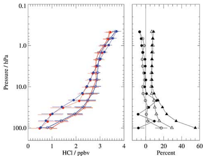
Fig. 16. As Fig. 3, but for MLS and ACE HCl comparisons. A total of 623 matched profiles was used in this case.
