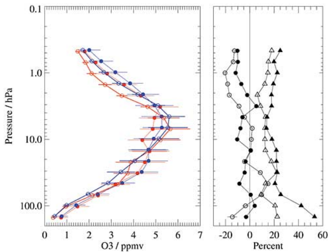
Fig. 5. As Fig. 3, but for MLS and POAM III O 3 comparisons, and with a tighter time coincidence criterion of (plus or minus) 3 h; see text. A total of 407 matched profiles was used in this case.
