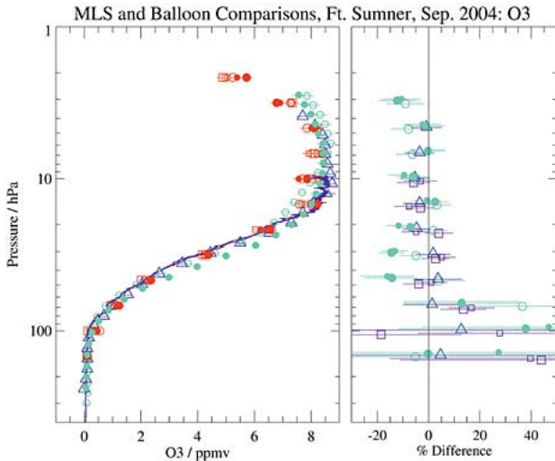
Fig. 8. MLS O_3 compared to Ft. Sumner balloon flight measurements in September 2004. (Left) As explained in the text, the two closest MLS profiles for daytime and nighttime are plotted for mid day on September 23 and the early morning of September 24, respectively. Open red circles are for daytime MLS profiles, with the larger symbol being for the closest profile to the FIRS-2 profile (open cyan circle) that is closest in time to the daytime Aura overpass. Closed red circles are the same but for the nighttime FIRS-2 profile (closed cyan circle) closest in time to the nighttime Aura overpass. Open blue triangles are the profile from MkIV sunset data on the evening of September 23, to be compared to the daytime MLS profiles. Error bars on the MLS and remote balloon measurements are based on estimated errors from each experiment (essentially the random error component). The purple fine resolution profile is from the OMS in situ photometer data, for September 17; this is to be compared to the two open red squares, representing the two closest daytime MLS profiles for that day's flight. (Right) Percent differences (for MLS minus balloon data) are shown, with symbols referring to the balloon measurements listed in the left panel caption, but with open squares for the in situ photometer comparison. Error bars give twice the random errors in these differences.
