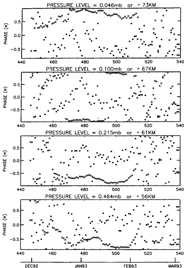
FIG. 6. Time series of the 2-day wave phases at 20°S (circles) and 20°N (filled circles) for selected pressure levels 0.46, 0.22, 0.1, and 0.046 mb. The out-of-phase relation at these levels suggests the existence of the global (3, 0) Rossby normal mode.
