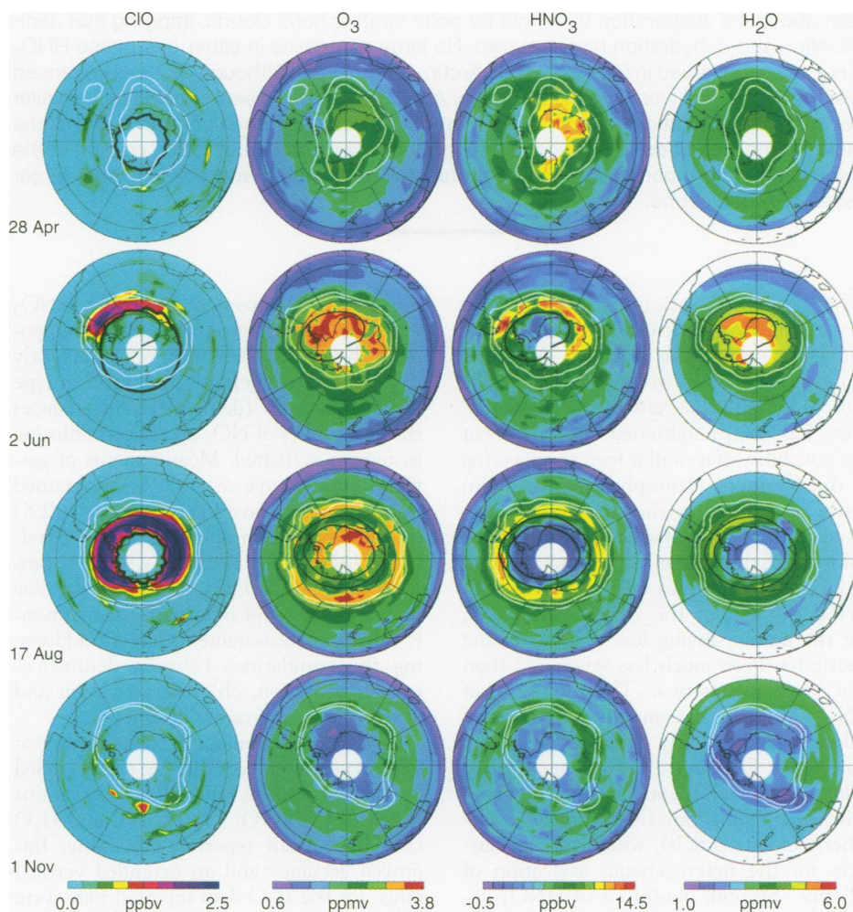
Fig. 1. Maps of MLS HNO 3 , ClO, O 3 , and H 2 O for selected days during the 1992 southern winter, interpolated onto the 465 K potential temperature (17) surface with U.S. National Meteorological Center (NMC) temperatures. The maps are polar orthographic projections extending to the equator, with the Greenwich meridian at the top and black circles at 30° and 60°S. They were produced by linear interpolation of measurements taken over a 24-hour period. The nonlinear H 2 O retrieval was performed poleward of 30°S, and no measurements were obtained in the white area poleward of 80°S. The thick black contours on the ClO maps identify the edge of daylight for the measurements; only data from the “day” side of the orbit are shown for ClO (34). Thin black lines show NMC temperature contours of 195 K (outer contour) and 188 K (inner contour), the approximate threshold temperatures (6) for type I and type II PSCs, respectively. Also superimposed (in white) on each of the maps are two contours of potential vorticity (PV) (18), calculated from NMC temperature and geopotential height fields. The outer contour ( -2.5 \times 10^{-5} \text{ K m}^2 \text{ kg}^{-1} \text{ s}^{-1} ) represents the approximate edge of the polar vortex during winter when it is well established (12); inclusion of the inner contour ( -3.0 \times 10^{-5} \text{ K m}^2 \text{ kg}^{-1} \text{ s}^{-1} ) provides information on the steepness of the PV gradient, indicating the strength of the vortex.
