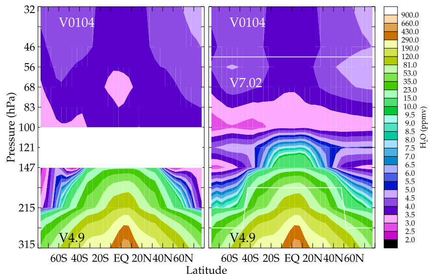
Figure 4. Zonal mean of water vapor versus pressure using MLS data taken in 1992. The left panel is the V4.9 and V0104 data sets. The blank region is where H 2 O is not sampled by either data set. The right panel shows the H 2 O obtained from overlaying the V7.02 data between 147 and 56 hPa on the combined V4.9 and V0104 data. White lines on the right panel indicate the altitude ranges of the respective data set used to produce the figure.
