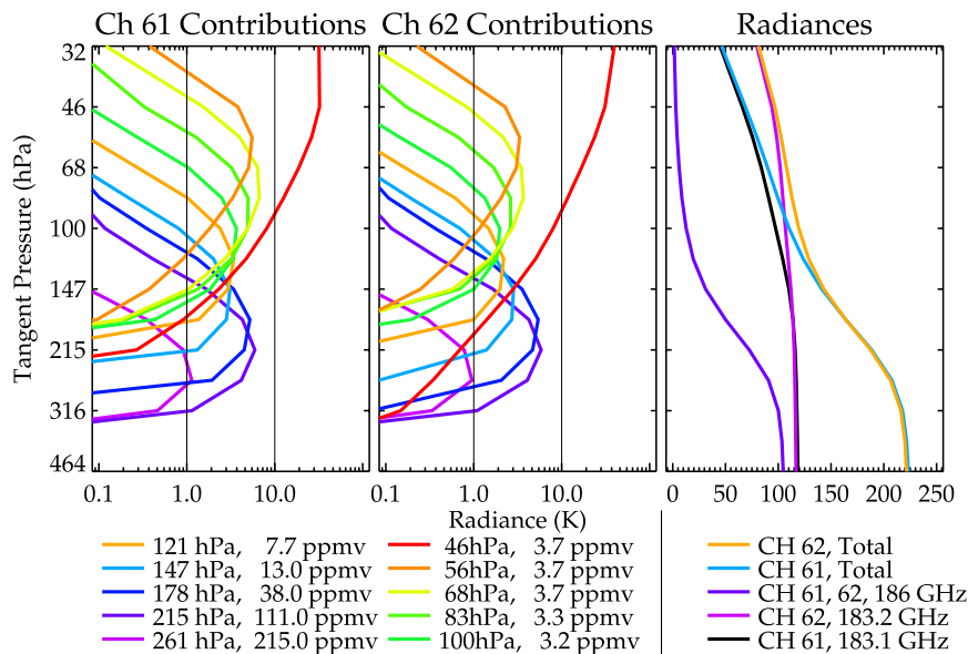
Figure 1. The two left panels show contributions to the radiances measured by MLS channels 61 and 62, respectively, as a function of observation path tangent pressure. The different colors indicate contributions from H 2 O in layers at the different pressures as indicated. The radiance contribution is the radiance Jacobian times the H 2 O concentration in the layer indicated by the color. The rightmost panel shows the sideband fraction weighted radiance signals at 183 GHz and 186 GHz (same for both channels) and the double sideband signals for channels 61 and 62.
