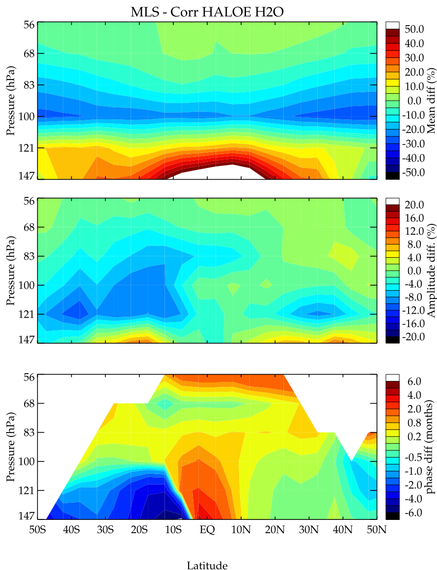
Figure 7. Difference in the zonal H 2 O seasonal cycle amplitude and phase between MLS V7.02 (October 1991 to April 1993) and corrected HALOE V19 (1992–2003). The percent difference in the annual mean (top), the percent difference in the annual cycle relative amplitude (middle), and the phase difference (bottom) in months are shown.
