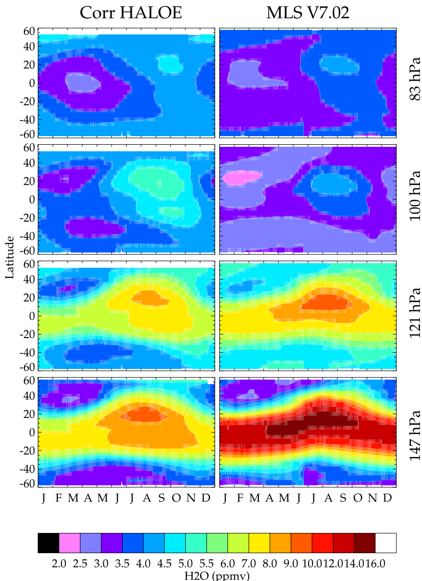
Figure 6. A climatology of zonal means by month and pressure for corrected HALOE V19 (1992–2003) (left panels) and MLS V7.02 (October 1991 to April 2003) (right panels).
