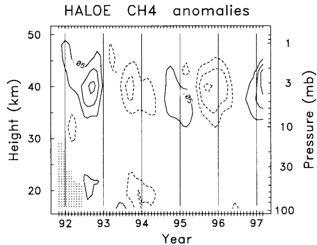
FIG. 19. Altitude-time section of interannual anomalies in \text{CH}_4 over the equator. Contour interval is 0.05 \text{ ppmv} , with zero contours omitted. The vertical lines denote January for each year.
