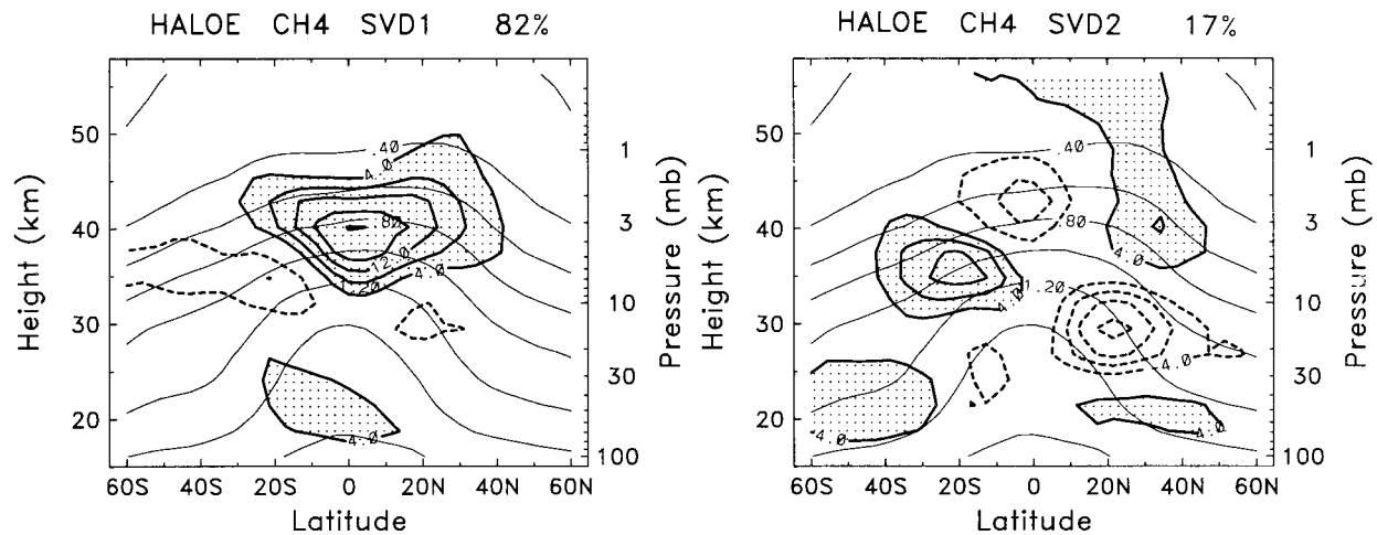
FIG. 22. Heavy solid and dashed lines with shading show the spatial structure of QBO SVD1 (left) and SVD2 (right) for \text{CH}_4 . Contours show local mixing ratio variations with arbitrary units. Light lines denote background annual mean \text{CH}_4 structure.
