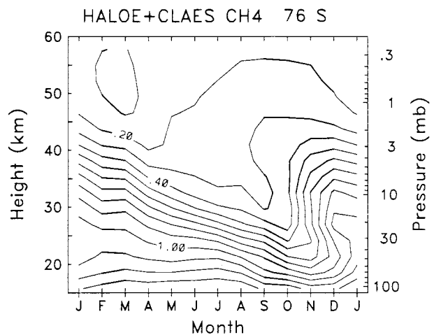
FIG. 11. Altitude–time sections of seasonal cycle variations in \text{CH}_4 at 76^\circ\text{N} (top) and 76^\circ\text{S} (bottom). Contour interval is 0.1 ppmv. Note the respective time axes are shifted by 6 months between the two panels.
