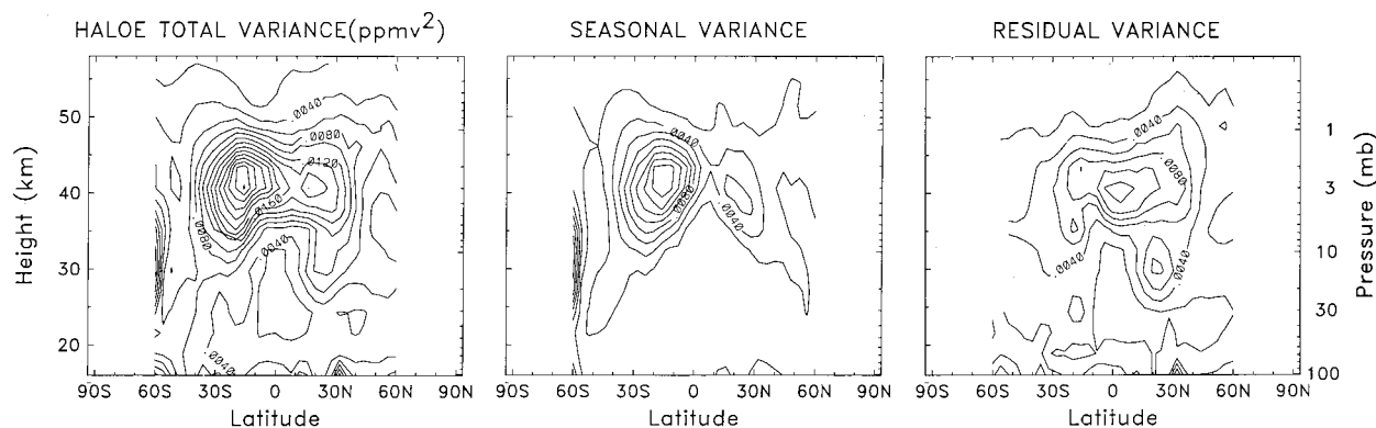
FIG. 5. Components of temporal variance in HALOE \text{CH}_4 data over 1991–97. Shown are total variance (left), seasonal cycle variance (middle), and residual interannual variance (right). Contours in all panels are 0.002 \text{ ppmv}^2 .
