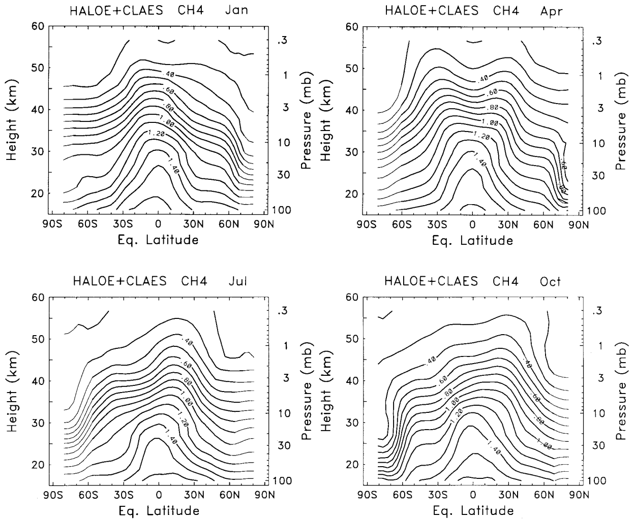
FIG. 6. Seasonal cycle estimates of \text{CH}_4 in January, April, July, and October. Contour interval is 0.1 ppbv.
