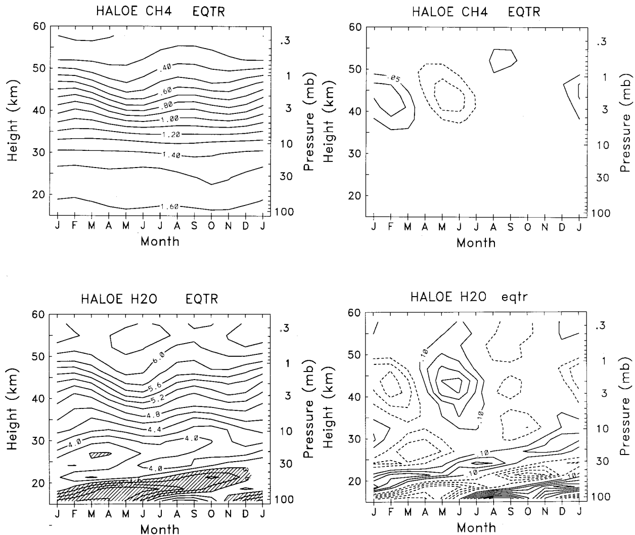
FIG. 14. Altitude–time sections of seasonal cycle variations in \text{CH}_4 (top) and \text{H}_2\text{O} (bottom) over the equator. Left panels show full fields, while right panels show seasonal anomalies (calculated by subtracting the time means at each pressure level). Values below 3.6 ppmv in the lower-left panel are shaded.
