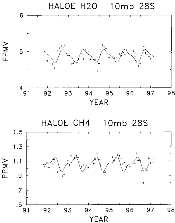
FIG. 3. Time series of HALOE H 2 O and CH 4 data at 10 mb, 28°S. Crosses denote monthly mean data, and thin lines denote (repeating) seasonal cycles fit by harmonic regression.
