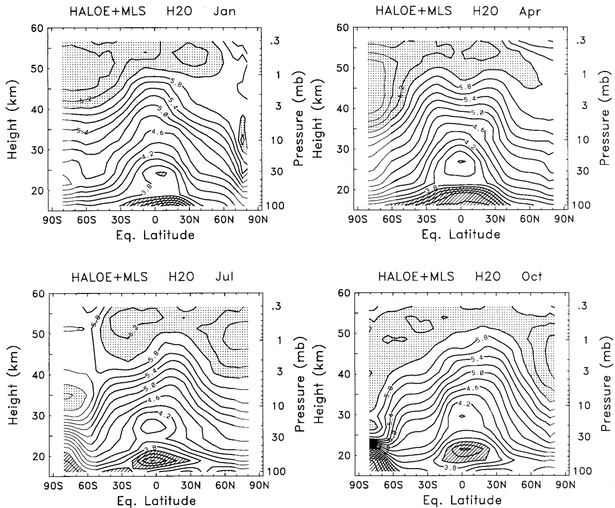
FIG. 7. Seasonal cycle estimates of \text{H}_2\text{O} in January, April, July, and October. Contour interval is 0.2 ppmv. Values below 3.6 ppmv are hatched, and values above 6.0 ppmv are stippled.
