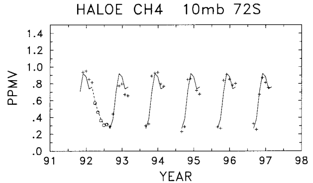
FIG. 4. Time series of CH 4 data at 10 mb, 72°S. Crosses and solid lines denote HALOE observations and fit seasonal cycle; note data are only available during September–February for each year. Circles and dashed lines during 1992–93 show adjusted CLAES data and seasonal cycle fit.
