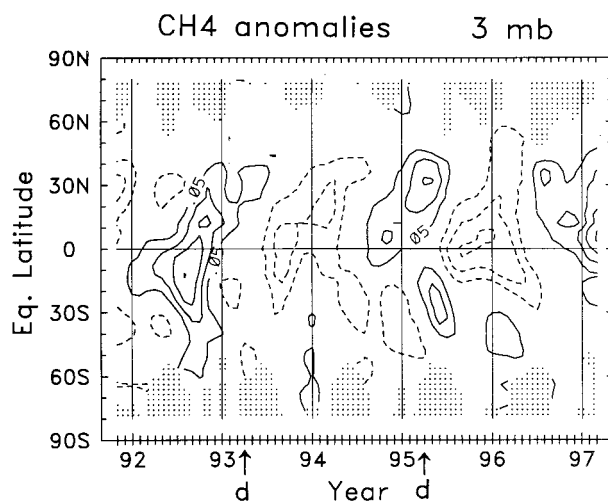
FIG. 25. Latitude–time sections of \text{CH}_4 at 3 mb during 1991–97. Shown are the full field (top) and the detrended interannual anomalies (bottom). Dashed lines and arrows denote periods of double-peaked (d) latitudinal structure.
