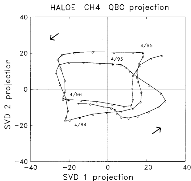
FIG. 23. Phase–space diagram of the projection of the monthly global \text{CH}_4 anomalies onto spatial structures SVD1 and SVD2 (shown in Fig. 22). Time progression corresponds to counterclockwise orbit transits, with locations during several months noted.
