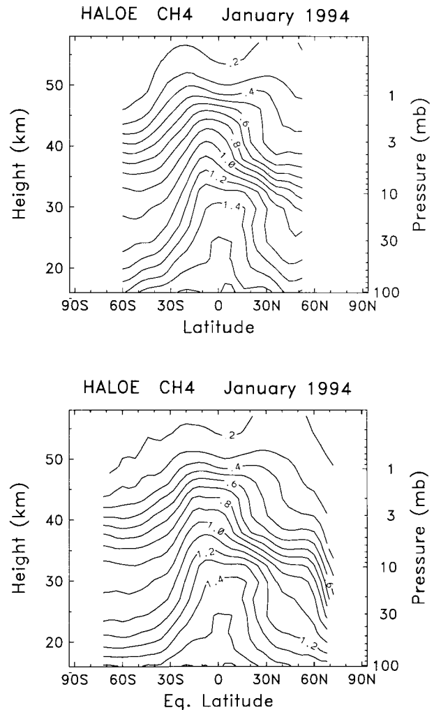
FIG. 2. Comparison of HALOE \text{CH}_4 observations during January 1994 calculated using zonal averages (top) and averages along PV contours (equivalent latitude mapping—bottom).
