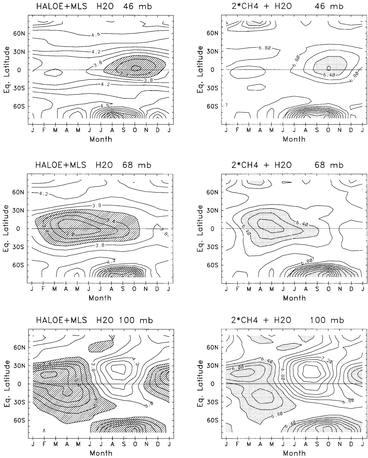
FIG. 16. Latitude–time plots of seasonality in H 2 O (left) and H 2 O + 2CH 4 (right) at 100 mb (bottom), 68 mb (middle), and 46 mb (top). Contour interval is 0.2 ppmv in each panel.
