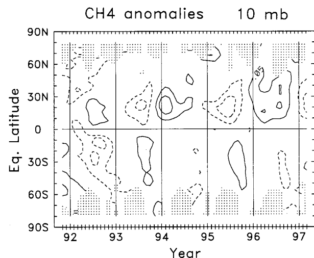
FIG. 26. Latitude–time sections of \text{CH}_4 at 10 mb over 1991–97, for the full field (top—contour interval 0.1 ppmv) and interannual anomalies (bottom—contour interval of 0.05 ppmv, with zero contours omitted).
