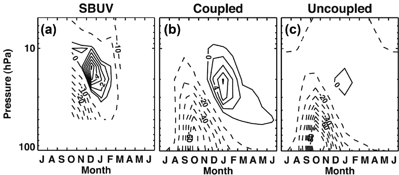
Fig. 20 (a) Summer O_3 trends calculated from SBUV data (1979–2003) for the latitude band between 75^{\circ}\text{S} and 80^{\circ}\text{S} as a function of month of the year. Positive contours are spaced by 1% per decade while negative contours are every 5% per decade. (b) Ozone trend from the GEOS CCM and (c) ozone trend from the GEOS CTM as a function of month and altitude between 75^{\circ}\text{S} – 80^{\circ}\text{S} . In (b) and (c) positive contours are spaced by 2% per decade, while negative contours are spaced by 5% per decade (Stolarski et al. (2006) reproduced by permission of the American Geophysical Union).
