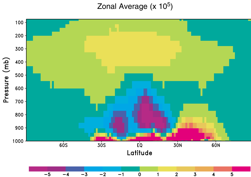
Fig. 2 Zonal and monthly mean ozone production ( \text{cm}^{-3} \text{s}^{-1} ) for the period of 6 March – 5 April 2006, using the GEM-AQ model (Kaminski et al., 2007) (courtesy of Alex Lupu, York University).
