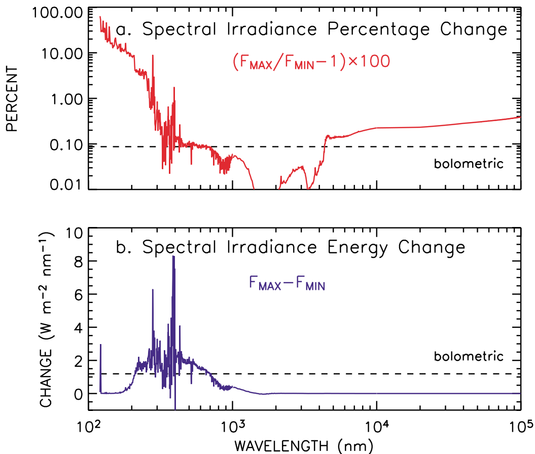
Fig. 14 The spectrum variations that cause the changes in total solar irradiance are shown in (a) as ratios of spectra at high and low solar activity, respectively ( F_{MAX} ) and ( F_{MIN} ), and in (b) as their difference in energy units. The changes for wavelengths longer than 400 nm are theoretical estimates (reproduced by permission of Fröhlich and Lean, 2004).
