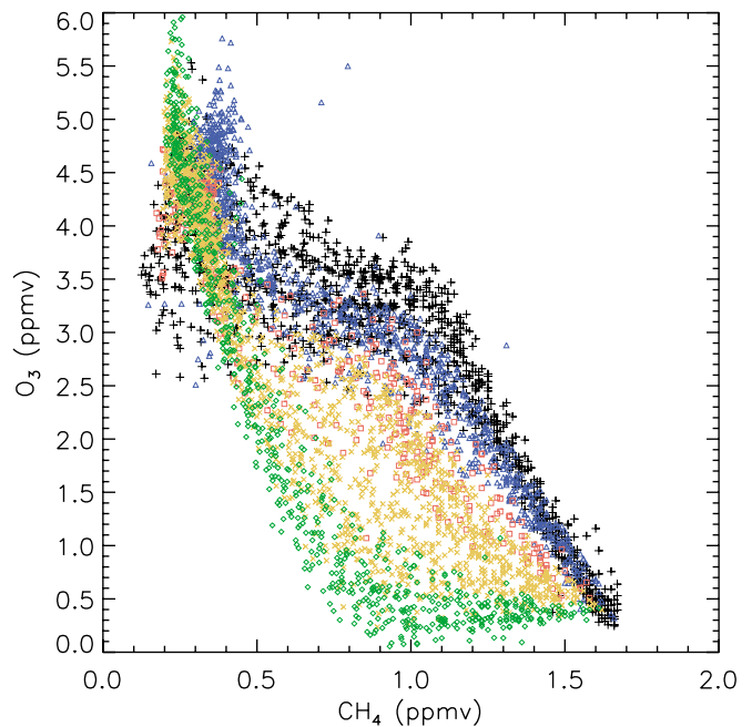
Fig. 12 O 3 /CH 4 correlation using ACE-FTS data from SCISAT-I for the same time period and locations as in Fig. 10 with the same colour scheme.
