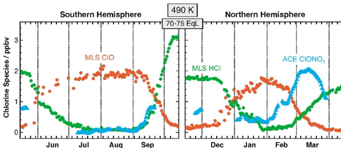
Fig. 6 (Left panel) Daily averages of ClO (red dots) and HCl (green dots) observed by Aura MLS, and ClONO 2 (cyan triangles) observed by ACE-FTS at 490 K (approximately 20 km) during the 2005 Antarctic winter/spring period, calculated over the 70° – 75° equivalent latitude band using the Global Modeling and Assimilation Office Goddard Earth Observing System (GEOS-4) temperatures and potential vorticity. Only daytime measurements are included in the averages for ClO; ClO data appear more sparse because measurements in sunlight are not always available at high equivalent latitudes, especially in early winter. The sampling pattern of ACE-FTS, a solar occultation instrument, does not provide coverage of this equivalent latitude band at all times throughout the winter. (Right panel) As in the left panel, for the 2004/2005 Arctic winter/spring period (reproduced by permission from WMO, 2007).
