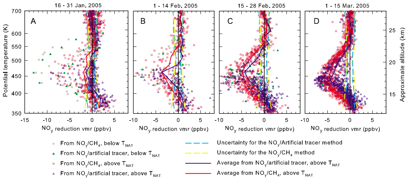
Fig. 7 \text{NO}_y reductions inside the polar vortex for the period 16 January 2005 – 15 March 2005. T_{\text{NAT}} is the threshold temperature for the formation of NAT. When the temperature is above T_{\text{NAT}} , it is assumed that \text{NO}_y is not temporarily sequestered (Jin et al. (2006b), reproduced by permission of the American Geophysical Union).
