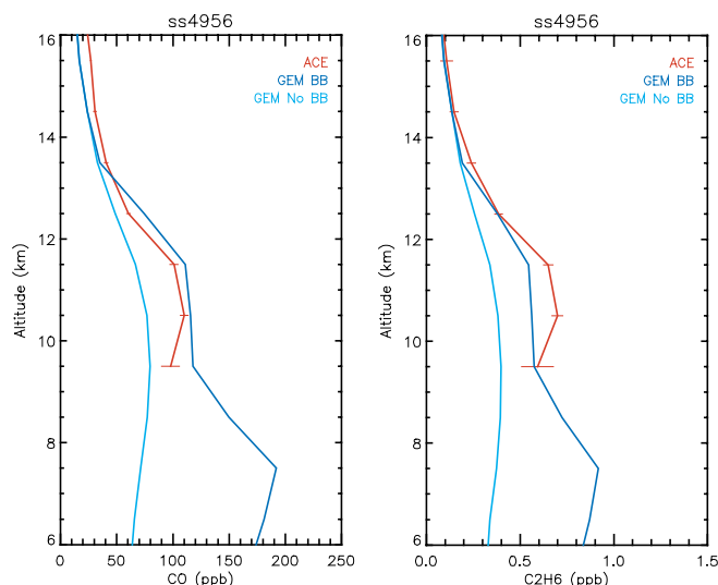
Fig. 19 A comparison of ACE-FTS profiles of CO and C_2H_6 from ACE (SCISAT-I) and the GEM-AQ modelling of boreal forest burning. The red curves are for the ACE data, while the cyan and blue curves are for GEM-AQ with seasonal and detailed burning emissions. The observation was made at 66^\circ N , 145^\circ W on 14 July 2004 (courtesy of Alex Lupu, York University).
