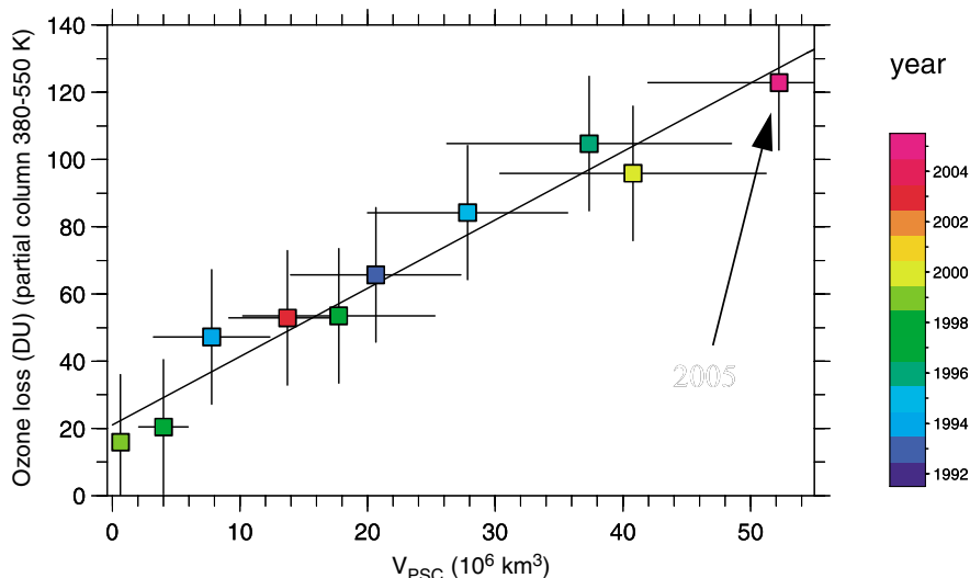
Fig. 13 O_3 loss versus V_{PSC} for Arctic winters between 1993 and 2005 (no values for the warm winters of 2001, 2002, 2004 due to major mid-winter warmings and/or lack of sufficient ozonesonde measurements). Value for 2005 is indicated. Values for other winters are from Rex et al. (2004), except all values are calculated between potential temperature levels of 380 K and 550 K. The line indicates a linear least squares fit to the points and has a slope of 15.6 \text{ DU K}^{-1} (Rex et al. (2006), reproduced by permission of the American Geophysical Union).
