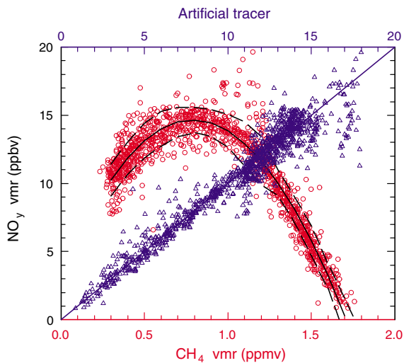
Fig. 8 Correlations of \text{NO}_y and \text{CH}_4 (red circles) and \text{NO}_y and an artificial tracer (blue triangles) between 350 K and 1000 K (approximately 12 – 35 km) for 1 – 15 January 2005. The black solid line is a third order polynomial fit for the \text{NO}_y/\text{CH}_4 correlation. The black dashed lines represent the 1- \sigma error range of the fit. The blue solid line represents a linear fit that has \text{NO}_y equal to the artificial tracer (Jin et al. (2006b), reproduced by permission of the American Geophysical Union).
