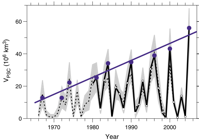
Fig. 21 V_{PSC} over the past 40 years from European Centre for Medium-range Forecasts (ECMWF) data (solid line) and FU-Berlin data (dashed line). See Rex et al. (2004) for a discussion of the FU-Berlin data. V_{PSC} has been calculated between 380 K and 550 K for all years. The grey shading represents the uncertainty of V_{PSC} due to a 1 K uncertainty in the long-term stability of radiosonde temperatures (Rex et al. (2006) reproduced by permission of the American Geophysical Union).
