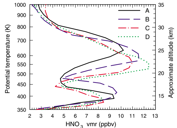
Fig. 9 Several typical \text{HNO}_3 profiles from ACE-FTS. A, at 63^\circ\text{N} , 96^\circ\text{W} on 13 January 2005; B, at 63^\circ\text{N} , 66^\circ\text{W} on 16 January 2005; C, at 65^\circ\text{N} , 80^\circ\text{W} on 22 January 2005; and D, at 65^\circ\text{N} , 63^\circ\text{W} on 23 January 2005 (Jin et al. (2006b), reproduced by permission of the American Geophysical Union).
