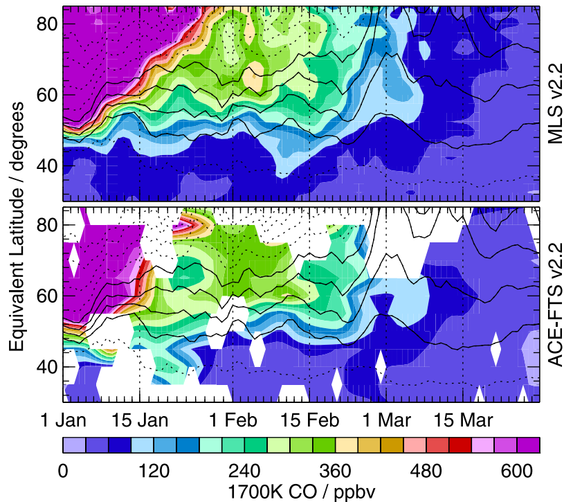
Figure 11. As in Figure 8 but for (top) MLS v2.2 and (bottom) ACE-FTS CO (ppbv) at 1700 K, using GEOS-4 DMPs.
