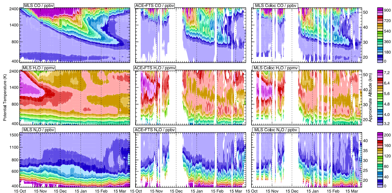
Figure 7. Vortex averages (within 1.4 \times 10^{-4} \text{ s}^{-1} sPV contour, see text, from GEOS-4 DMPs) for 3 October 2004 through 31 March 2005 of (top) CO (ppbv), (middle) H 2 O (ppmv), and (bottom) N 2 O (ppbv) from (left) MLS v1.5, (middle) ACE-FTS, and (right) MLS v1.5 measurements coincident with ACE (see text). Vertical range is 400 to 2500 K for CO and H 2 O, 400 to 1600 K for N 2 O.
