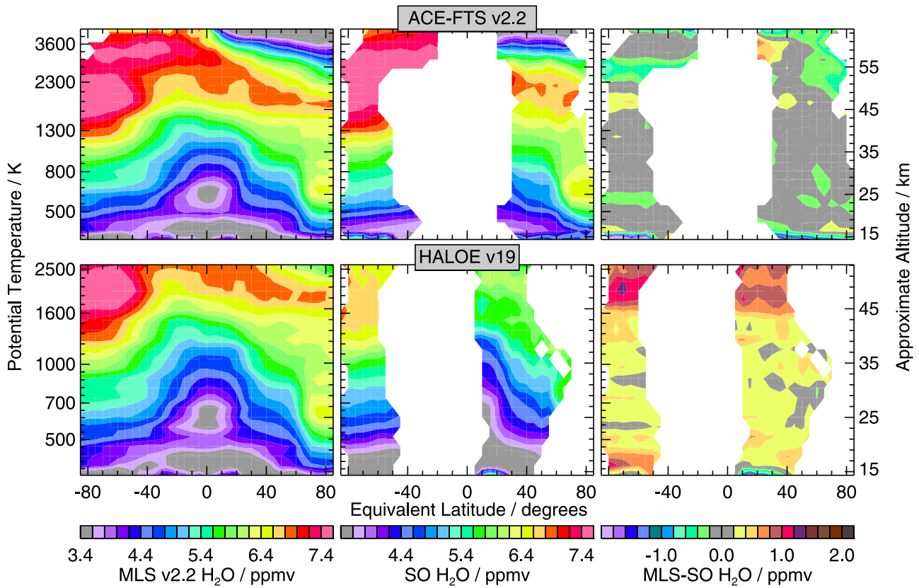
Figure 10. As in Figure 9 but for MLS v2.2 H 2 O (ppmv) compared with (top) ACE-FTS and (bottom) HALOE. GEOS-5 DMPs are used for ACE-FTS comparison and MetO for HALOE comparison. Vertical range for ACE-FTS comparison is 360–4300 K, for HALOE comparison, 360–2500 K.
