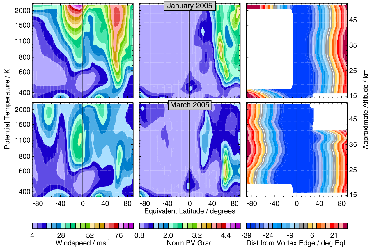
Figure 1. Monthly averages of equivalent latitude (EqL)/potential temperature ( \theta )-mapped (left) wind speed ( \text{m s}^{-1} ), (middle) normalized (see text) horizontal PV gradient, and (right) distance in EqL from the vortex edge center ( ^{\circ}\text{EqL} , see text). EqL/ \theta mapping is from derived meteorological products (DMPs) calculated from GEOS-4 data for MLS locations, during (top) January 2005 and (bottom) March 2005. White space in EqL from vortex edge plots indicates that the vortex is not defined anytime during the month in these regions.
