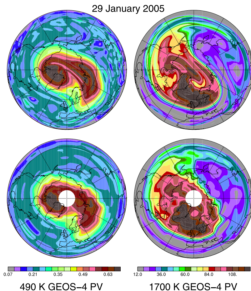
Figure 4. PV ( 10^{-4} \text{ K m}^2 \text{ kg}^{-1} \text{ s}^{-1} ) maps (top) from GEOS-4 analyses and (bottom) gridded (see text) from the MLS GEOS-4 DMP PV field, at (left) 490 K and (right) 1700 K. Projection is orthographic, with 0^\circ longitude at the bottom and 90^\circ\text{E} to the right; latitude range is from 0^\circ to 90^\circ\text{N} ; fine dashed lines show a 30^\circ latitude/longitude grid. White space above \sim 82^\circ\text{N} in Figure 4 (bottom) is region not sampled by MLS.
