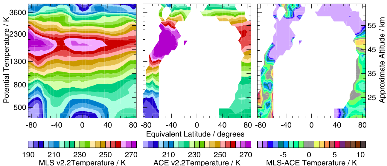
Figure 21. As in Figure 9 but for 17–24 September 2005 MLS v2.2 and ACE-FTS temperatures, using GEOS-5 DMPs. Vertical range is 360 to 4300 K.
