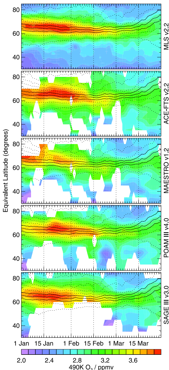
Figure 13. EqL/time series for 1 January through 31 March 2005 of O_3 (ppmv) at 490 K from (top to bottom) MLS (v2.2), ACE-FTS, MAESTRO, POAM III, and SAGE III. EqL mapping is done with MetO DMPs. Overlaid contours are MetO sPV ( 10^{-4} \text{ s}^{-1} ), with three contours in the vortex edge region shown as solid lines.
