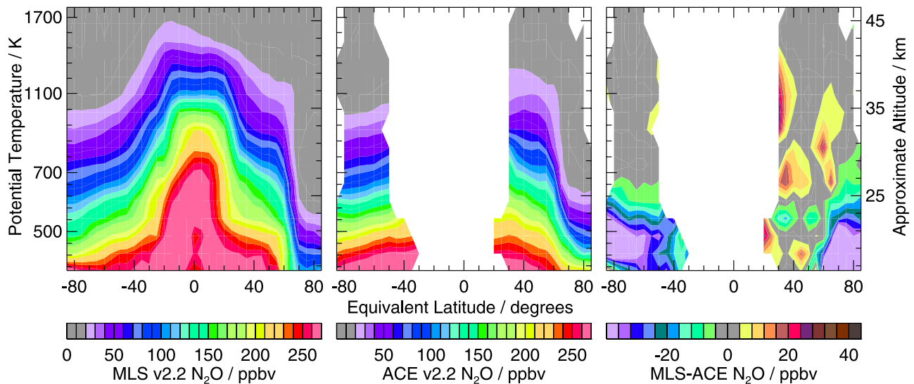
Figure 9. Global EqL/ \theta cross sections for 10–16 March 2005 comparing MLS v2.2 with ACE-FTS N 2 O. (left) MLS v2.2 N 2 O, (middle) ACE-FTS v2.2 N 2 O, and (right) the MLS-ACE-FTS N 2 O difference (ppbv). GEOS-5 DMPs are used for EqL/ \theta mapping. Vertical range is 400 through 1800 K.
