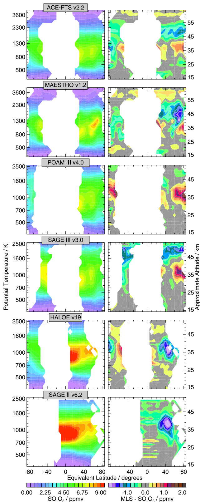
Figure 16. Global EqL/ \theta cross sections for 10–16 March 2005 comparing MLS v2.2 \text{O}_3 with (top to bottom) ACE-FTS, MAESTRO, POAM III, SAGE III, HALOE, and SAGE II. (left) Solar occultation instruments' \text{O}_3 and (right) the MLS-solar occultation instrument \text{O}_3 difference (ppmv). For comparisons with ACE-FTS and MAESTRO, GEOS-5 DMPs are used for EqL/ \theta mapping; others comparisons use MetO DMPs. MLS/ACE comparisons are shown from 360 through 4430 K; others are 360 through 2500 K (the top limit of the MetO DMPs).
