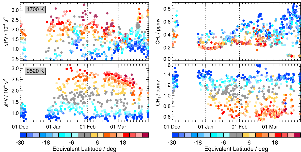
Figure 2. Time series of distance in EqL from vortex edge center (colors, ^{\circ}\text{EqL} ) as a function of (left) sPV ( 10^{-4} \text{ s}^{-1} ) and (right) ACE-FTS \text{CH}_4 (ppmv) at (top) 1700 K and (bottom) 520 K, for ACE measurement locations during December 2004 through March 2005. Vortex edge location values are from GEOS-4 DMPs.
