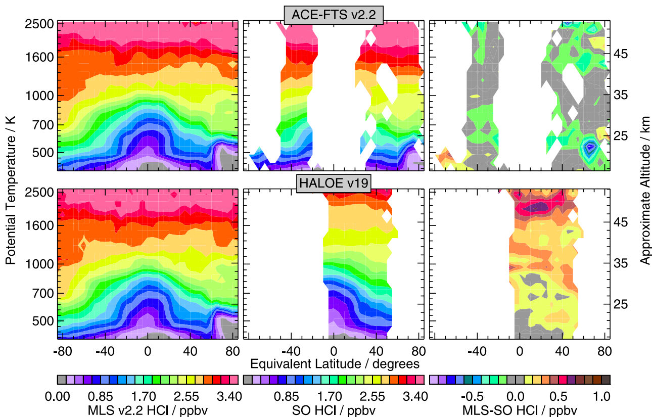
Figure 20. As in Figure 9 but for MLS v2.2, ACE-FTS, and HALOE HCl (ppbv) for 25–31 January 2005. ACE-FTS comparison uses GEOS-5 DMPs, HALOE comparison uses MetO DMPs. Vertical range is 400–2500 K.
