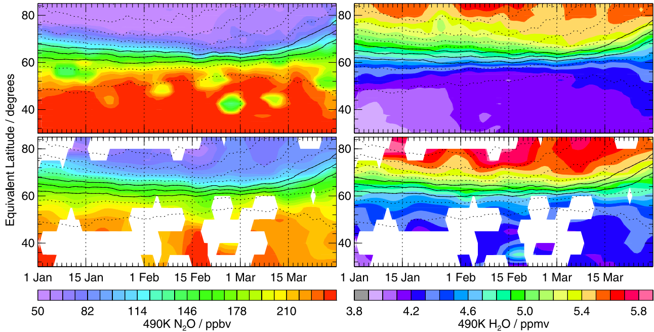
Figure 8. EqL/time series for 1 January through 31 March 2005 of (top) MLS v2.2 and (bottom) ACE-FTS (left) N 2 O (ppbv) and (right) H 2 O (ppmv) at 490 K, using GEOS-4 DMPs.
