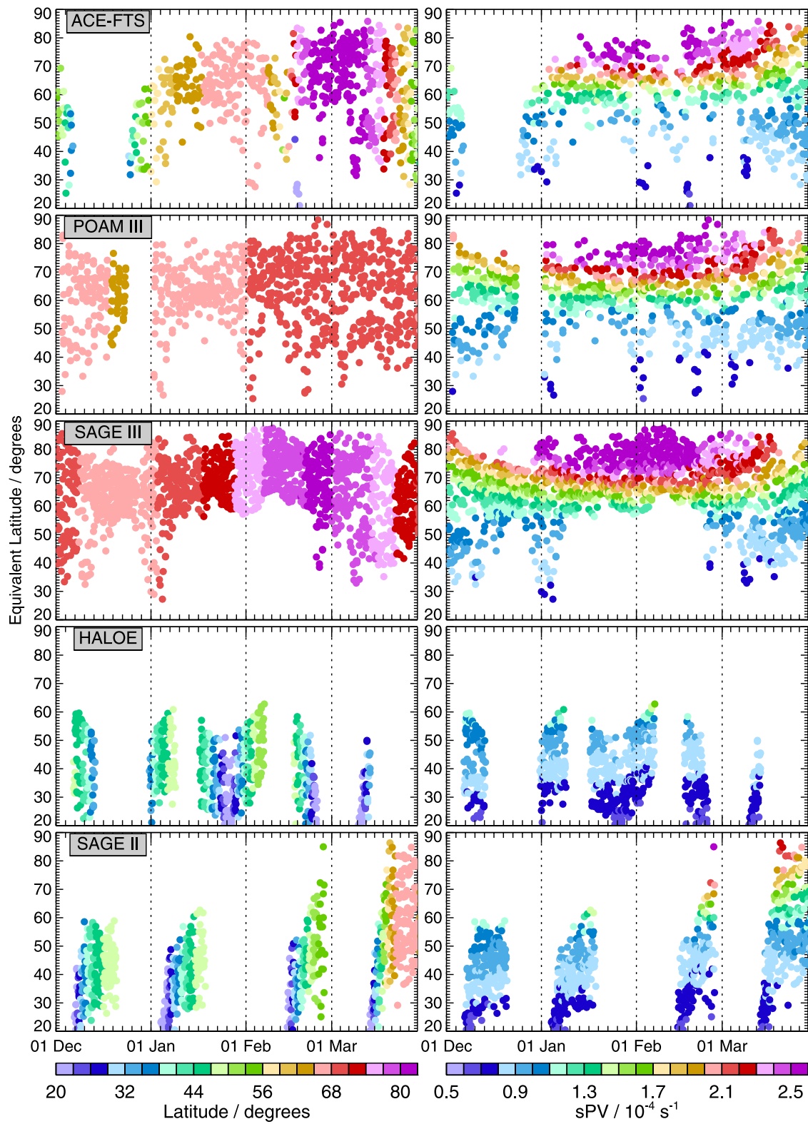
Figure 5. EqL/time plots of (left) latitude ( ^{\circ} ) and (right) sPV ( 10^{-4} \text{ s}^{-1} ) sampled by (top to bottom) ACE, POAM III, SAGE III, HALOE, and SAGE II during December 2004 through March 2005 EqL on the 490 K isentropic surface.
