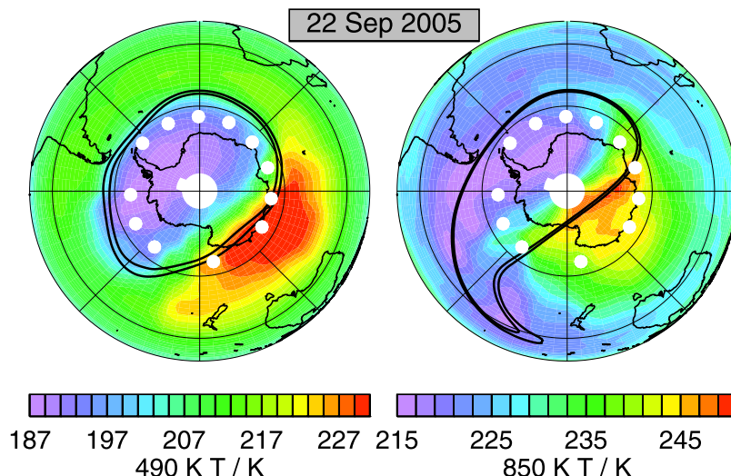
Figure 22. Maps of MLS v2.2 Temperature (colors, K) on 22 September 2005 at (left) 490 K and (right) 850 K. Overlaid contours are 1.4 and 1.8 \times 10^{-4} \text{ s}^{-1} sPV. White dots show ACE observation locations.
