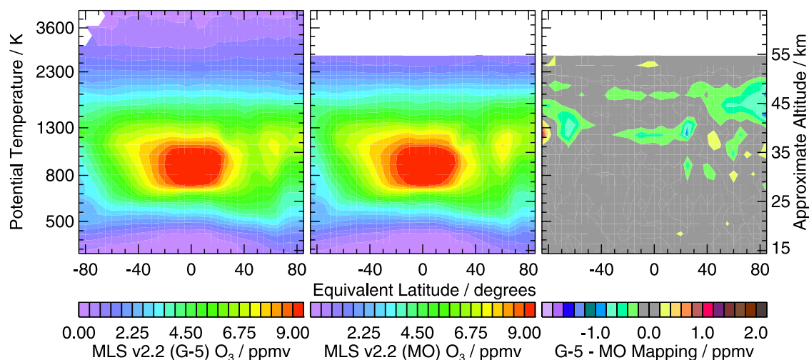
Figure 15. Global EqL/ \theta cross sections for 10–16 March 2005 comparing MLS v2.2 O 3 (ppmv) mapped using (left) GEOS-5 and (middle) MetO DMPs and (right) the difference (ppmv). Vertical range is 360 through 4300 K.
