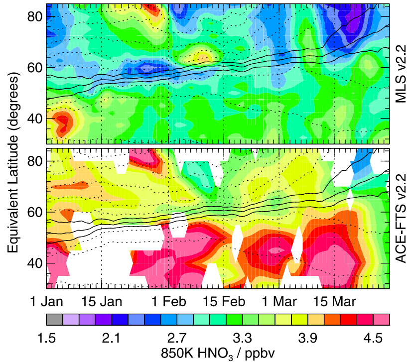
Figure 17. As in Figure 13 but for (top) MLS v2.2 and (bottom) ACE-FTS \text{HNO}_3 (ppbv) at 850 K, using GEOS-4 DMPs.
