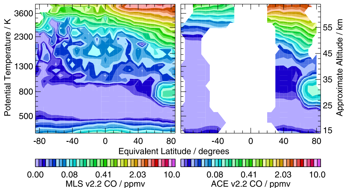
Figure 12. As in Figure 9 (with difference panel omitted) but for MLS v2.2 CO (ppbv) compared with ACE-FTS, using GEOS-5 DMPs. Vertical range is 360–4300 K. CO contour interval is on a log scale, from 20 to 10,000 ppbv.
