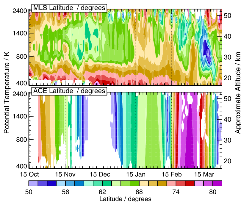
Figure 6. Vortex-averaged (within the 1.4 \times 10^{-4} \text{ s}^{-1} sPV contour, see text, from GEOS-4 DMPs) latitude ( ^{\circ} ) sampled by (top) MLS and (bottom) ACE from 15 October 2004 through 31 March 2005.
