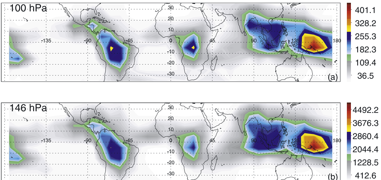
Figure 3. (a) Geographical distribution of total accumulation of ice water content in 10^\circ \times 10^\circ boxes at 100 hPa from 2005 AURA MLS data. Units are \text{mg}/\text{m}^3 . (b) Same as Figure 3a but for 146 hPa.
