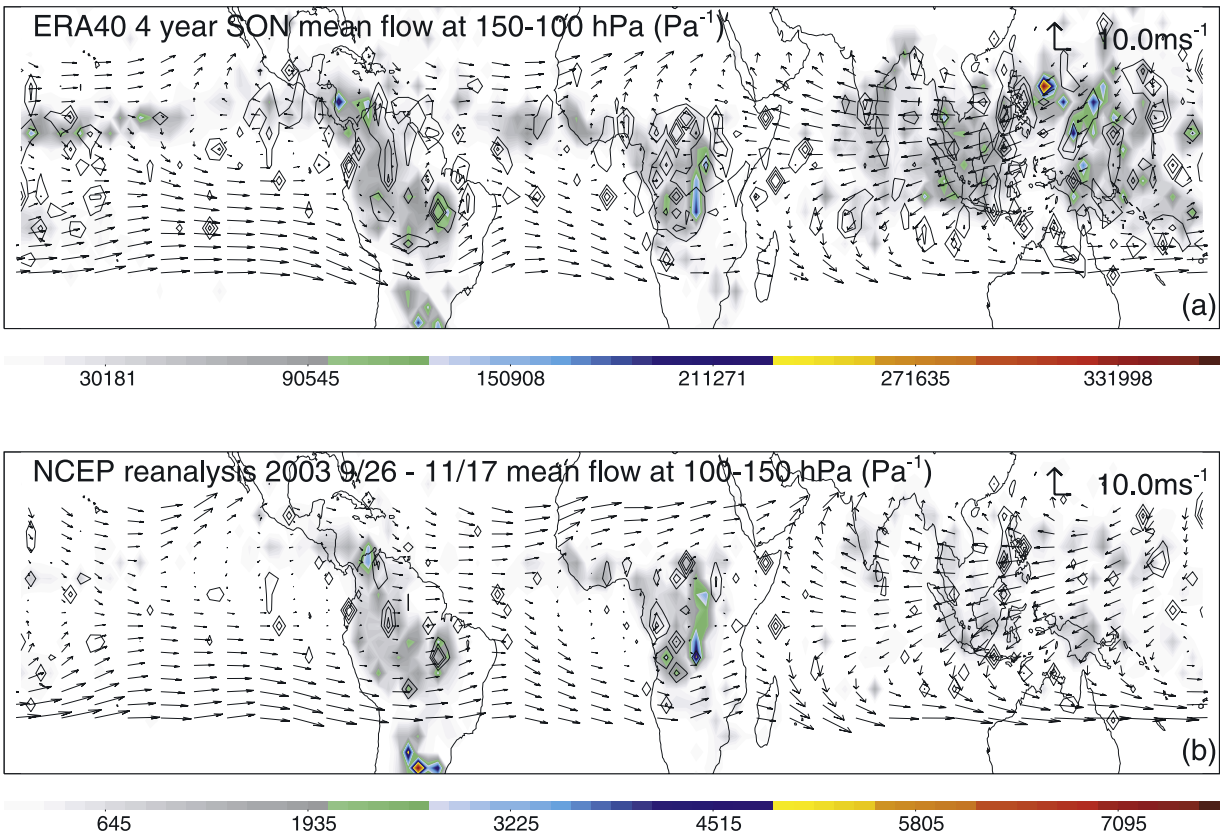
Figure 7. (a) Accumulative TRMM VIRS area of T_{B11} < 210 K in 3^\circ \times 3^\circ boxes (color fill) and total coverage of GCFs above 14 km with size above 100 km in the same box (contoured with 300, 600, and 900 km). ERA40 4 year (1998–2001) September, October, and November mean flow between 100 and 150 hPa are overlapped. (b) Accumulative area of TRMM PR 20 dBZ reaching 14 km in 3^\circ \times 3^\circ boxes (color fill) and total coverage of GCFs thicker than 1 km above 14 km in the same box (contoured with 300, 600, and 900 km). NCEP reanalysis 26 September to 17 November mean flow between 100 and 150 hPa are overlapped.
