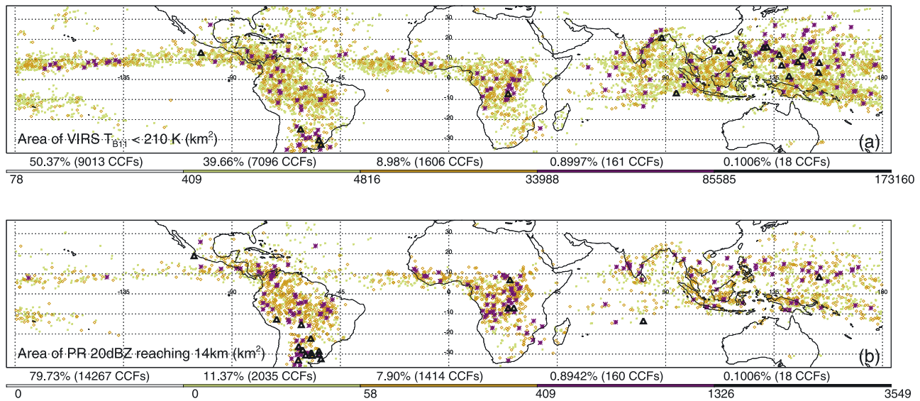
Figure 6. Location of September–November 2003 TRMM CCFs ( \leq 210 K) categorized by (a) size of T_B \leq 210 K and (b) size of 20 dBZ reaching 14 km. Rarity of the events is represented with green dots (approximately top 10%), orange diamonds (approximately top 1%), purple asterisks (approximately top 0.1%), and black triangles (approximately top 0.01%).
