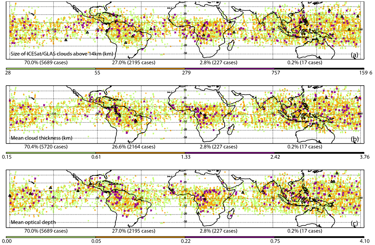
Figure 5. Locations of GCFs above 14 km categorized by (a) size, (b) mean thickness, and (c) mean optical depth. Rarity of the events is represented by green dots (approximately bottom 80%), orange diamonds (approximately top 20%), purple asterisks (approximately top 2%), and black triangles (approximately top 0.2%).
