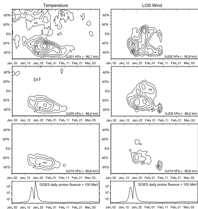
Figure 1. (top) The 2005 latitude-time evolution of the two-day wave amplitude in temperature (every 2 K) and line-of-sight (LOS) wind (every 5 m/s). The LOS wind is computed from profiles along the ascending tracks (see Section 2). (bottom) Concurrent values of NOAA GOES daily proton fluence (in Protons/cm 2 -day-sr).
