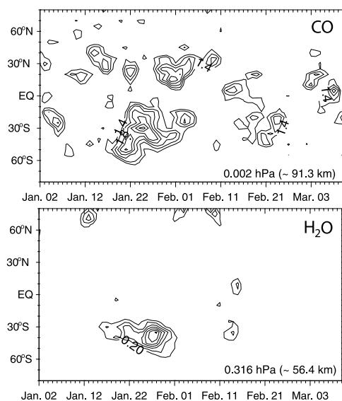
Figure 3. The 2005 latitude-time evolution of the two-day wave amplitude in carbon monoxide (top; every 0.5 ppmv) and water vapor (bottom; every 0.2 ppmv).
