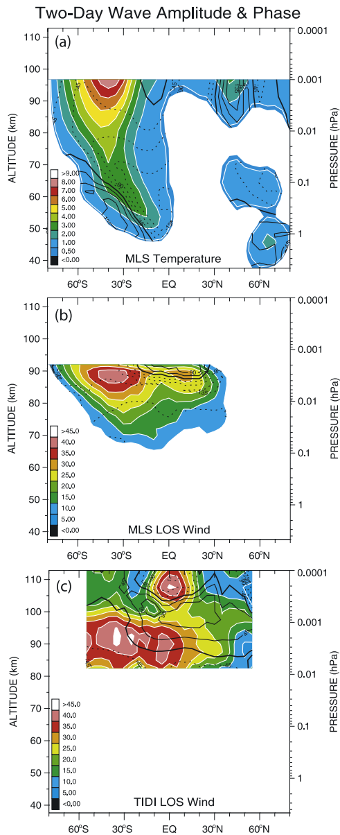
Figure 2. January 24–27 meridional structure of the two-day wave amplitude (filled contours) for (a) temperature in K and (b) LOS wind in m/s from ascending MLS data, and (c) ascending cold side TIDI profiles in m/s. Phase lines (every 45^\circ ) are in black.
