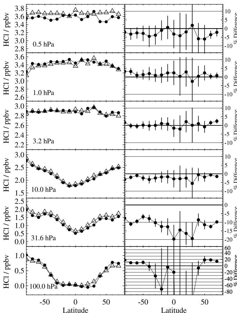
Figure 13. Similar to Figure 10 but for v2.2 MLS and ACE-FTS HCl comparisons including matched profiles from 2004, 2005, and 2006.
