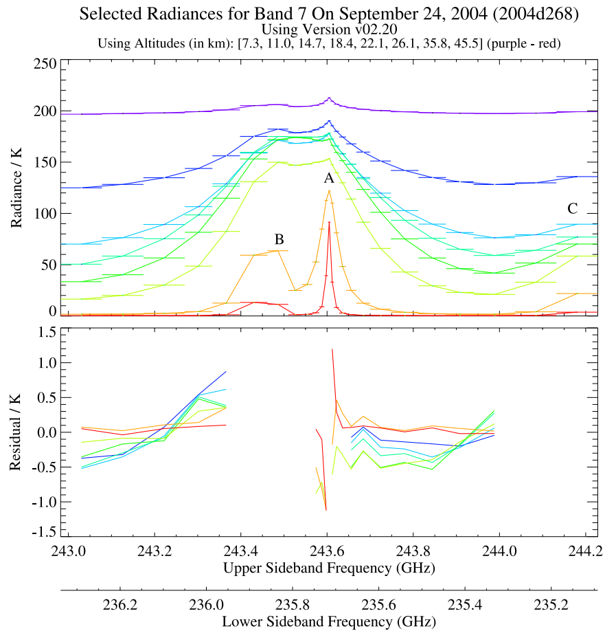
Figure 1. (top) MLS daily average radiances for the “band 7” spectral region near 240 GHz, relevant to the retrievals of the MLS standard O_3 product. The width of the channel filters is indicated by horizontal lines. The primary ozone emission line occurs in the lower sideband and is seen near the center of the plot (label A), with weaker ozone lines (from the upper sideband, folded over in this plot) to the left of it (label B), and wing emission from another line to the right (label C). These radiances are for 24 September 2004 for average tangent heights of 7 km (purple) to 45 km (red), as indicated above the plot. The x axes provide the frequencies in the upper and lower sidebands, which both contribute to the total radiances measured by MLS. (bottom) Residuals (average calculated minus observed radiances) corresponding to each colored curve from Figure 1 (top). Channels that are not shown here are not used in the retrievals, except for the very center of the main line, which is covered by fine-resolution digital autocorrelator spectrometer (DACs) channels for the mesosphere. Also, optical depth cut-off criteria “turn off” certain channels (near-line center) at the lower altitude levels.
