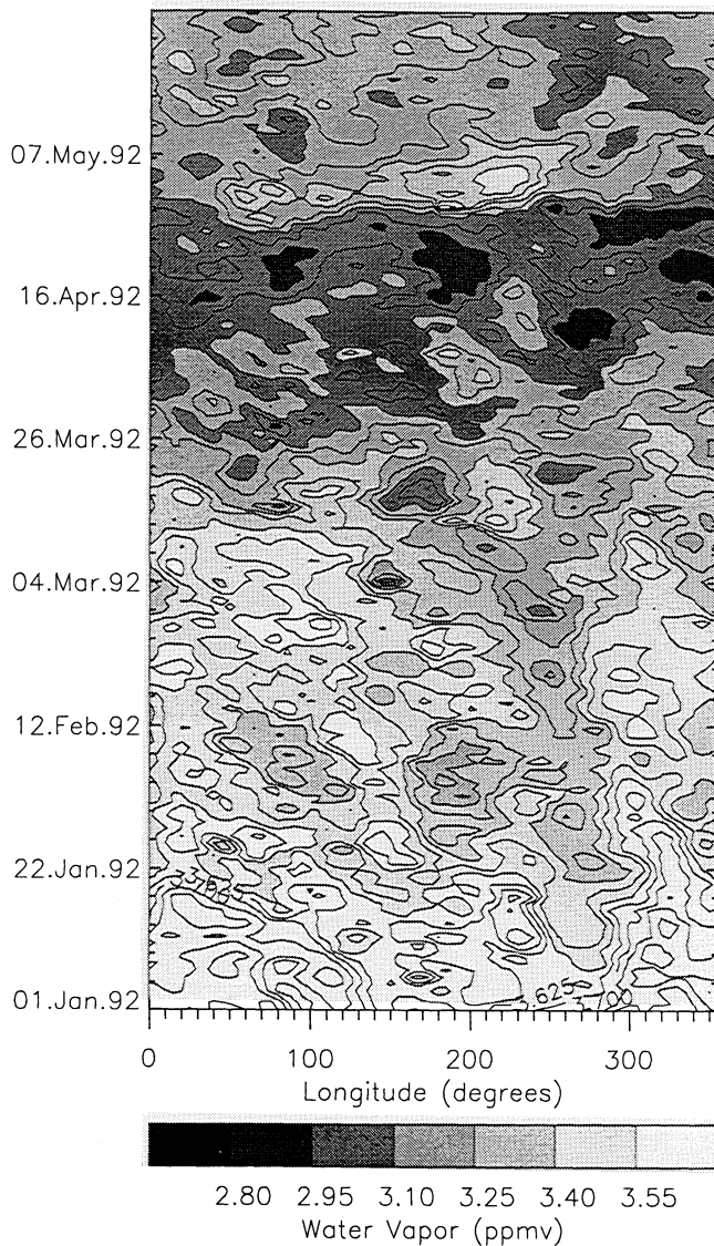
Figure 1. Longitude-time section at 10^{\circ}\text{N} showing the driest phase of Northern Hemisphere winter 1992. The contour interval is 0.075 ppmv, and the shading corresponds to that in Figure 2.
