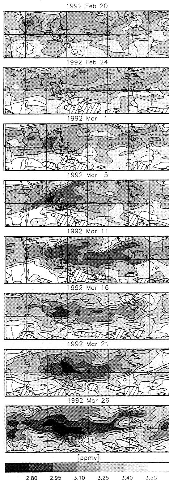
Figure 4. Ten-day advection of MLS water vapor (ppmv) for 1992 on the 435 K isentropic surface using UKMO winds.
