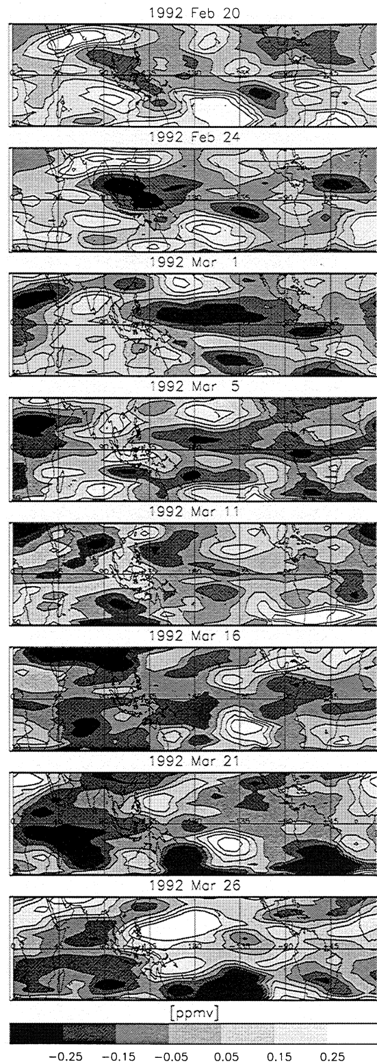
Figure 3. Difference between the MLS water vapor field (ppmv) and that of 10 days earlier. This figure therefore illustrates the change in the observed field over 10 days.
