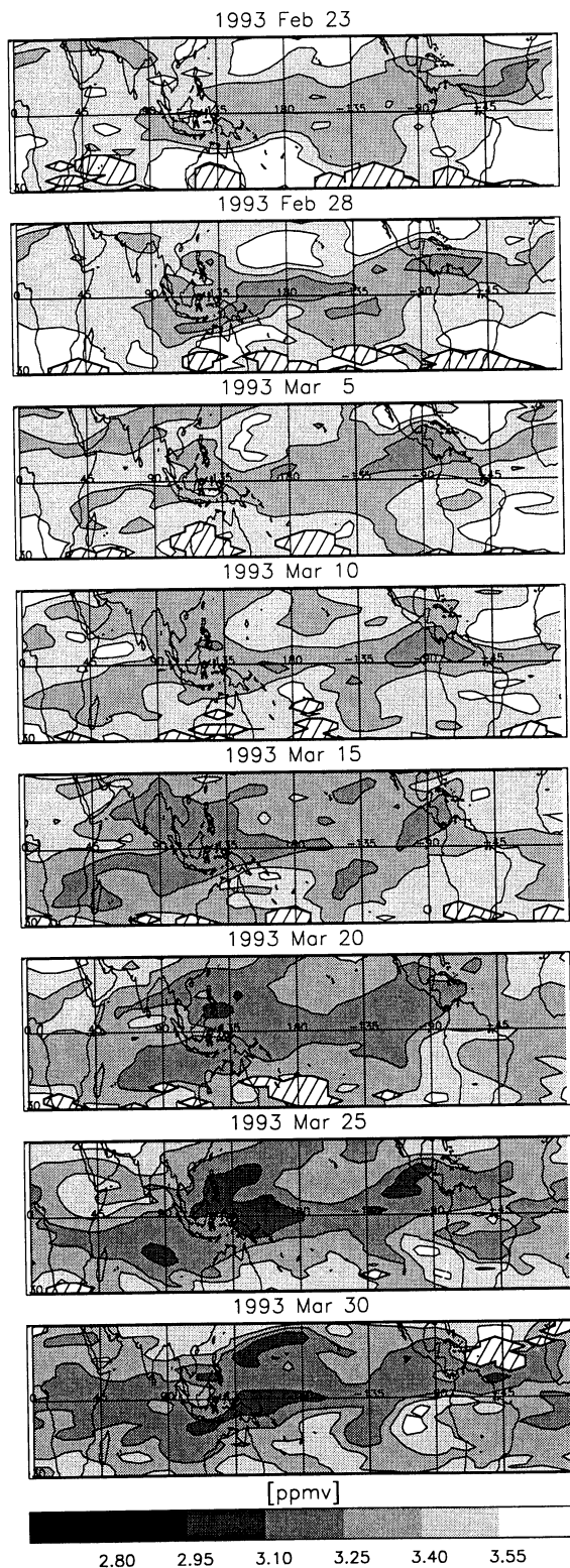
Figure 8. Ten-day advection of MLS water vapor (ppmv) for 1993 on the 435 K isentropic surface using UKMO winds.
