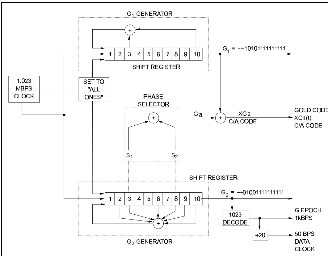
Figure 2-4. C/A-Code Generation
