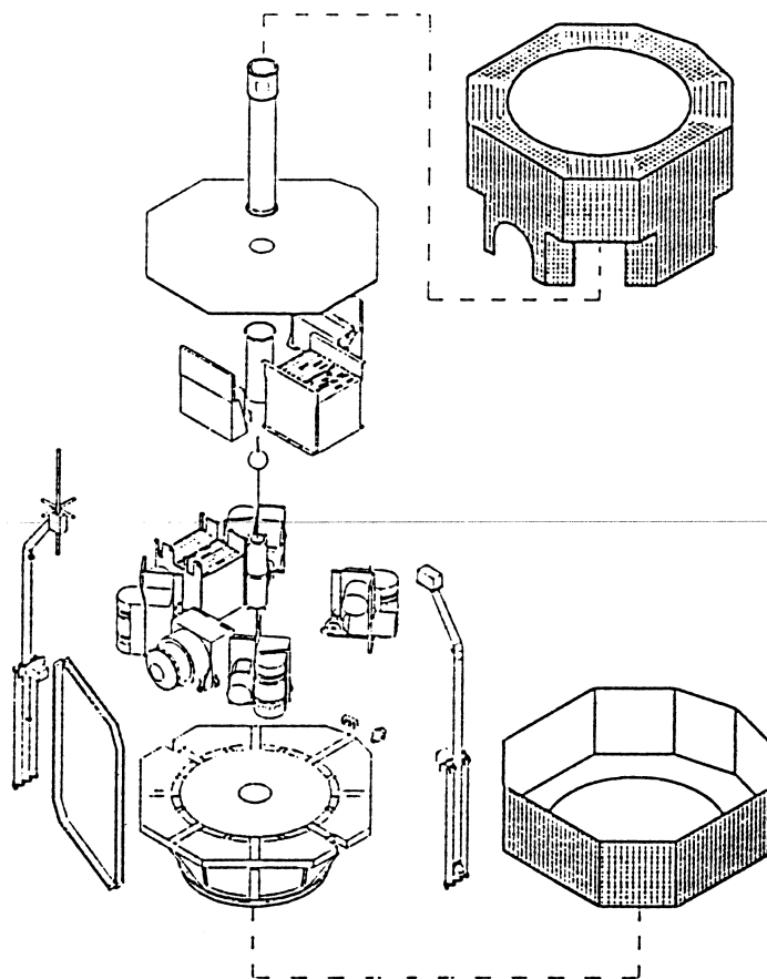
Figure 1: FAST Spacecraft
