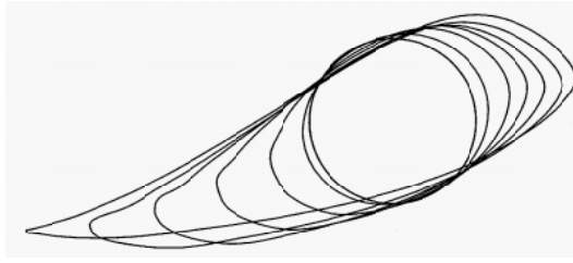
Figure 3.8 ERS-100 Blade Root Sections
