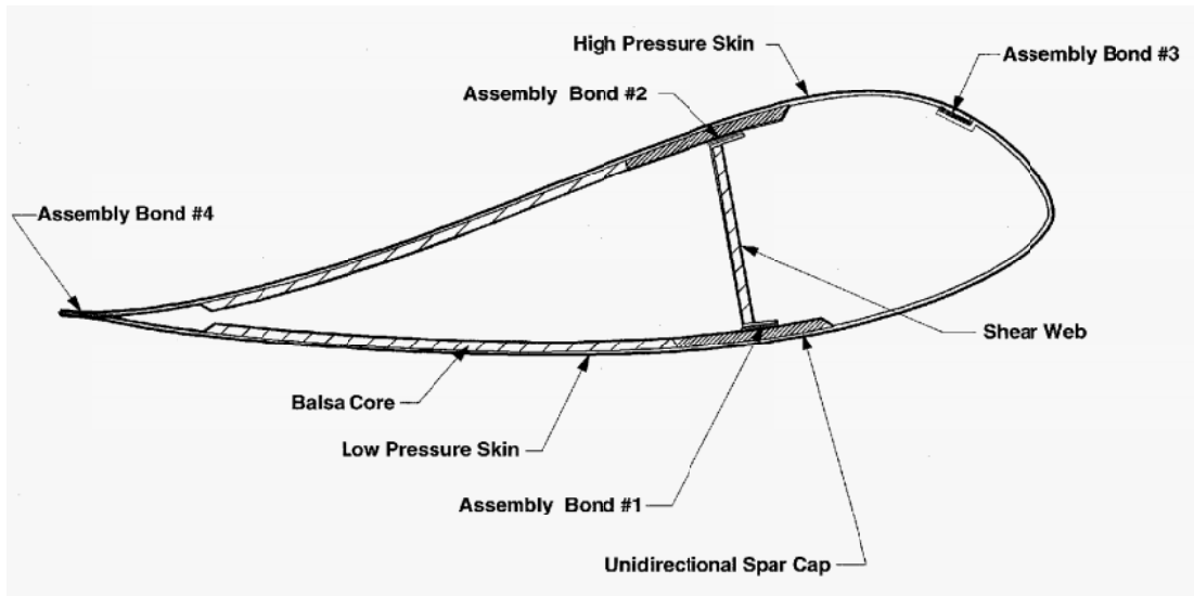
Figure 3.6 Typical ERS-100 Blade Cross-Section
