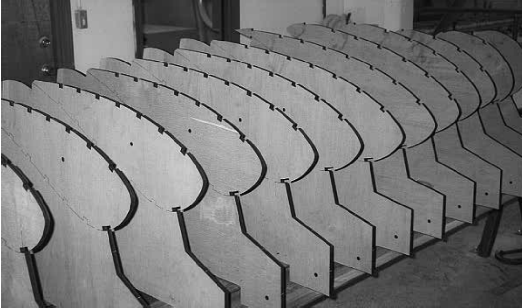
Figure 3.11 Photograph of ERS-100 Blade Pattern Templates
