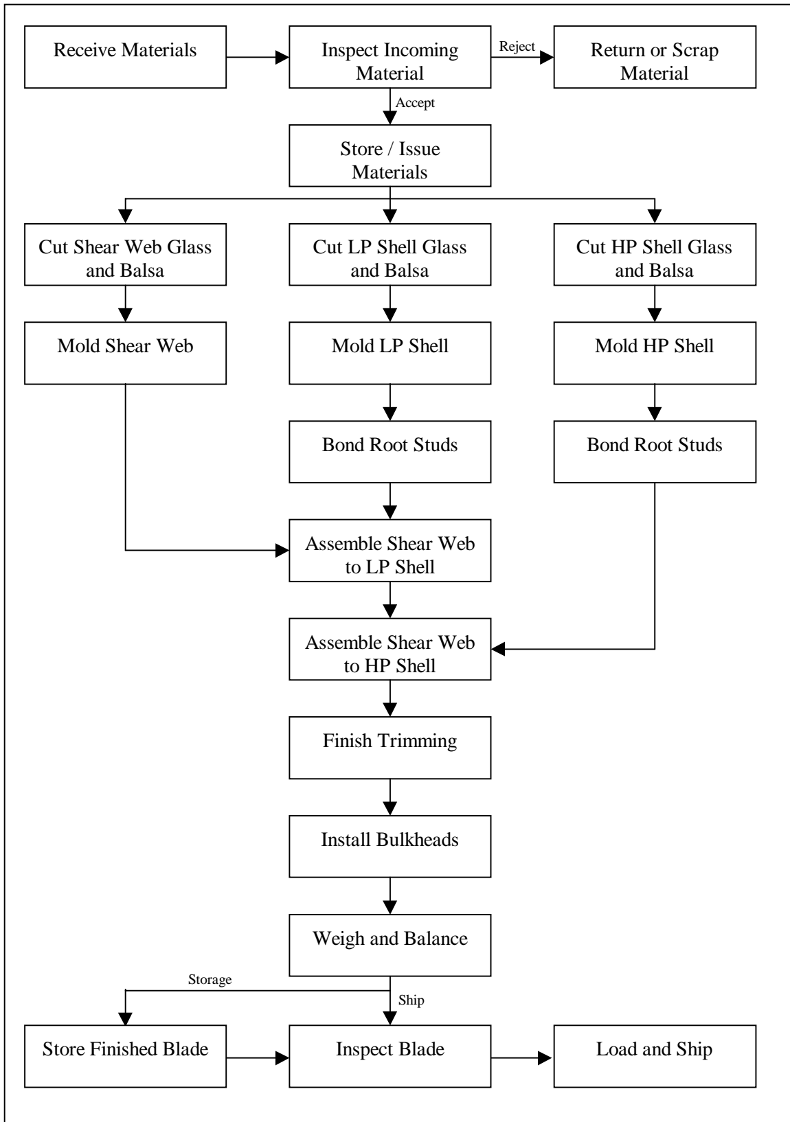
Figure 3.12 Schematic of the ERS-100 Manufacturing Process
