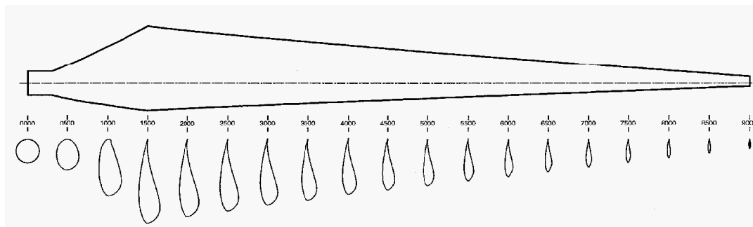
Figure 3.7 ERS-100 Blade Planform and Airfoil Sections
