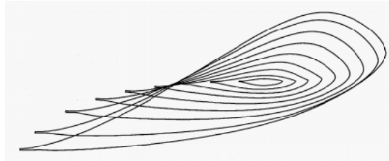
Figure 3.9 ERS-100 Blade Outboard Sections
