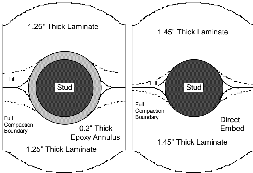
Figure 4.1 Stud Test Specimen Cross Sections
