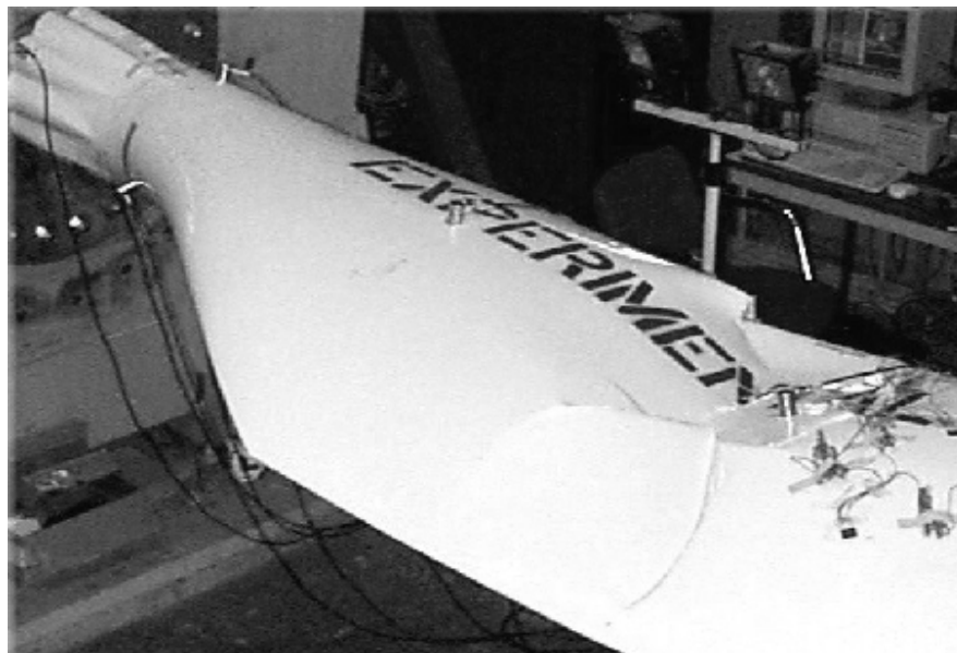
Figure 4.6 Photograph of the ERS-100 Blade After Static Failure
