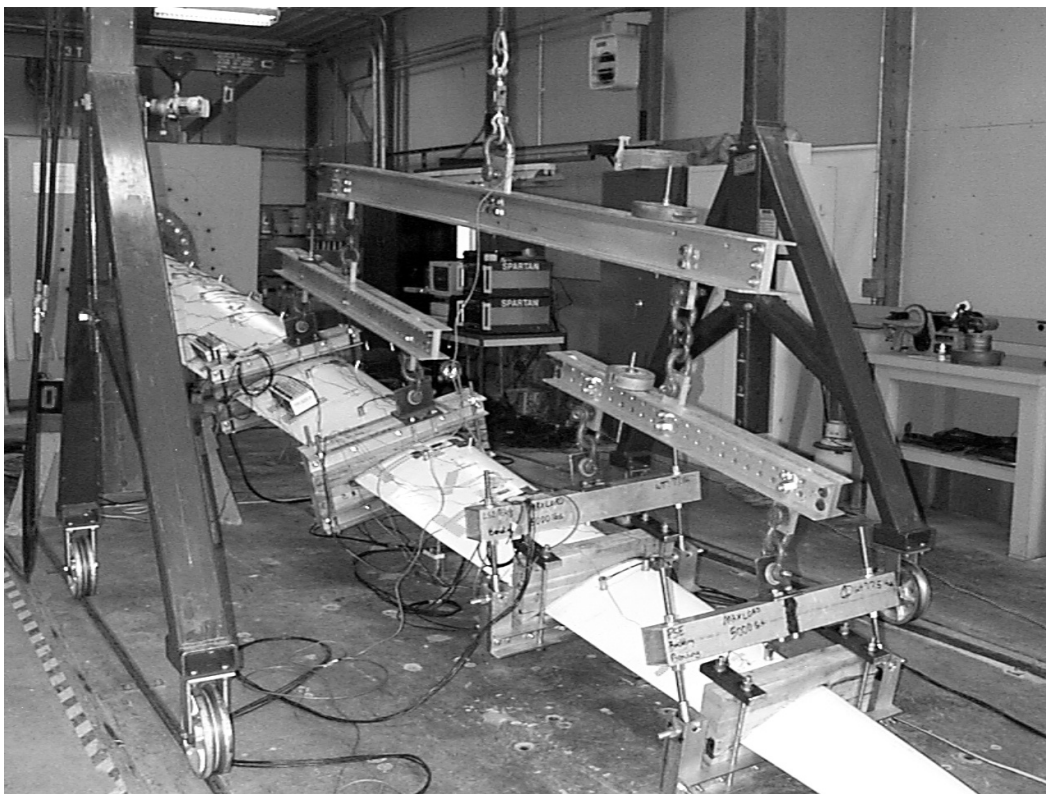
Figure 4.4 Photograph of the ERS-100 Blade in the Test Stand
