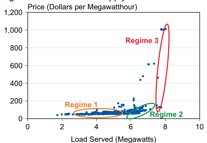
Figure 4.2. NYISO Zonal Supply Curve
