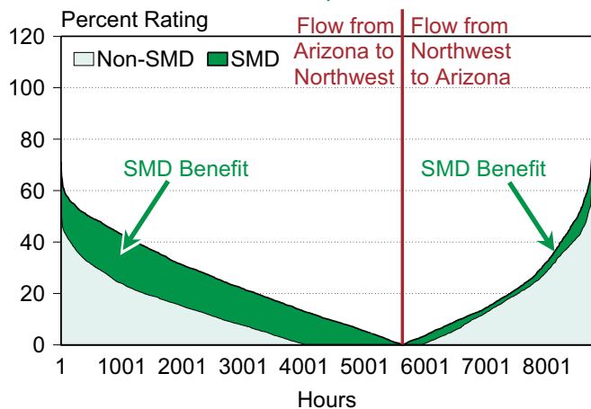
Figure 3.26. Power Flows Across the Arizona-Northwest Interface, 2005
