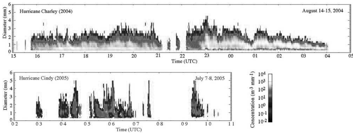
Hurricane Cindy (2005) was observed after it became an extratropical cyclone indicated by larger raindrops that are decreasing in abundance of raindrops as the hours pass when compared to smaller raindrops in greater abundance during Hurricane Charley (2004). Credit: Ali Tokay/NASA.
