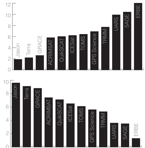
Figure 1: (top) Relative rank of each mission, with 1 being the highest and 12 the lowest. Figure 2: (bottom) Rank based on absolute scientific value (10-8 compelling; 7-4 excellent but less compelling, and 3-0 modest)
