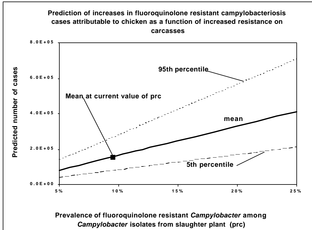
Figure 5.6. Using the risk assessment model to predict changes in I_{3r} , on the vertical axis, due to increases in p_{rc} , on the horizontal axis.
