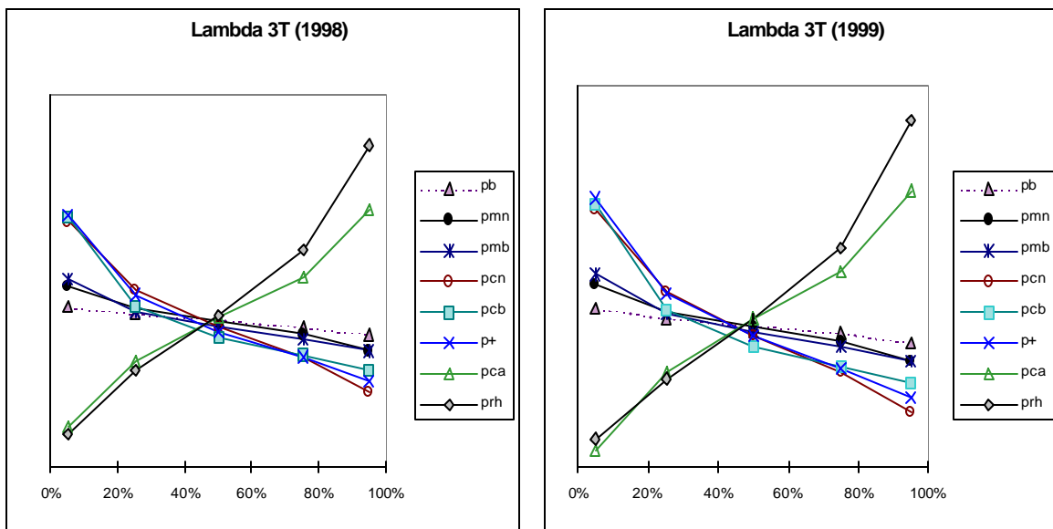
Figure 5.7. The parameters that contribute the most to the uncertainty in the value for \lambda_{3T} .
