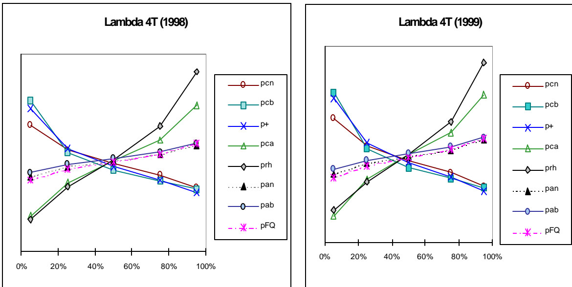
Figure 5.8. The parameters that contribute the most to the uncertainty in the value for \lambda_T .
