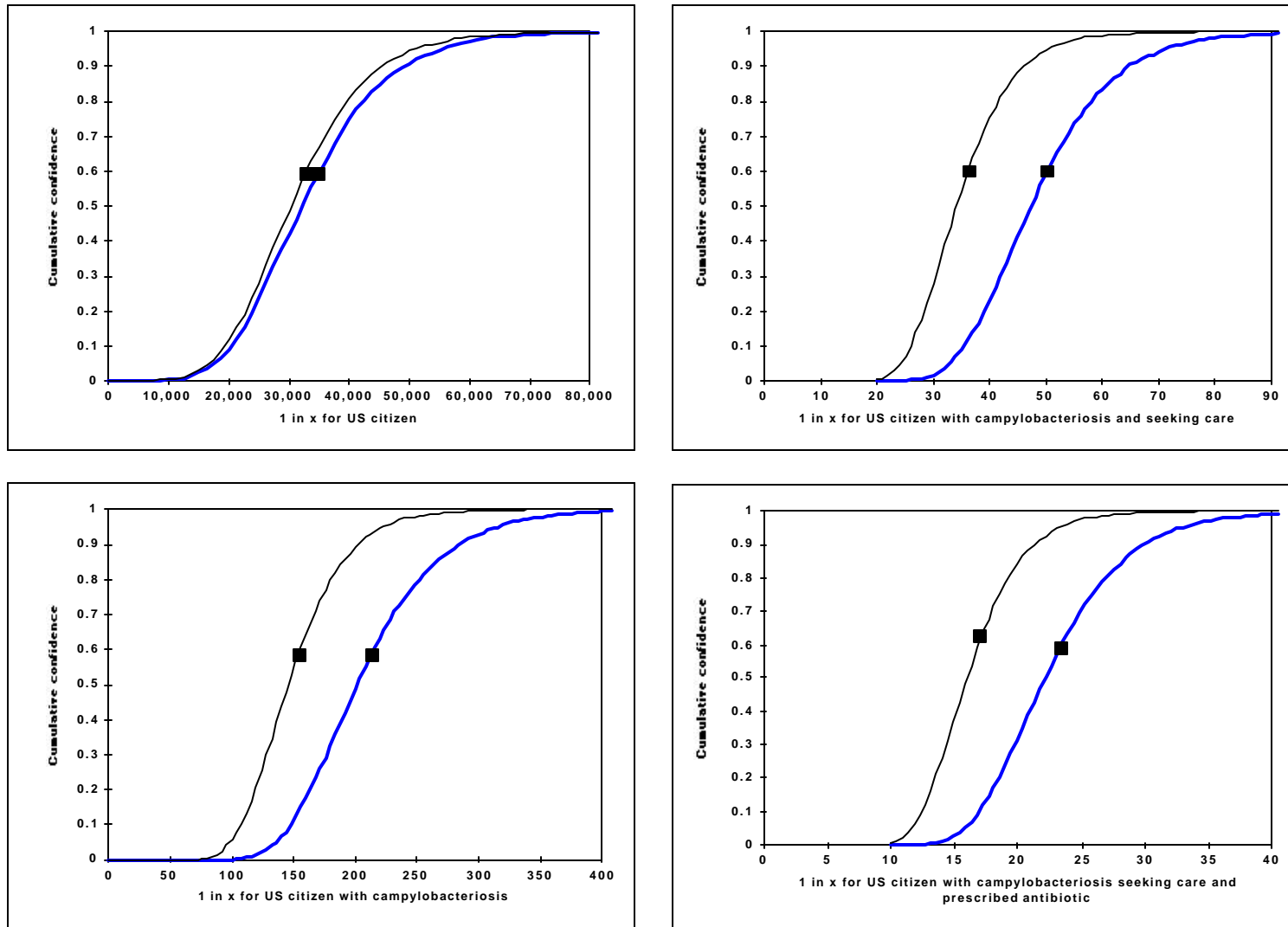
Figure 5.1b Confidence distributions for 1998 (heavier lines) and 1999 (lighter lines) values for the probabilities described in this section (in 1 in x format) for the four different denominators representing different populations at risk – black squares denote expected value
