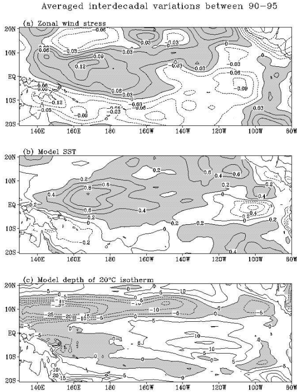
Figure 2: Same as Fig. 1, except for interdecadal modes instead of interannual anomalies. The interdecadal mode is defined as the variation with period longer than 8 years and was derived from the 36-year simulation through Fourier decomposition.
