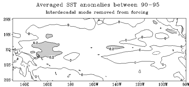
Figure 6: Average (1990-1995) of model-simulated sea surface temperature anomalies when forced by zonal wind stress and atmospheric humidity with decadal mode removed.
