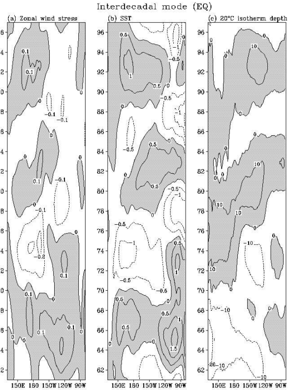
Figure 3: Longitudinal and temporal variations of decadal modes of (a) zonal wind stress, (b) sea surface temperature, and (c) depth of 20°C isotherm along the equator.
