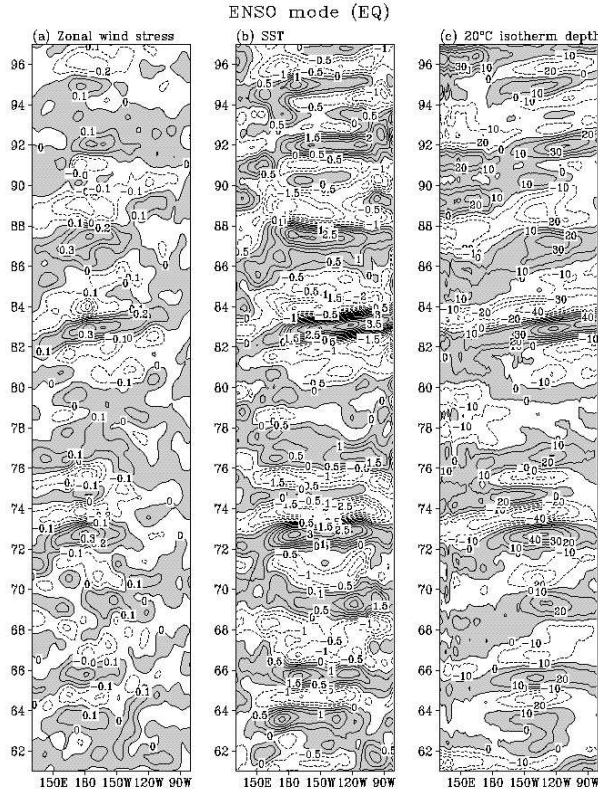
Figure 4: Same as Fig. 3, except for ENSO mode instead of decadal mode. The ENSO mode is defined as the variation with period between 2 to 7 years and was derived with the same method as the interdecadal mode.
