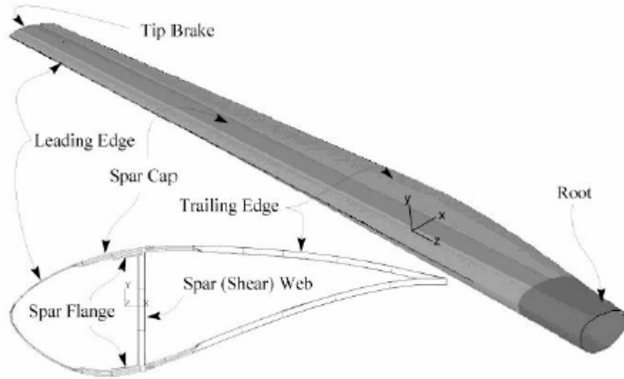
Figure 6: Blade construction [14].
