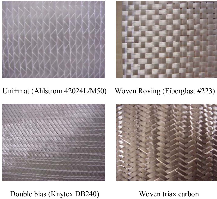
Figure 21: Fabrics tested for permeability.
