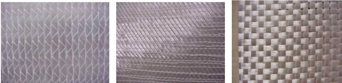
Figure 3: Unidirectional, double bias, and woven roving fabrics.
