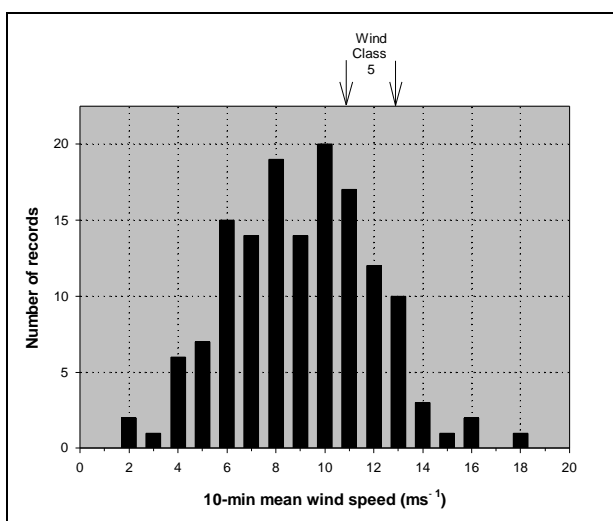
Figure 1. Simulated diurnal 10-minute mean wind speed distributions.
