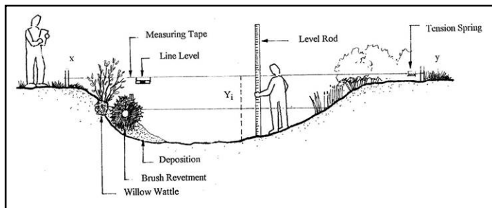
Measuring a stream cross section
