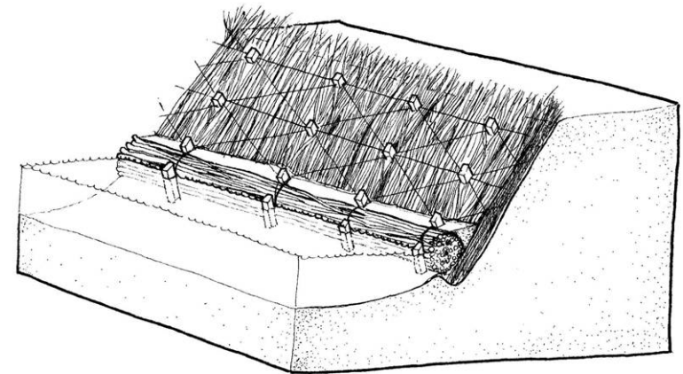
Brush mattress with a fascine toe
