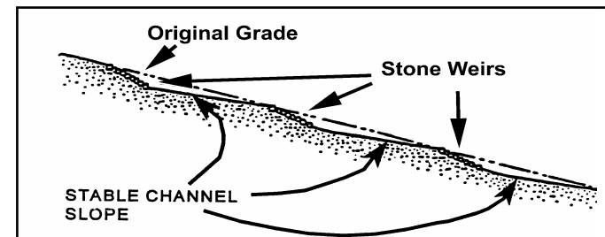
Channel stabilized with a series of low head stone weirs *
