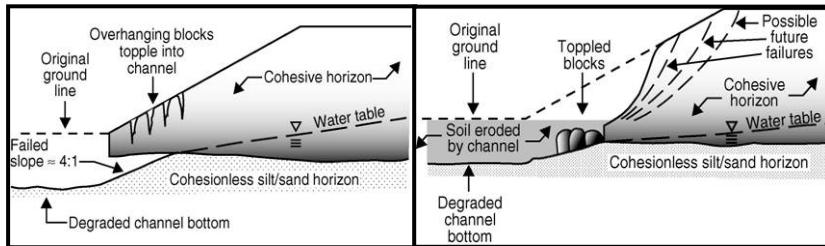
Development of piping/sapping bank failure
