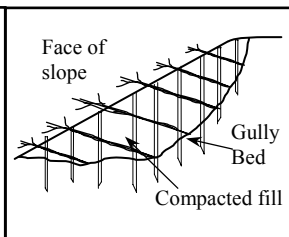
Brush Packing in gully: Cross Section
