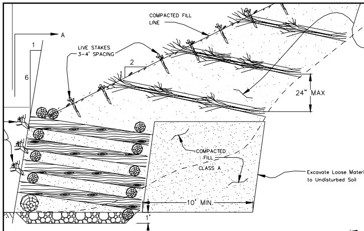
Cross Section of a vegetated crib wall. Note that in this case, brush layering and live staking treatments are specified above the structure.
