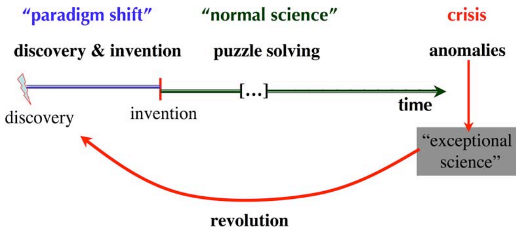
Figure 1: A schematic representation of Kuhn’s account of the advent, development, and dissolution of scientific fields. The scheme and nomenclature are from [1].
