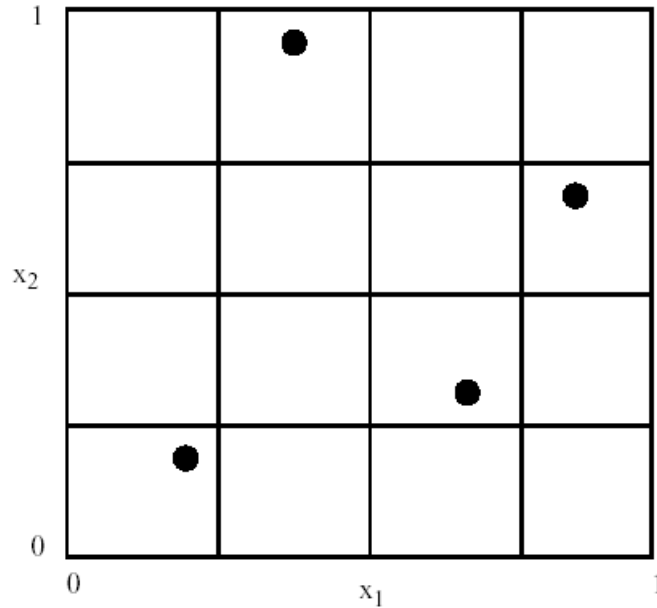
Figure 6.1: An example of Latin hypercube sampling with four bins in design parameters x_1 and x_2 . The dots are the sample sites.
