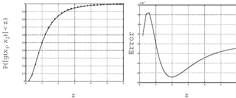
Figure 6.10: Comparison of the cumulative distribution function (CDF) computed by FORM (+ marks) and the exact CDF for g(x_1, x_2) = \frac{x_1}{x_2}
