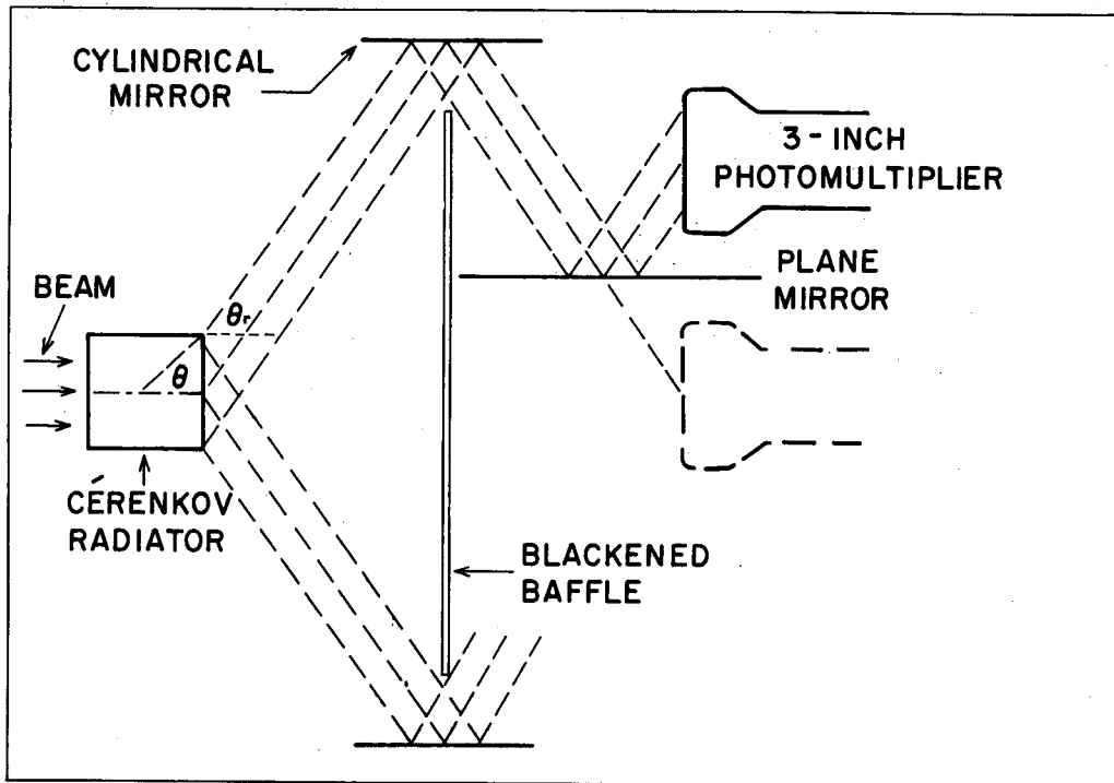
VELOCITY-SELECTING CÉRENKOV COUNTER (C 2)
