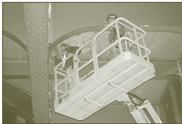
Part of an In-Depth Inspection task at a STAR bridge.
