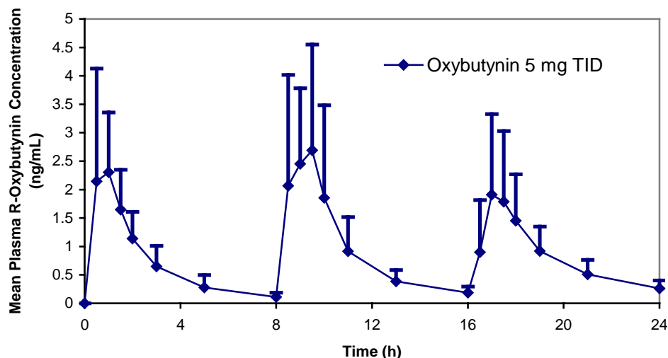
Figure 1. Mean R-oxybutynin plasma concentrations following three doses of DITROPAN ® 5 mg administered every 8 hours for 1 day in 23 healthy adult volunteers
