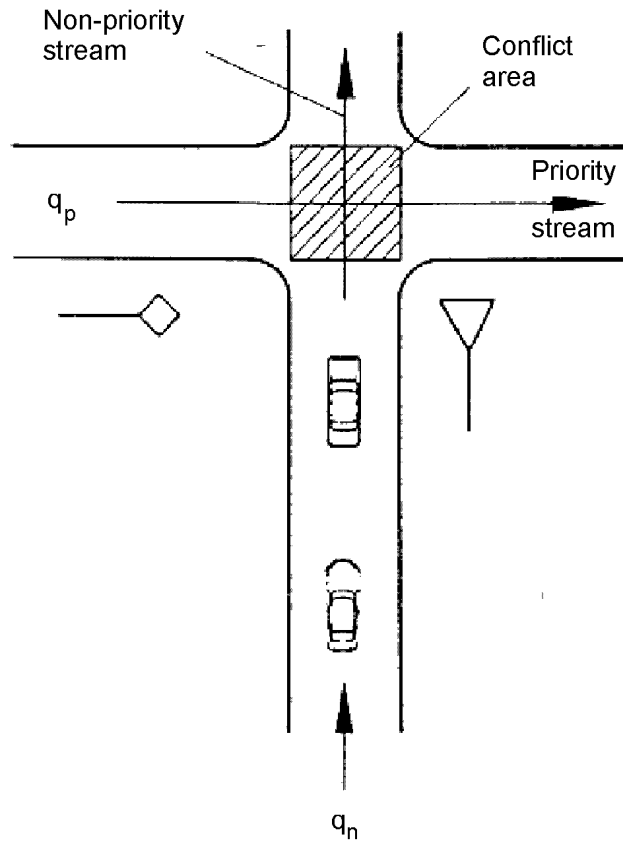
Figure 8.7 Illustration of the Basic Queuing System.
