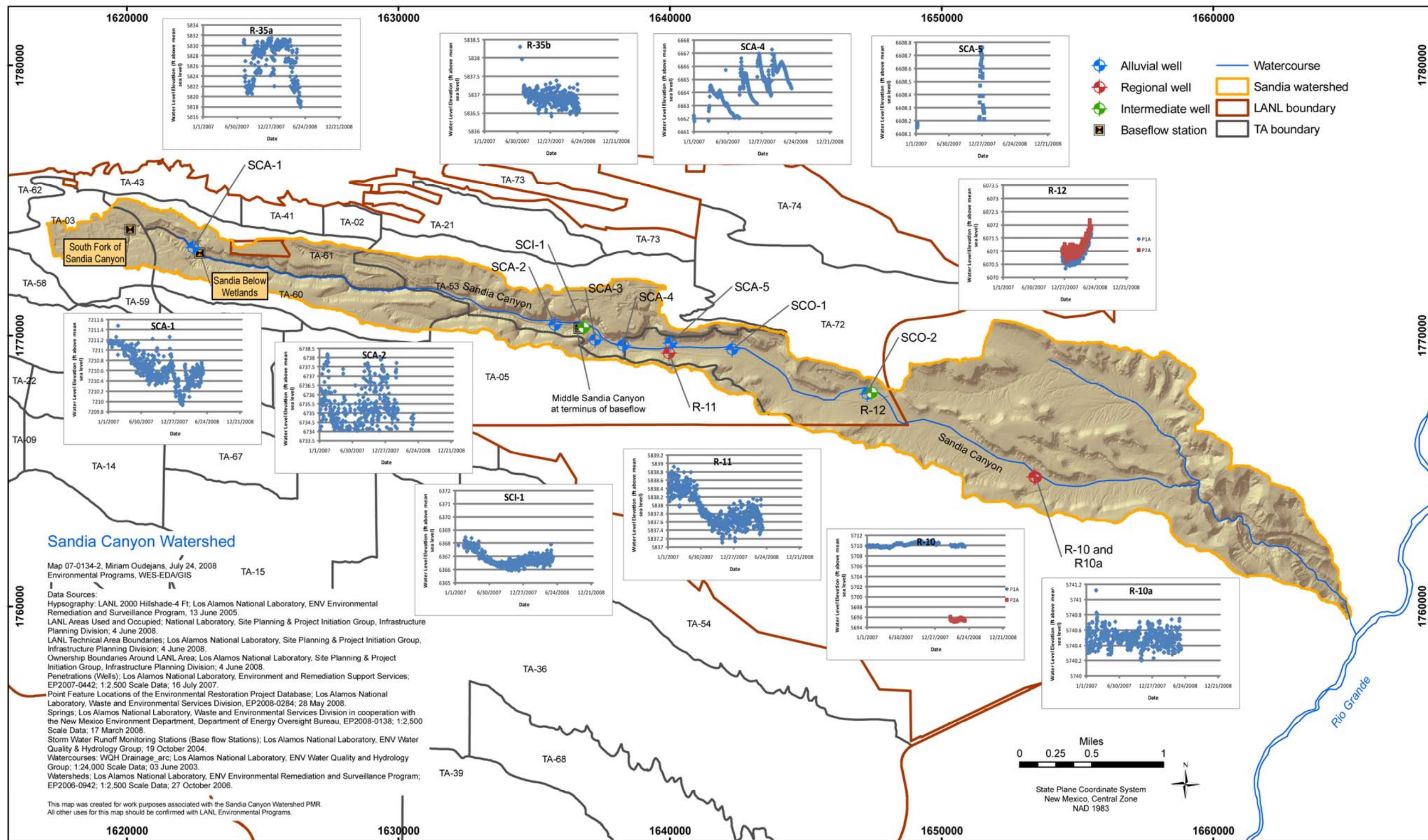
Figure 3.3-1 Groundwater elevations
