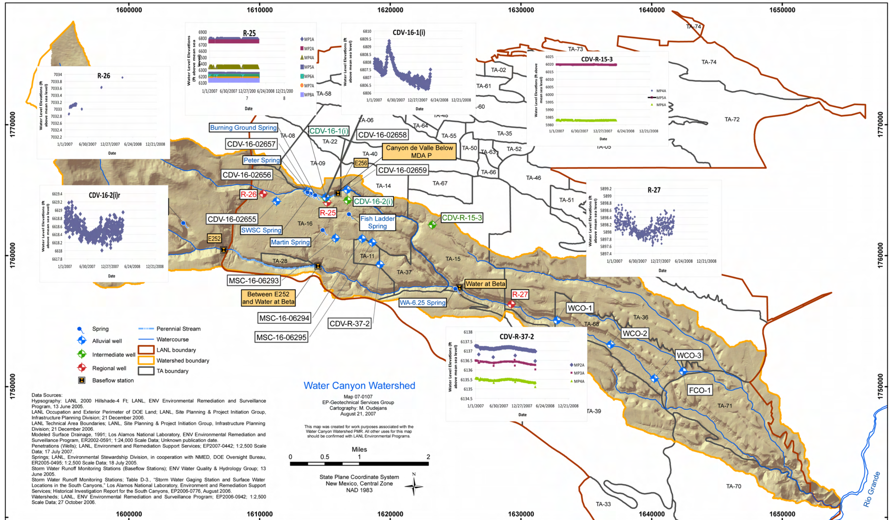
Figure 3.3-2 Intermediate and regional groundwater elevations
