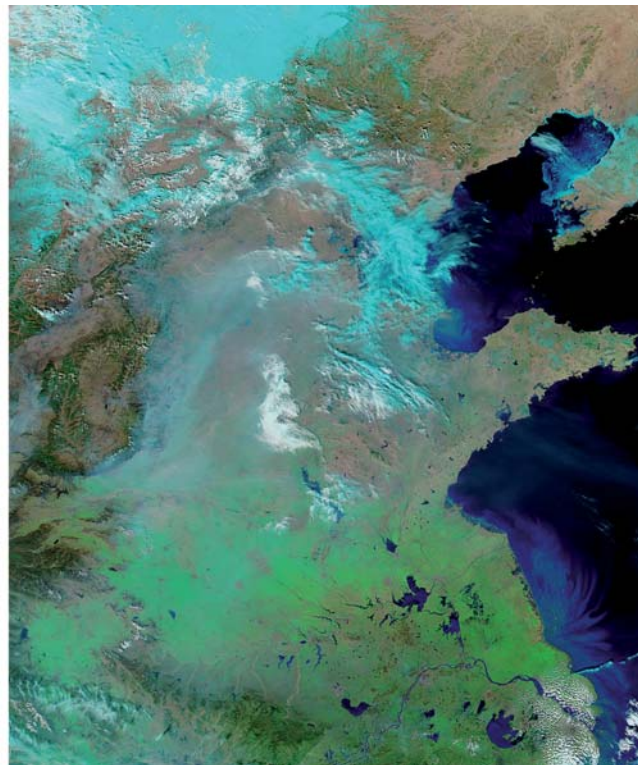
Air pollution does not affect health alone; it can reduce farm productivity by shielding crops from sunlight. The image to the left, similar to a digital photograph, shows a natural-colour view of thick haze over the agricultural regions north of the Yangtze River in eastern China, 28 February 2005. The image to the right uses short-wave and near-infrared observations to reveal the green winter crops, mostly wheat and rice (close to the Yangtze River), underneath the haze. Water is deep blue or brighter blue when sediment levels are high.
