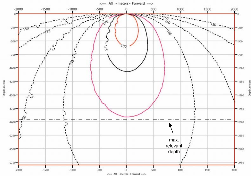
FIGURE 3. Modeled received sound levels (SELs) from the 36-airgun array operating in deep water at a 6-m tow depth, planned for use during the TAIGER survey, 21 March–15 July 2009. Received rms levels (SPLs) are expected to be ~10 dB higher. Maximum relevant depth is applicable to marine mammals.
