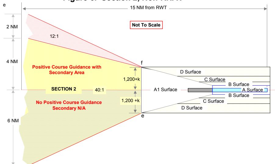
Figure 6. Section 2, Non-RNAV
