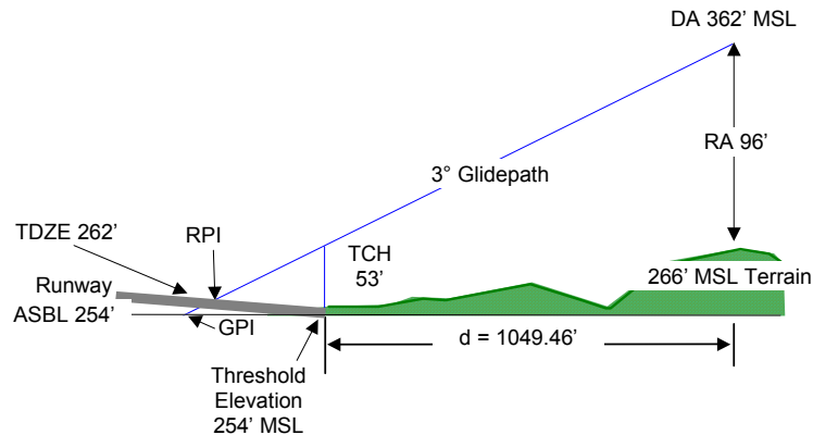
Figure 4. Calculating RA
