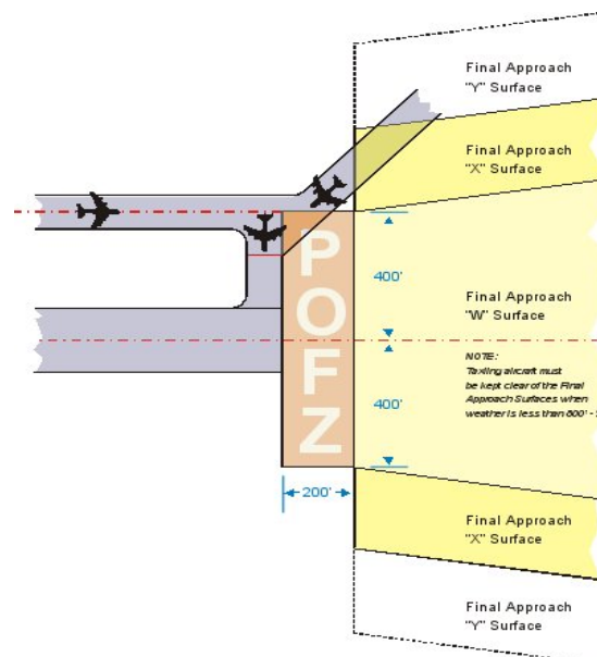
Figure 2. POFZ/Final Segment Obstacle Clearance Surfaces
