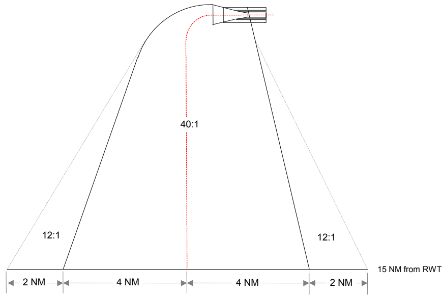
Figure 8. Turning Missed Approach (Section 1 Extended)
