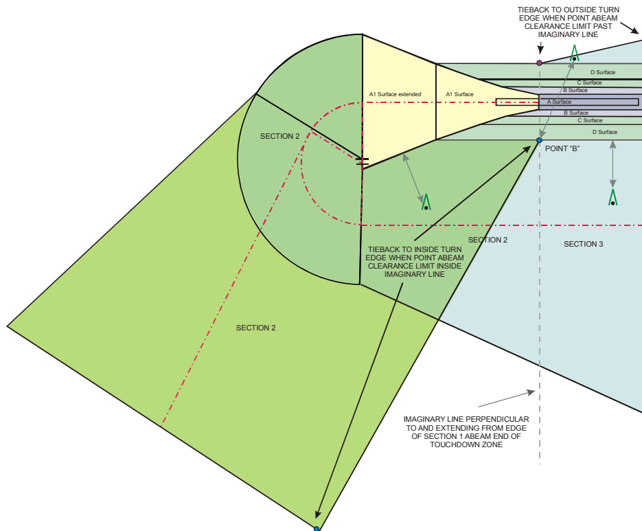
Figure 9. Turning Missed Approach Detail - Continued
