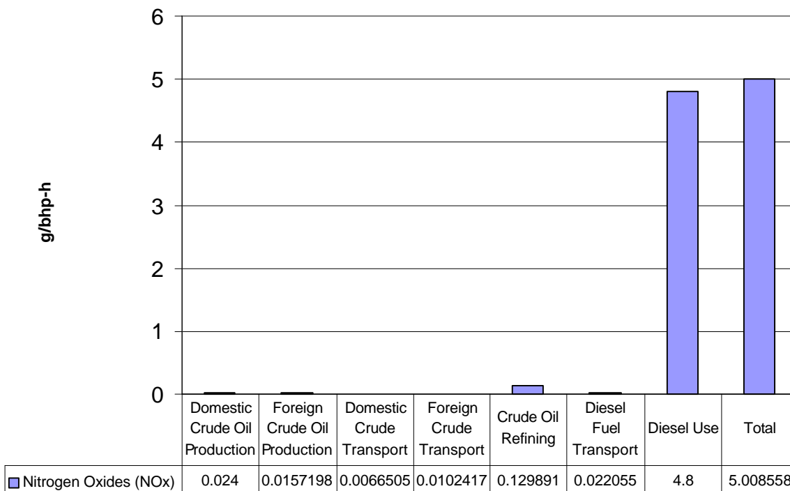
Figure 119: NO x Emissions from Petroleum Diesel Life Cycle (Reported as NO 2 )
