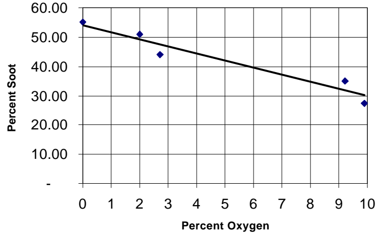
Figure 81: Correlation for Soot Content in PM as a Function of Oxygen Content
