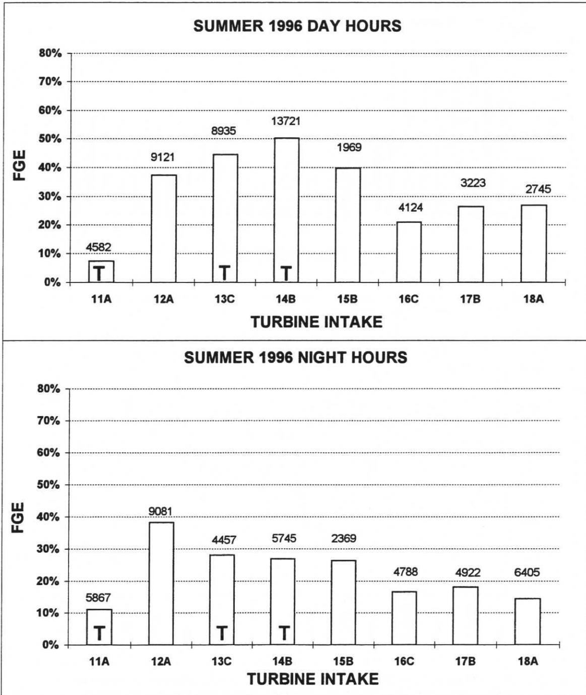
Figure 53. Plots of fish guidance efficiency (FGE) by turbine intake for day and night hours in summer at Powerhouse 2. Bars represent mean FGE based on day or night hours for each intake through the season. Values above the bars indicate total smolt passage for each intake during those hours. A "T" at the base of some of the bars indicates that a turbine intake extension was present.
