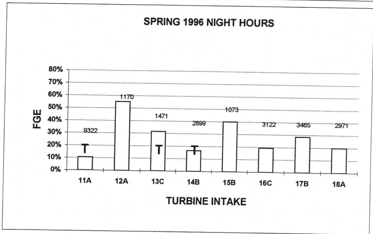
Figure 50. Plots of fish guidance efficiency (FGE) by turbine intake for day and night hours in spring at Powerhouse 2. Bars represent mean FGE based on day or night hours for each intake through the season. Values above the bars indicate total smolt passage for each intake during those hours. A "T" at the base of some of the bars indicates that a turbine intake extension was present.
