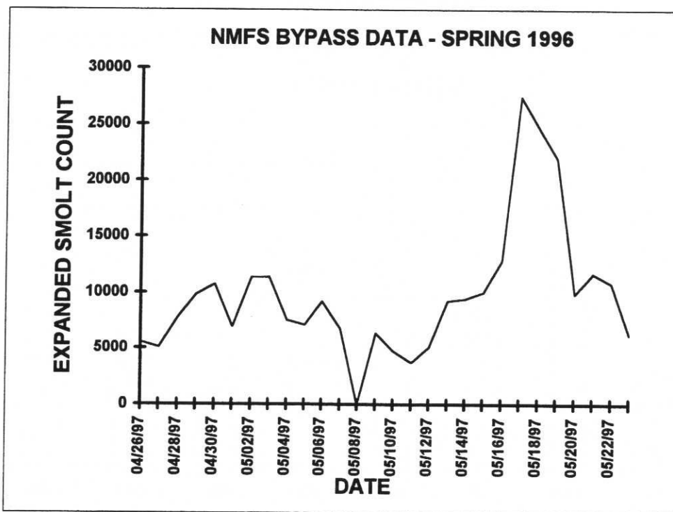
Figure 48. Plot of fish guidance efficiency (FGE) and normalized total passage by treatment day in spring at Powerhouse 2 (upper plot) and National Marine Fisheries Service juvenile bypass data by spring date in 1996 (lower plot). Bars represent mean FGE across the powerhouse for each treatment day. The horizontal line is the grand mean for spring. Total passage values were normalized to a maximum of 1. Mean FGE for the season is shown in the upper left corner. Bypass counts reflect sub-samples expanded to full hours. Dates along the abscissa coincide with spring treatment days.
