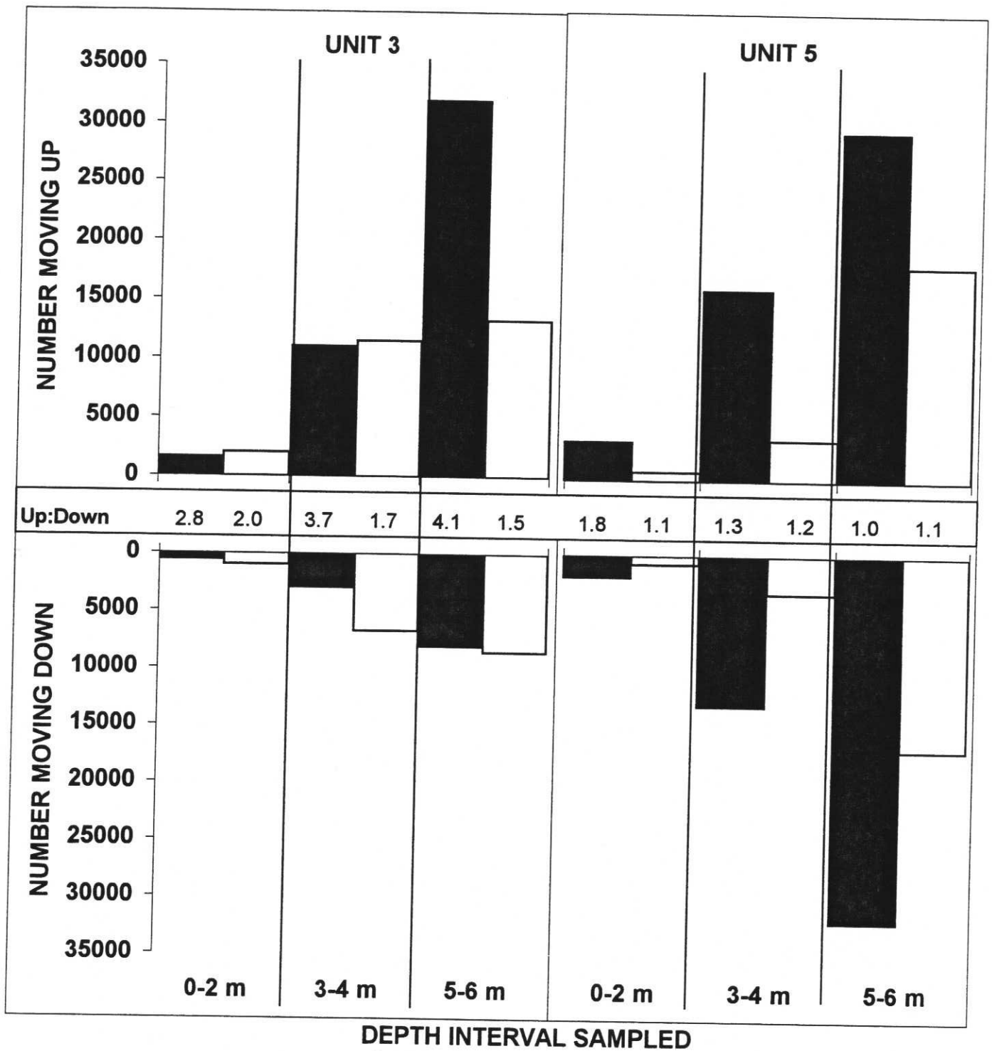
Figure 54. Plots showing the number of smolt-sized fish moving up or down in the water column 3-4 m upstream of trash racks of center intakes of Unit 3 and 5 when the sluice gate was open. Trash rack treatments are indicated by the color of bars (black = blocked; white = unblocked). Positive and negative vectors indicate upward and downward movement, respectively.
