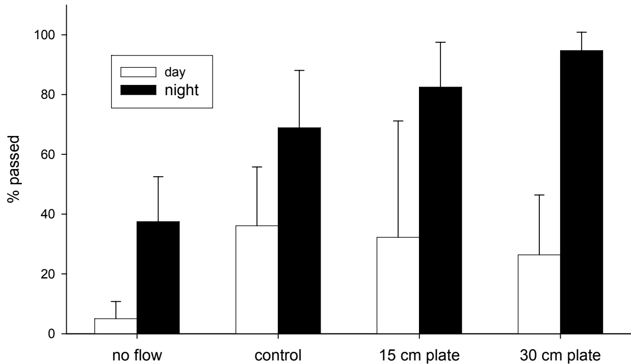
Figure 15. Mean percentage of lamprey to successfully pass through a simulated fishway during one-hour day and night trials with a diffuser grating placed adjacent to and upstream from the second upstream weir (control), with no water flowing through the diffuser, with a 15 cm solid plate attached to the diffuser adjacent to the orifice, and with a 30 cm solid plate attached to the diffuser adjacent to the orifice.
