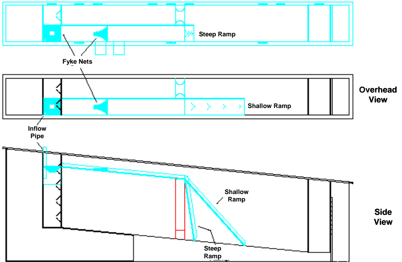
Figure 7. Diagram showing placement and structure of a steep and a shallow bypass ramp.
