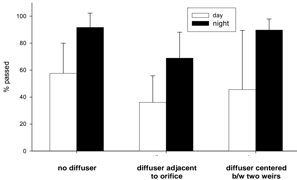
Figure 14. Mean percentage of lamprey that successfully passed through a simulated fishway during one-hour day and night trials with no diffuser grating, with a diffuser placed adjacent to and upstream from the second upstream weir, and with a diffuser centered between the second and third upstream weirs.
