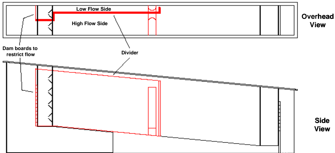
Figure 8. Diagram showing placement of a vertical slot entrance, a divider, and dam boards used to differentially control flow through two portions of the entrance weir.
