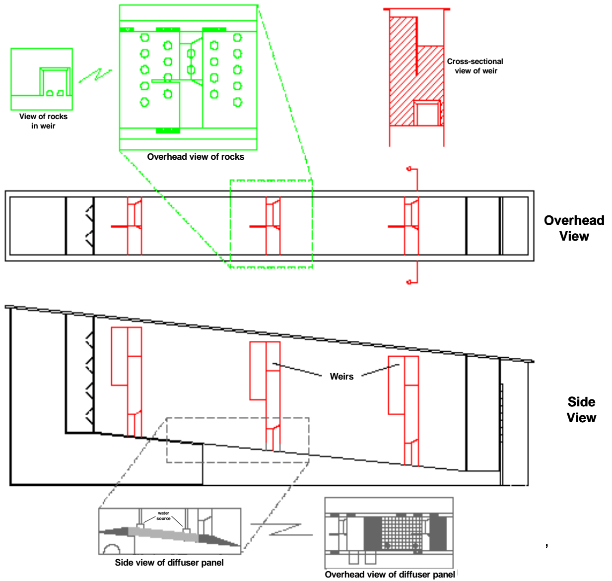
Figure 4. Diagram showing placement and structure of overflow weirs, orifices, a diffuser panel, and velocity refuges.
