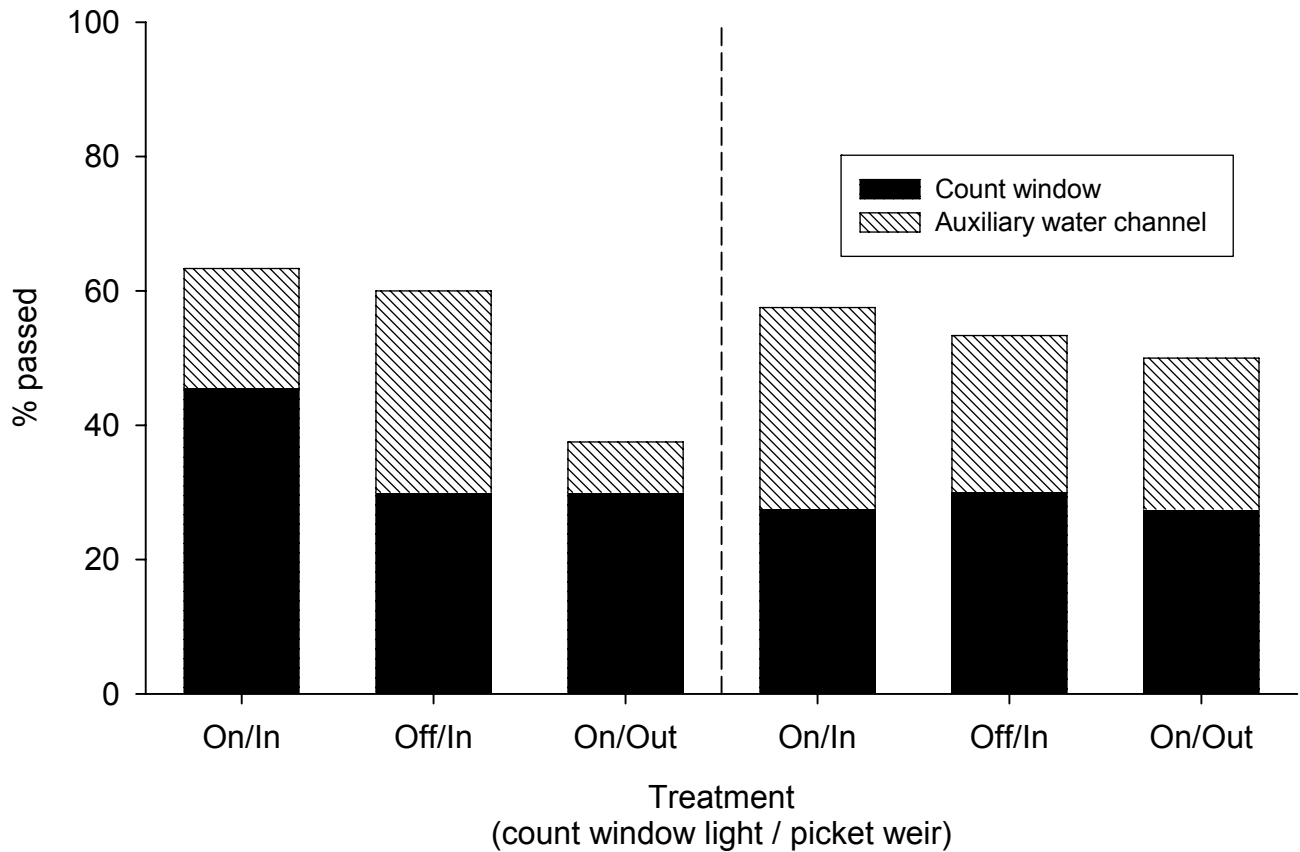
Figure 16. Mean percentage of lamprey that successfully passed through a simulated count window and the proportion of lamprey that passed on each side of divider during one-hour day and night trials with (In) and without (Out) the presence of a picketed lead and with count window lighting on and off.
