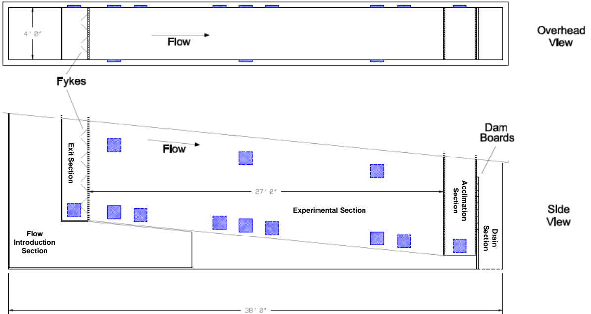
Figure 2. Basic configuration of the experimental fishway set up in the Bonneville Dam Adult Fish Facility (AFF). Squares represent view port locations.
