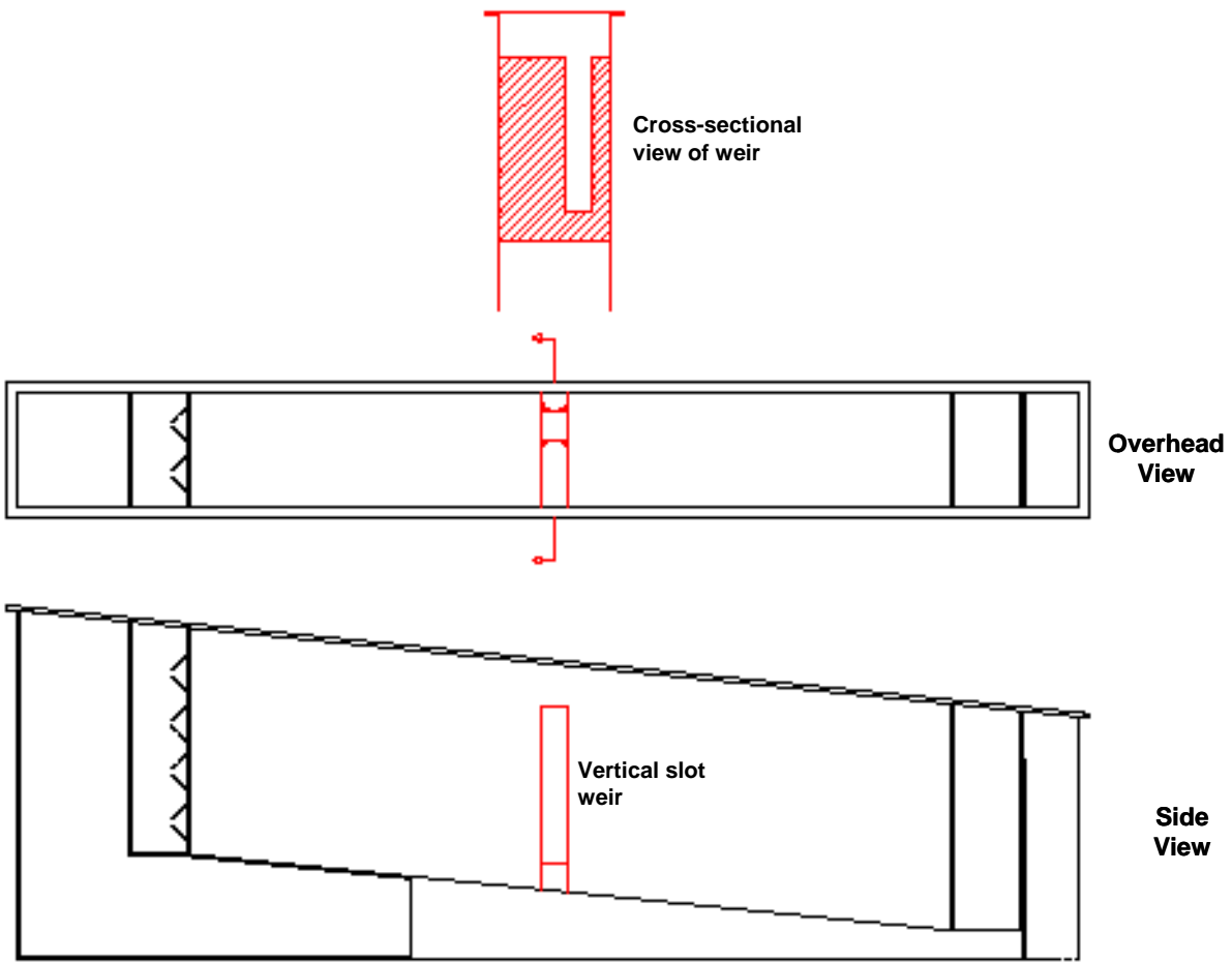
Figure 6. Diagram showing placement of a vertical slot weir with squared or rounded bulkheads.
