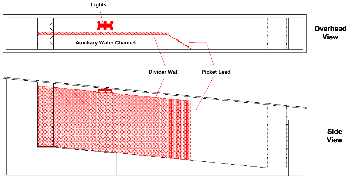
Figure 5. Diagram showing placement of count window lights, a divider, and picket lead weir.
