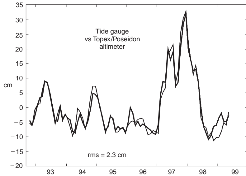
a0340fig0006 Figure 6 Monthly mean sea level deviation near the Galapagos Islands derived from tide gauge data and altimeter data. The ~ 2 cm agreement demonstrates the accuracy of altimetry for observing sea level variability. The effect of the 1997-98 El Niño is apparent.
