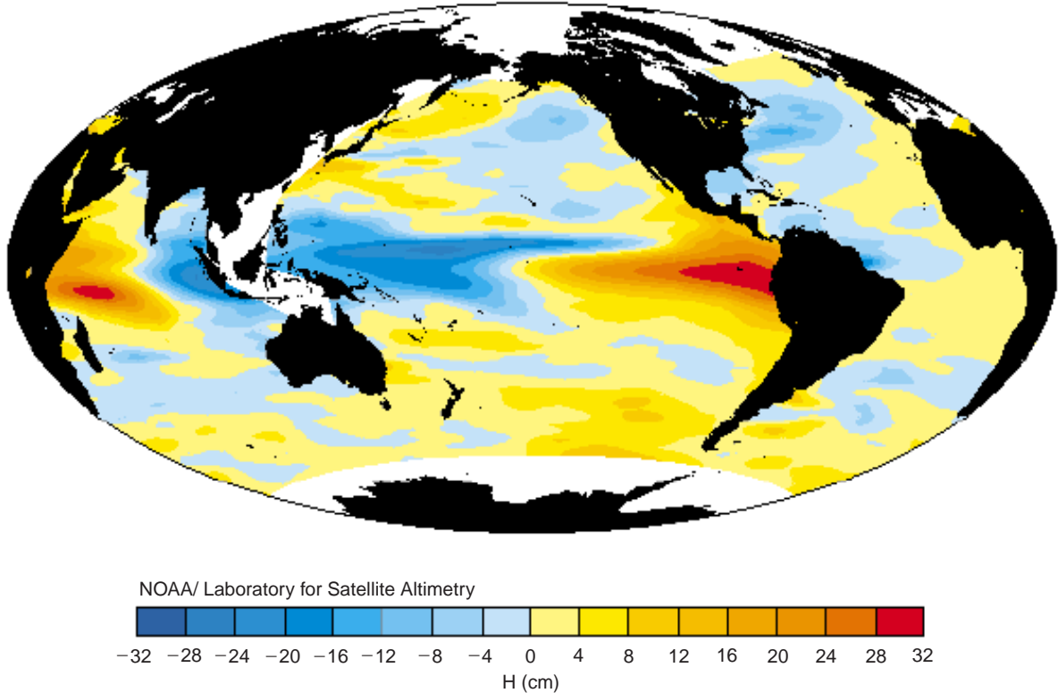
a0340fig0007 Figure 7 Global sea level anomaly observed by the Topex/Poseidon altimeter at the height of the 1997–98 El Niño. High (low) sea level corresponds to areas of positive (negative) heat anomaly in the ocean’s upper layers.
