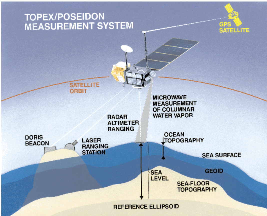
a0340fig0001 Figure 1 Schematic diagram of satellite radar altimeter system. Range to the sea surface together with independent determination of the satellite orbit yields profiles of sea surface topography (sea level) relative to the Earth's reference ellipsoid. Departures of sea level from the geoid drive surface geostrophic currents.
