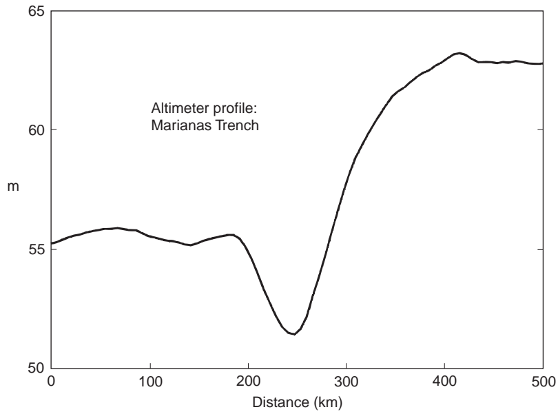
a0340fig0002 Figure 2 Sea surface topography across the Marianas Trench in the western Pacific measured by Topex/Poseidon. Heights are relative to the Earth's reference ellipsoid.
