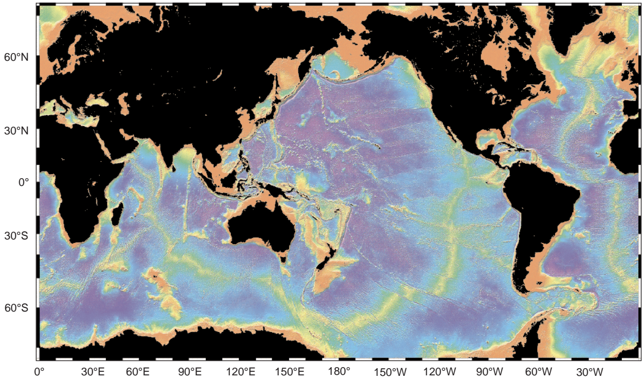
Figure 3 Topography of the ocean bottom determined from a combination of satellite altimetry, gravity anomalies, and bathymetric data collected by ships. (Courtesy of Walter H.F. Smith, NOAA, Silver Spring, Md., USA.)
