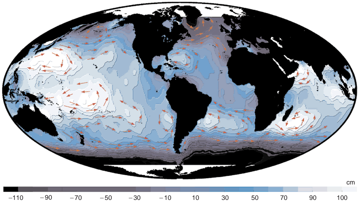
Figure 4 Surface geostrophic circulation determined from a combination of satellite altimetry and a model of the marine gravity field. (Courtesy of Centre National d'Etudes Spatiales, Toulouse, France.).
