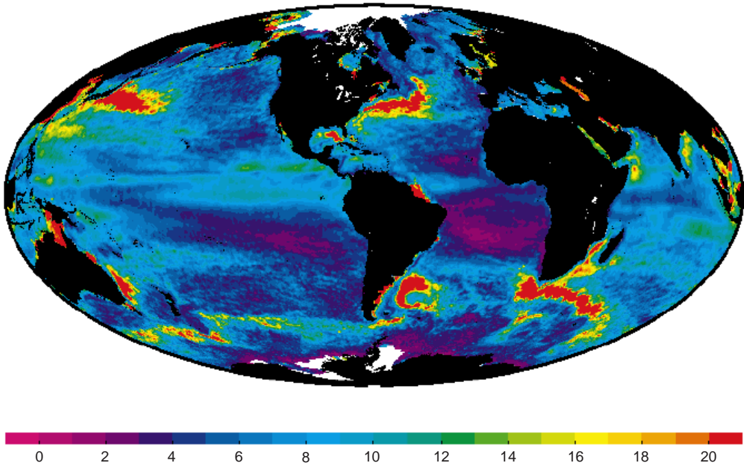
a0340fig0005 Figure 5 Variability of sea surface topography over the period 1992–98 from three satellite altimeters: Topex/Poseidon, ERS-1, and ERS-2. Highest values (cm) correspond to western boundary currents which meander and generate eddies. (Courtesy of Centre National d’Etudes Spatiales, Toulouse, France.).
