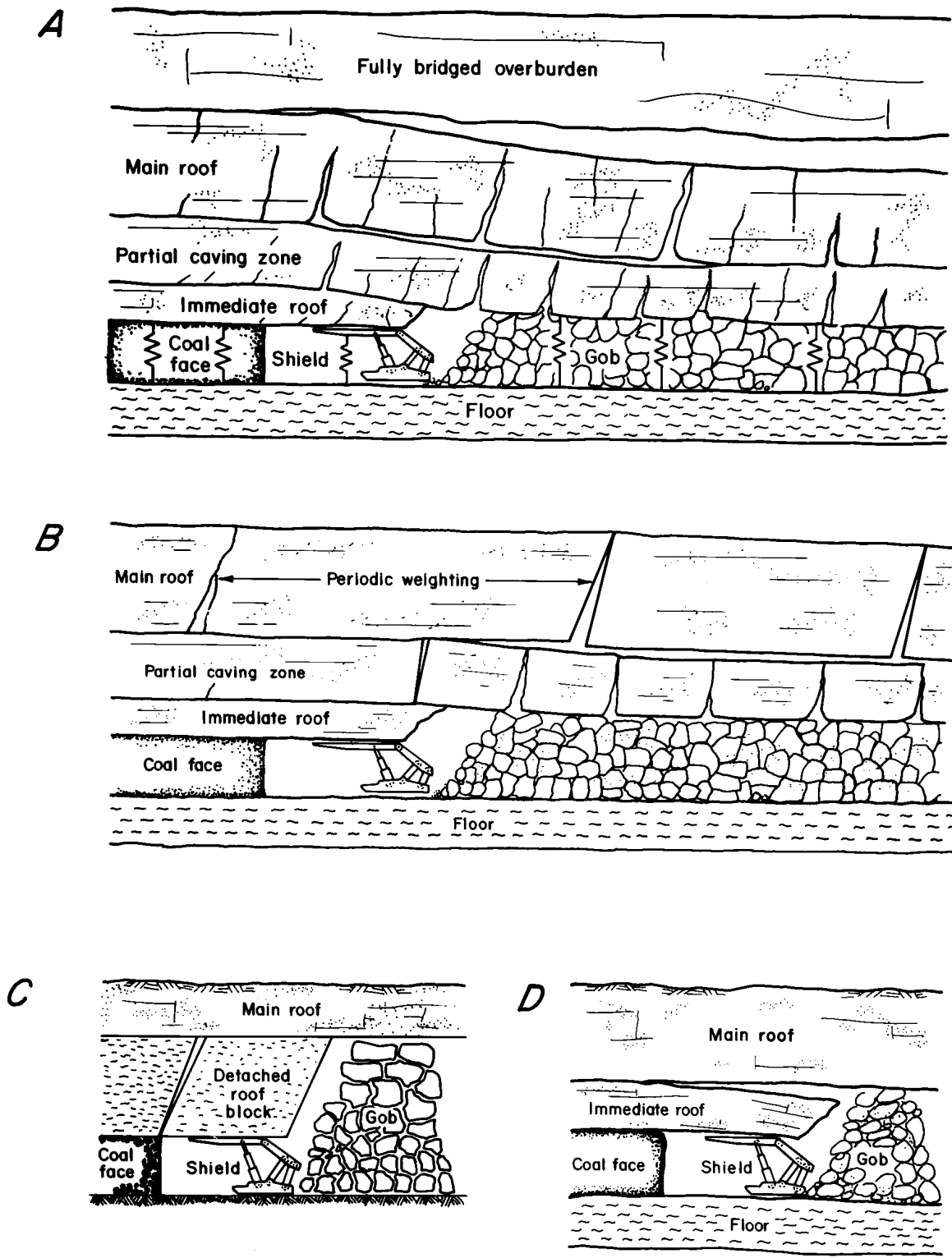
Figure 23.—Four general categories of strata behavior pertaining to shield loading. A, Main roof convergence; B, periodic weighting; C, detached immediate roof; D, deflection of immediate roof.
