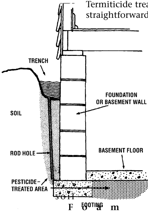
Figure 6. Pesticide treatment for houses with a basement.
