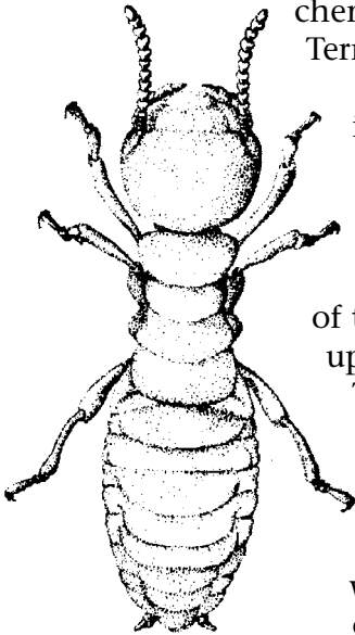
Figure 1. Worker termite.
