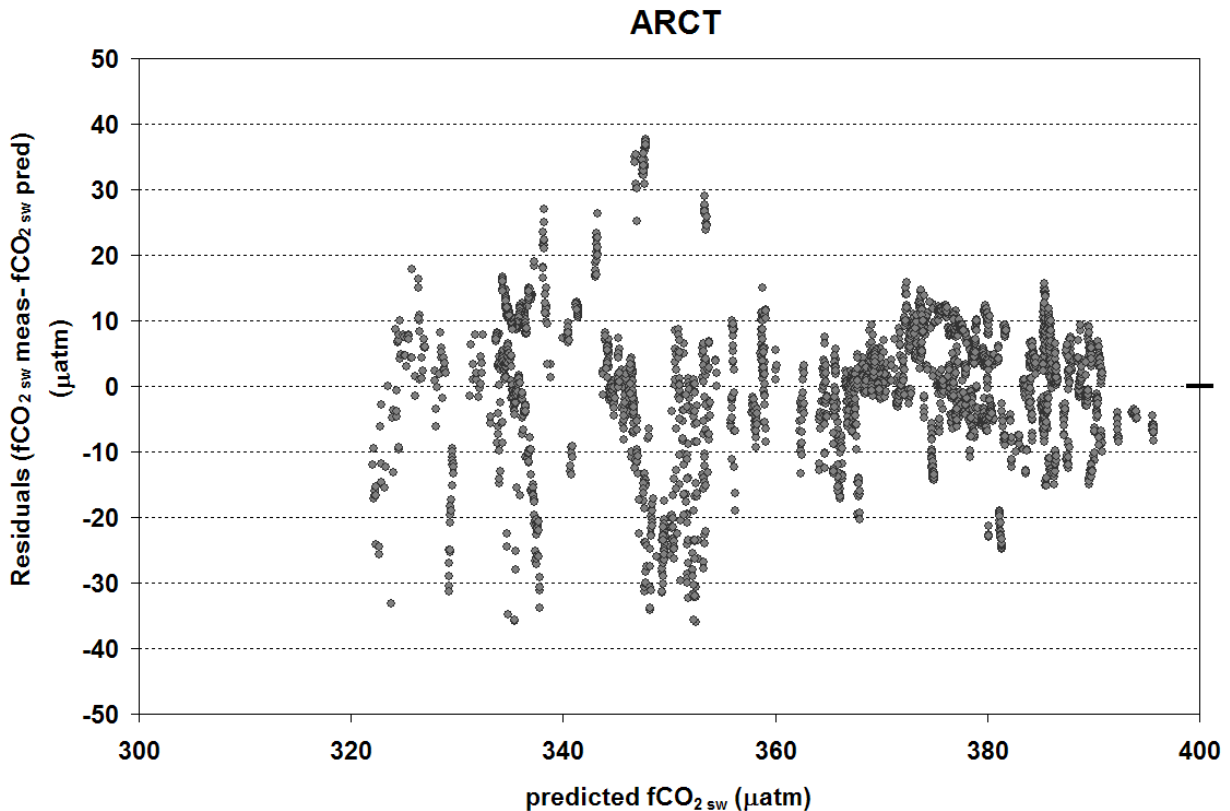
Figure 4: Comparison of the residuals and predicted f\text{CO}_{2,sw} data in the ARCT province. The predicted f\text{CO}_{2,sw} data were retrieved from equation 9 by using mixed layer depth data (source: Argo), SST (source: AVHRR), and position information. Also shown is the mean difference which is 0.00 \mu\text{atm} (black bar on the right).
