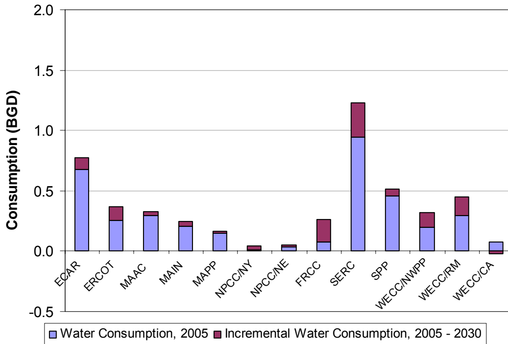
Figure 35 – Average Daily Regional Freshwater Consumption for Thermoelectric Power Generation – Case 4
