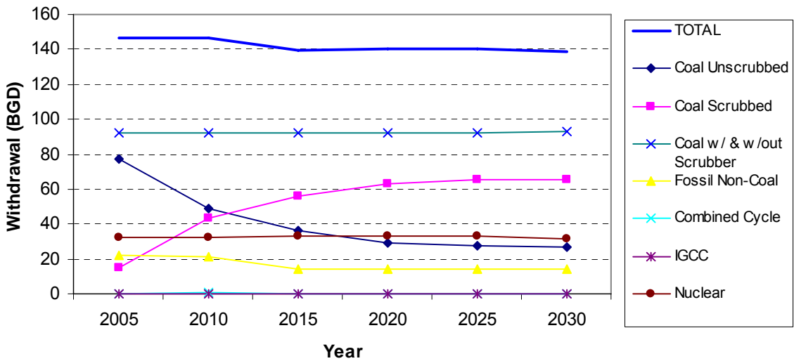
Figure 21 - Average Daily National Freshwater Withdrawal by Fuel for Thermolectric Power Generation – Case 3
