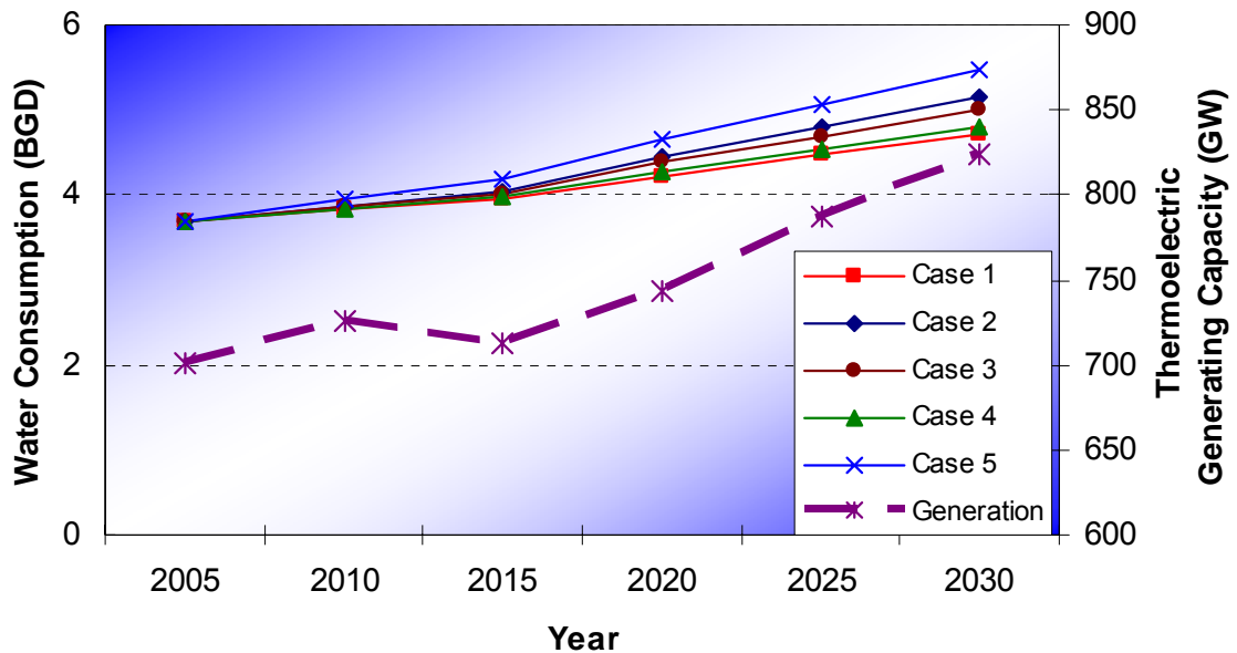
Figure 14 – Average Daily National Freshwater Consumption for Thermoelectric Power Generation
