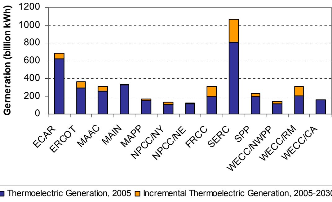
Figure 7 - Thermoelectric Generation, 2005 vs. 2030, by NERC region
