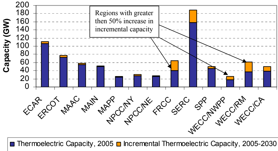
Figure 6 - Thermoelectric Capacity, 2005 vs. 2030, by NERC region
