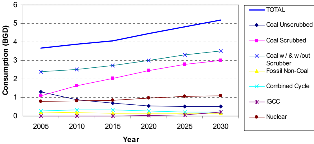
Figure 20 - Average Daily National Freshwater Consumption by Fuel for Thermolectric Power Generation – Case 2
