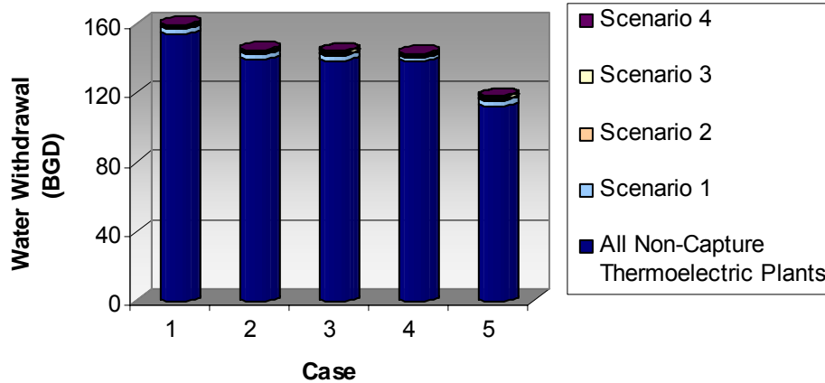
Figure 51 - Thermoelectric Generation with Additional Water Withdrawal for PC and IGCC Carbon Capture Deployment for Year 2030
