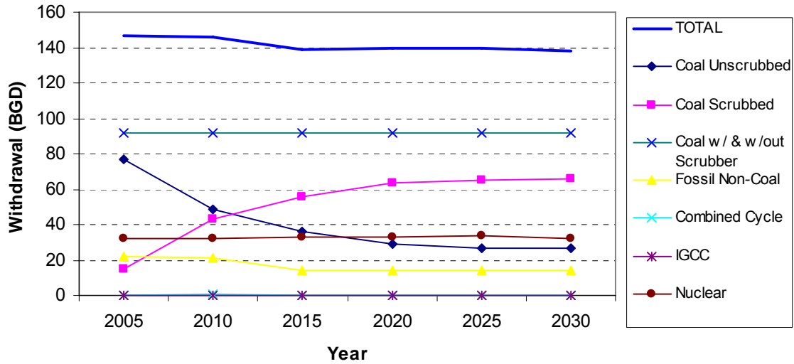
Figure 23 - Average Daily National Freshwater Withdrawal by Fuel for Thermolectric Power Generation – Case 4
