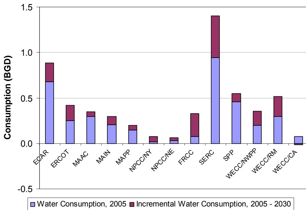
Figure 36 – Average Daily Regional Freshwater Consumption for Thermoelectric Power Generation – Case 5
