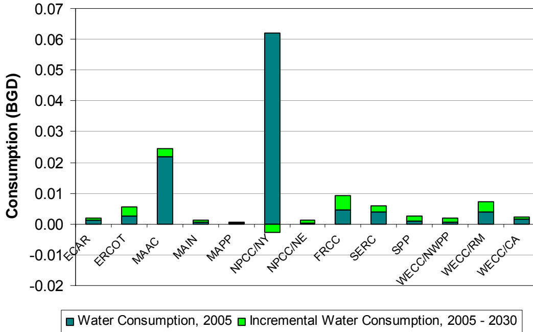
Figure 38 – Average Daily Regional Saline Water Consumption for Thermolectric Power Generation – Case 3
