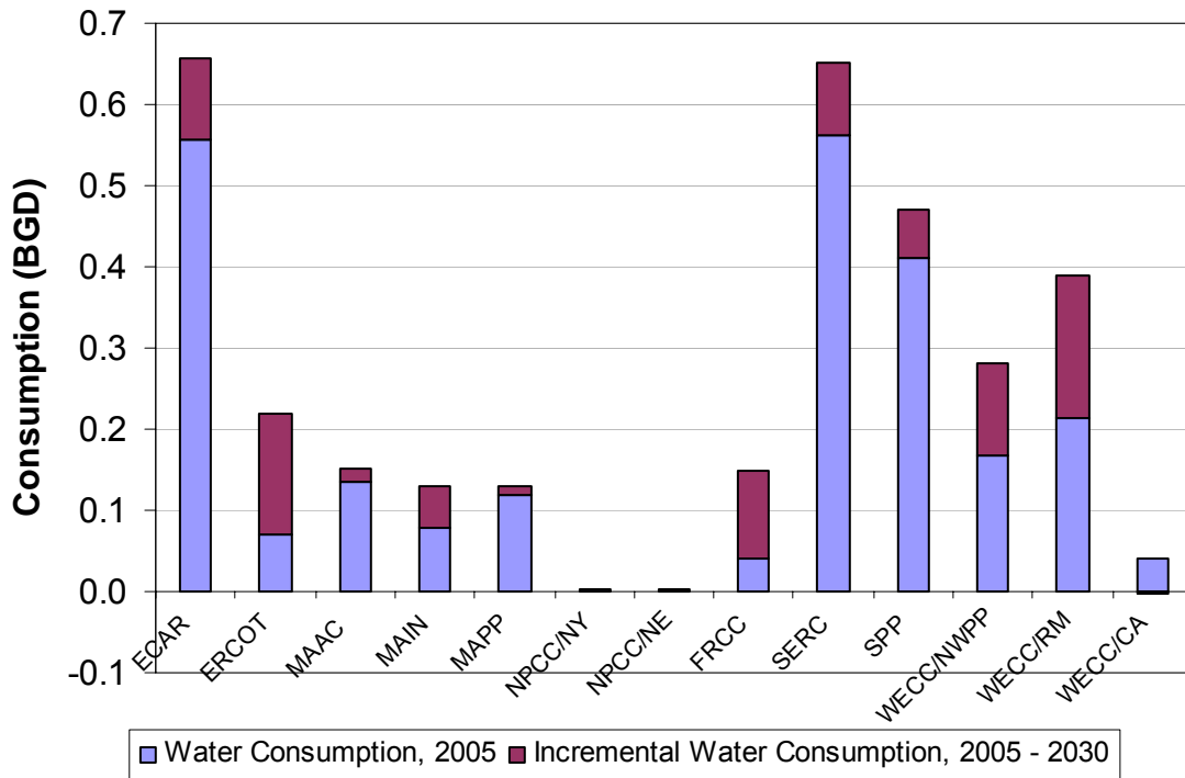
Figure 49 – Average Daily Regional Freshwater Consumption for Coal-Fired Power Generation – Case 4
