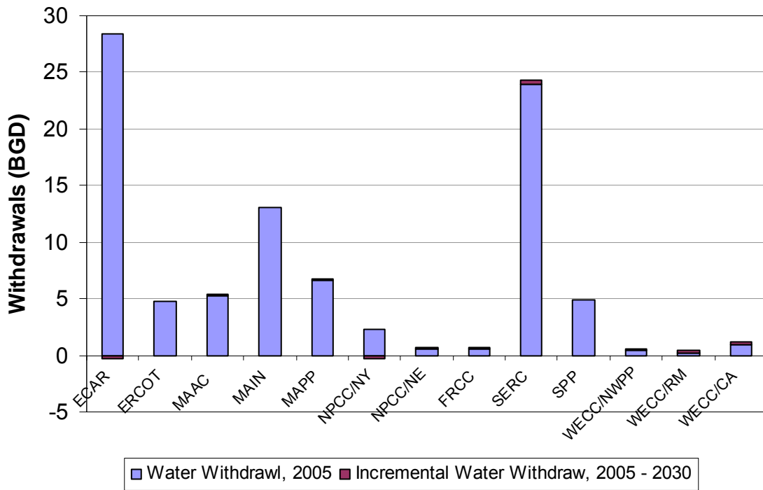
Figure 42 – Average Daily Regional Freshwater Withdrawal for Coal-Fired Power Generation – Case 2
