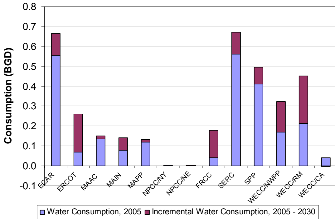
Figure 47 – Average Daily Regional Freshwater Consumption for Coal-Fired Power Generation – Case 2
