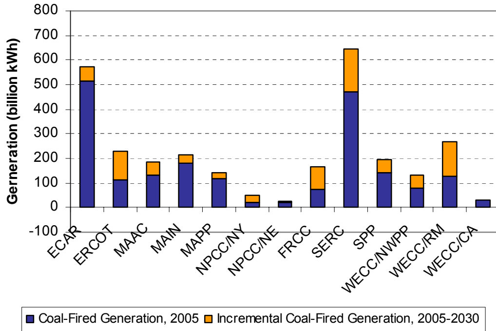
Figure 9 – Coal-Fired Generation, 2005 vs. 2030, by NERC region
