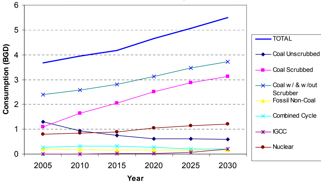
Figure 26 - Average Daily National Freshwater Consumption by Fuel for Thermolectric Power Generation – Case 5
