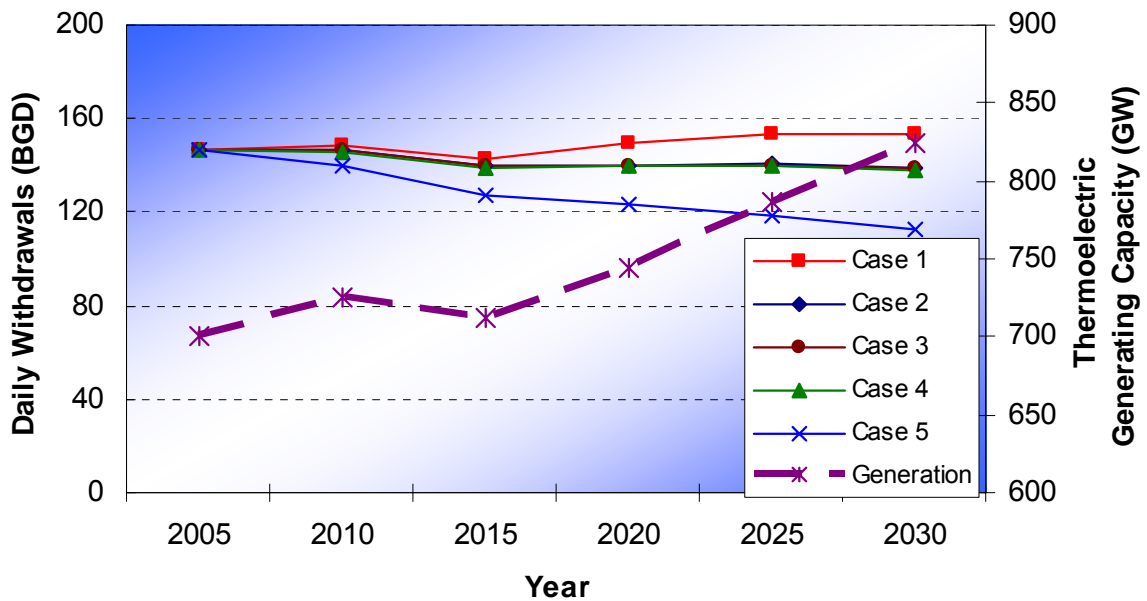
Figure 13 – Average Daily National Freshwater Withdrawal for Thermolectric Power Generation
