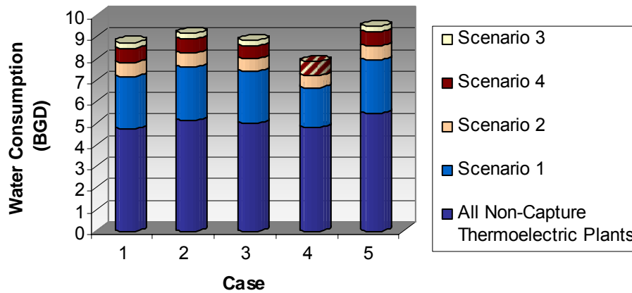
Figure ES-6 - Thermoelectric Generation with Additional Water Consumption for PC and IGCC Carbon Capture Deployment for Year 2030
