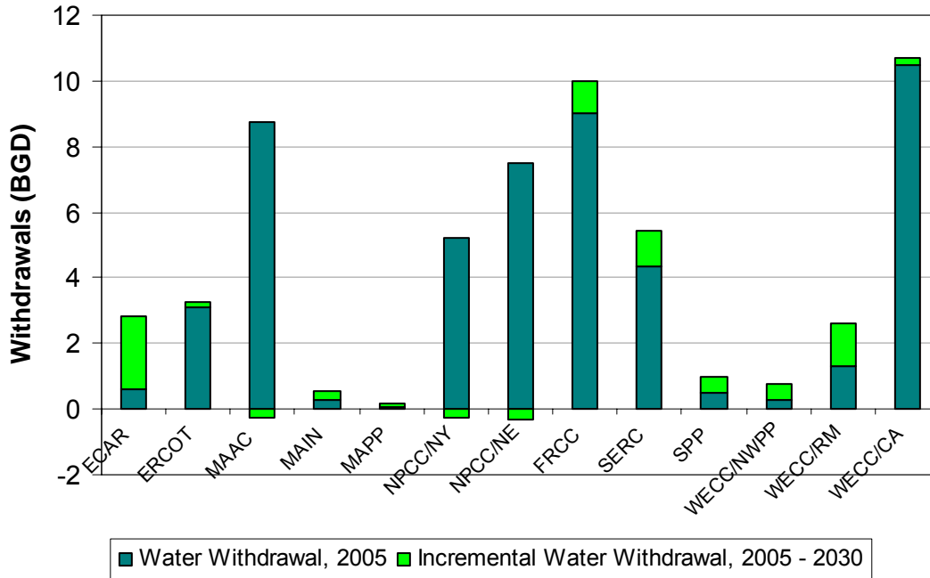
Figure 37 – Average Daily Regional Saline Water Withdrawal for Thermolectric Power Generation – Case 3
