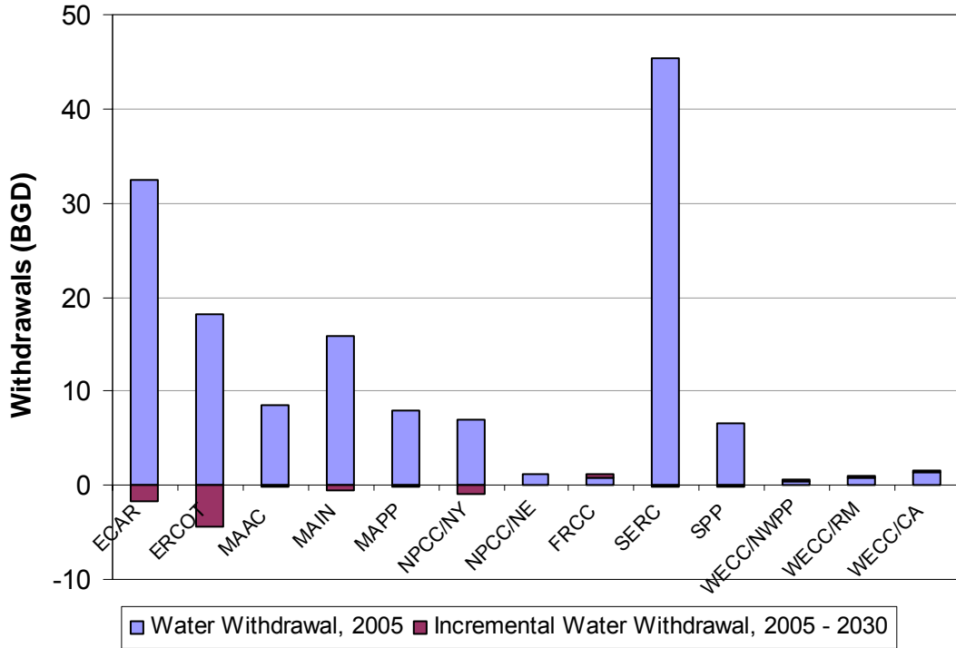
Figure 29 – Average Daily Regional Freshwater Withdrawal for Thermoelectric Power Generation – Case 3
