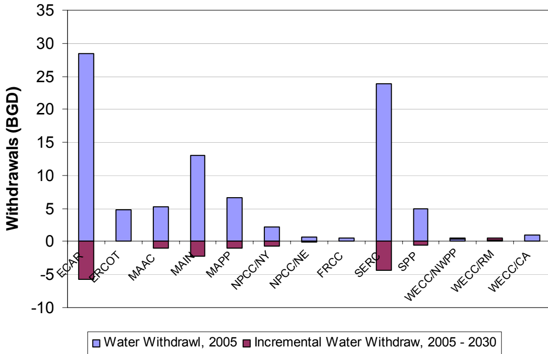
Figure 45 – Average Daily Regional Freshwater Withdrawal for Coal-Fired Power Generation – Case 5
