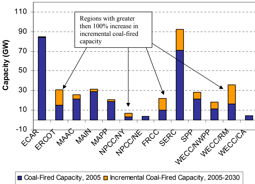
Figure 8 – Coal-Fired Capacity, 2005 vs. 2030, by NERC region
