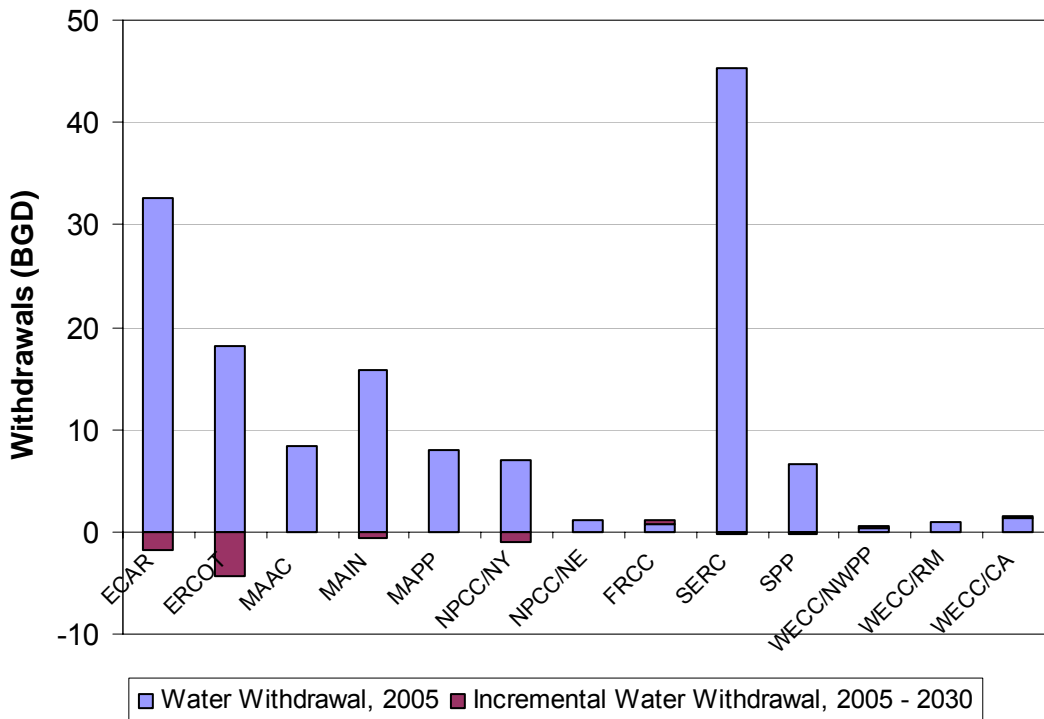
Figure 28 – Average Daily Regional Freshwater Withdrawal for Thermoelectric Power Generation – Case 2
