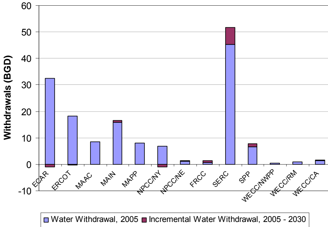
Figure 27 – Average Daily Regional Freshwater Withdrawal for Thermoelectric Power Generation – Case 1
