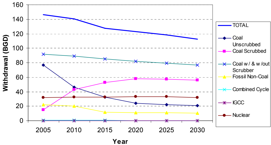
Figure 25 - Average Daily National Freshwater Withdrawal by Fuel for Thermolectric Power Generation – Case 5
