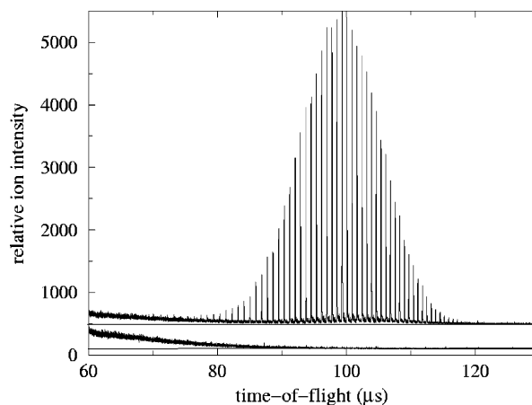
Figure 3. MALDI-TOF mass spectrum of the low-mass, narrow-polydispersity polystyrene (SRM 2888) and its congruent analyte-free spectrum used to demonstrate the method’s capabilities. Spectra are offset for clarity. Expanded views of the analyte spectrum are shown in Figures 8 and 9.
