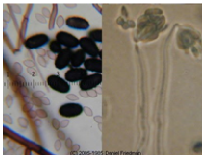
Figure 2: Mold Spores (Left) and Plant Bodies - Hyphae (Right)
