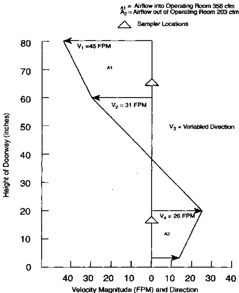
Velocity Distribution through Operating Room Doorway (Room Not in Use)
